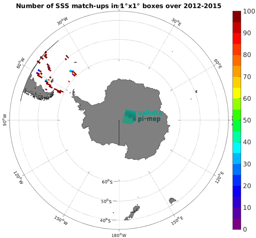
Figure 5: Number of SSS match-ups between TSG (CSIC-UTM) SSS and the Aquarius SSS L2 OR v5 (NASA-GSFC) SSS product for the Roaring Forties and Furious Fifties Pi-MEP region over 1^\circ \times 1^\circ boxes and for the full satellite product period.
