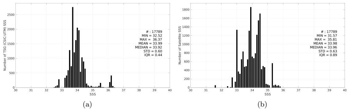
Figure 3: Histograms of SSS from TSG (CSIC-UTM) (a) and Aquarius SSS L2 OR v5 (NASA-GSFC) (b) considering all match-up pairs per bins of 0.1 over the Roaring Forties and Furious Fifties Pi-MEP region and for the full satellite product period.
