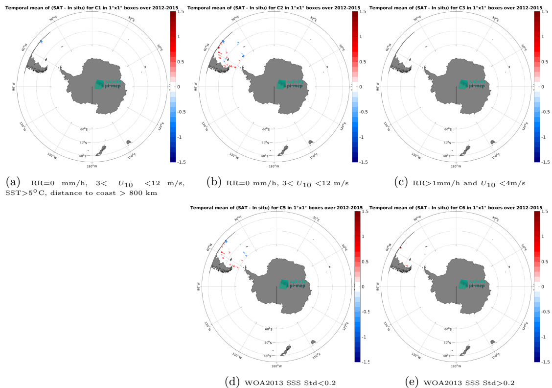
Figure 14: Temporal mean gridded over spatial boxes of size 1^\circ \times 1^\circ of \Delta SSS (Aquarius SSS L2 OR v5 (NASA-GSFC) - TSG (CSIC-UTM)) for 5 different subdatasets corresponding to: RR=0 mm/h, 3 < U_{10} < 12 m/s, SST > 5^\circ\text{C} , distance to coast > 800 km (a), RR=0 mm/h, 3 < U_{10} < 12 m/s (b), RR > 1 mm/h and U_{10} < 4 m/s (c), WOA2013 SSS Std < 0.2 (d), WOA2013 SSS Std > 0.2 (e).
