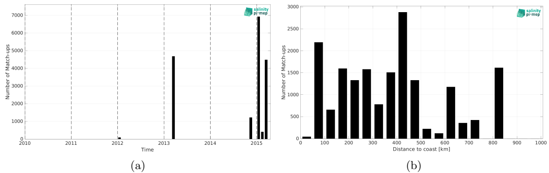
Figure 2: Number of match-ups between TSG (CSIC-UTM) and Aquarius SSS L2 OR v5 (NASA-GSFC) SSS as a function of time (a) and as function of the distance to coast (b) over the Roaring Forties and Furious Fifties Pi-MEP region and for the full satellite product period.
