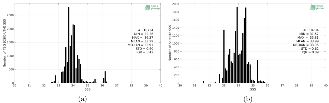
Figure 2: Histograms of SSS from TSG (CSIC-UTM) (a) and Aquarius SSS L2 OR v5 (NASA-GSFC) (b) considering all match-up pairs per bins of 0.1 over the Roaring Forties and Furious Fifties Pi-MEP region and for the full satellite product period.
