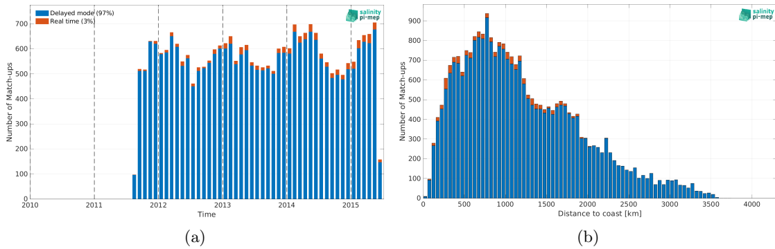
Figure 2: Number of match-ups between Argo and Aquarius SSS L2 OR v5 (NASA-GSFC) SSS as a function of time (a) and as function of the distance to coast (b) over the Roaring Forties and Furious Fifties Pi-MEP region and for the full satellite product period.
