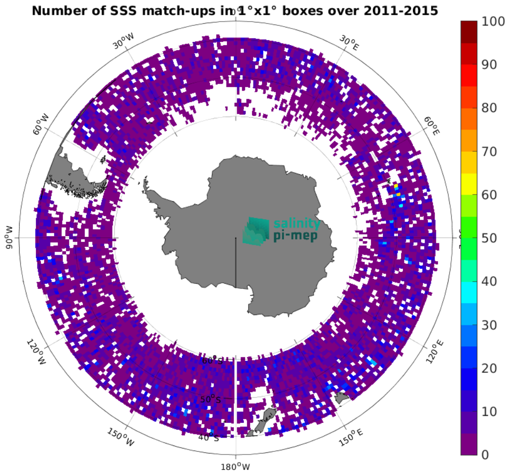
Figure 5: Number of SSS match-ups between Argo SSS and the Aquarius SSS L2 OR v5 (NASA-GSFC) SSS product for the Roaring Forties and Furious Fifties Pi-MEP region over 1^\circ \times 1^\circ boxes and for the full satellite product period.
