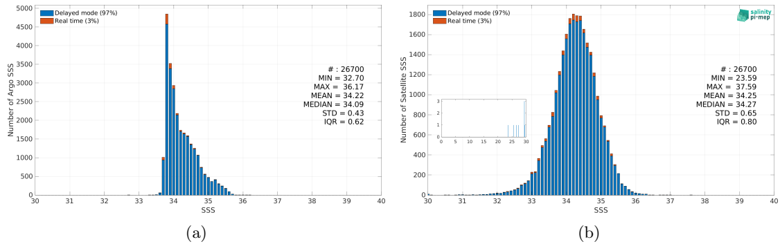
Figure 3: Histograms of SSS from Argo (a) and Aquarius SSS L2 OR v5 (NASA-GSFC) (b) considering all match-up pairs per bins of 0.1 over the Roaring Forties and Furious Fifties Pi-MEP region and for the full satellite product period.
