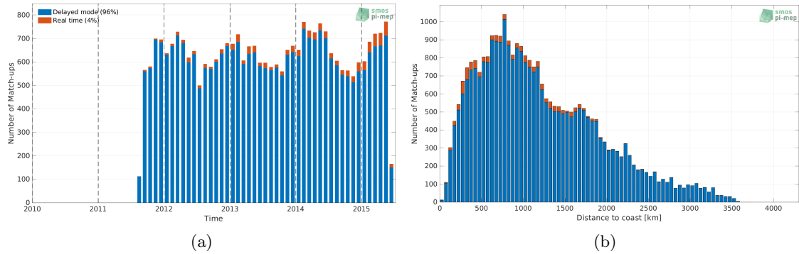
Figure 1: Number of match-ups between Argo and Aquarius SSS L2 OR v5 (NASA-GSFC) SSS as a function of time (a) and as function of the distance to coast (b) over the Roaring Forties and Furious Fifties Pi-MEP region and for the full satellite product period.
