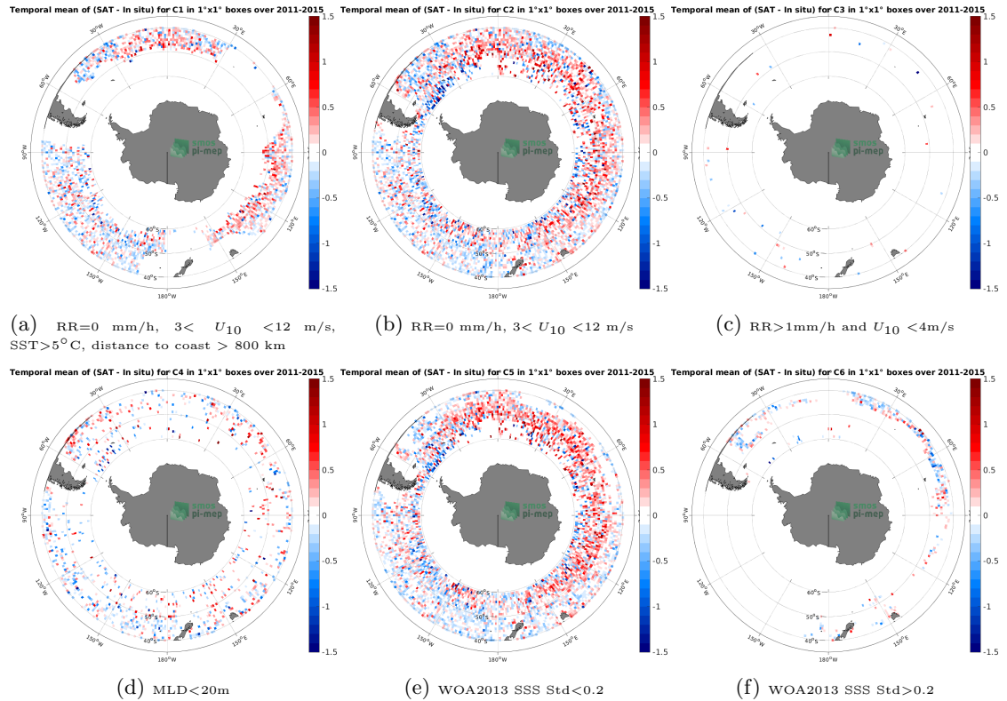
Figure 12: Temporal mean gridded over spatial boxes of size 1^{\circ}\times 1^{\circ} of \Delta\text{SSS} (Aquarius SSS L2 OR v5 (NASA-GSFC) - Argo) for 6 different subdatasets corresponding to:RR=0 mm/h, 3 < U_{10} < 12 m/s, SST >5^{\circ}\text{C} , distance to coast > 800 km (a), RR=0 mm/h, 3 < U_{10} < 12 m/s (b), RR >1 mm/h and U_{10} < 4 m/s (c),MLD <20 m (d),WOA2013 SSS Std <0.2 (e),WOA2013 SSS Std >0.2 (f).
