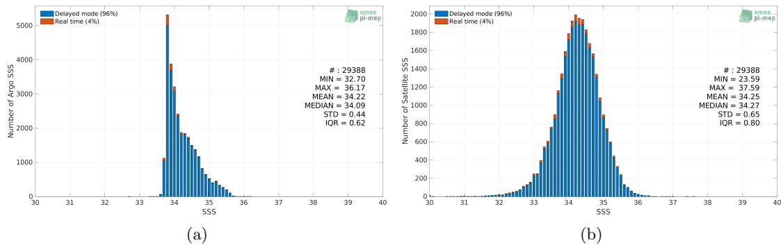
Figure 2: Histograms of SSS from Argo (a) and Aquarius SSS L2 OR v5 (NASA-GSFC) (b) considering all match-up pairs per bins of 0.1 over the Roaring Forties and Furious Fifties Pi-MEP region and for the full satellite product period.
