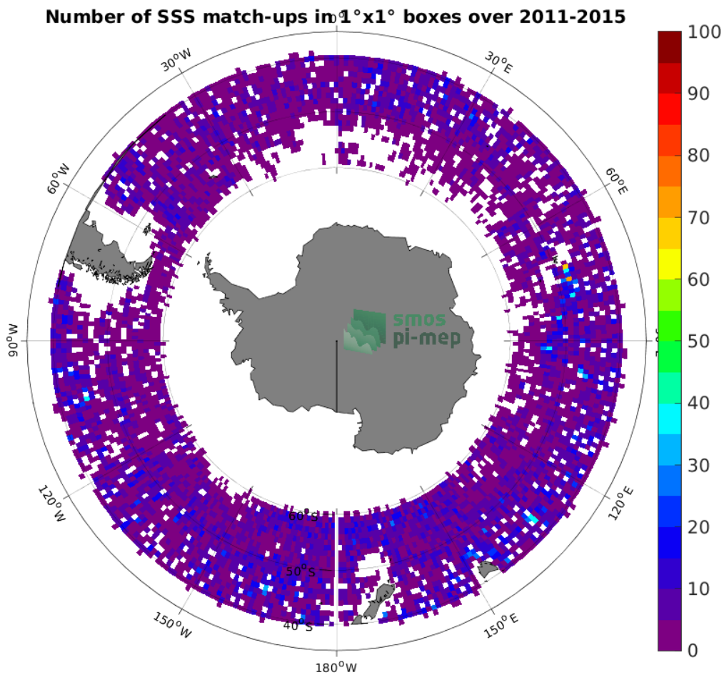
Figure 4: Number of SSS match-ups between Argo SSS and the Aquarius SSS L2 OR v5 (NASA-GSFC) SSS product for the Roaring Forties and Furious Fifties Pi-MEP region over 1^\circ \times 1^\circ boxes and for the full satellite product period.
