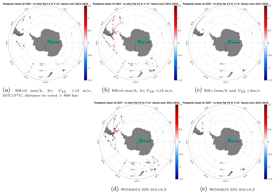
Figure 14: Temporal mean gridded over spatial boxes of size 1^\circ \times 1^\circ of \Delta SSS (Aquarius SSS L2 CAP v5 (JPL) - TSG (SAMOS)) for 5 different subdatasets corresponding to:RR=0 mm/h, 3 < U_{10} < 12 m/s, SST>5°C, distance to coast > 800 km (a), RR=0 mm/h, 3 < U_{10} < 12 m/s (b), RR>1mm/h and U_{10} < 4 m/s (c), WOA2013 SSS Std<0.2 (d), WOA2013 SSS Std>0.2 (e).
