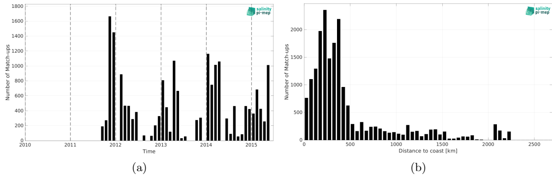
Figure 2: Number of match-ups between TSG (SAMOS) and Aquarius SSS L2 CAP v5 (JPL) SSS as a function of time (a) and as function of the distance to coast (b) over the Roaring Forties and Furious Fifties Pi-MEP region and for the full satellite product period.
