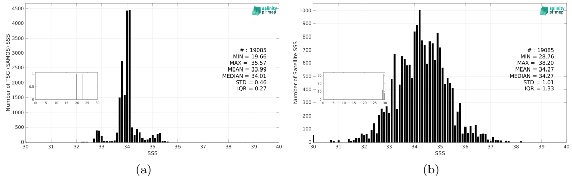
Figure 3: Histograms of SSS from TSG (SAMOS) (a) and Aquarius SSS L2 CAP v5 (JPL) (b) considering all match-up pairs per bins of 0.1 over the Roaring Forties and Furious Fifties Pi-MEP region and for the full satellite product period.
