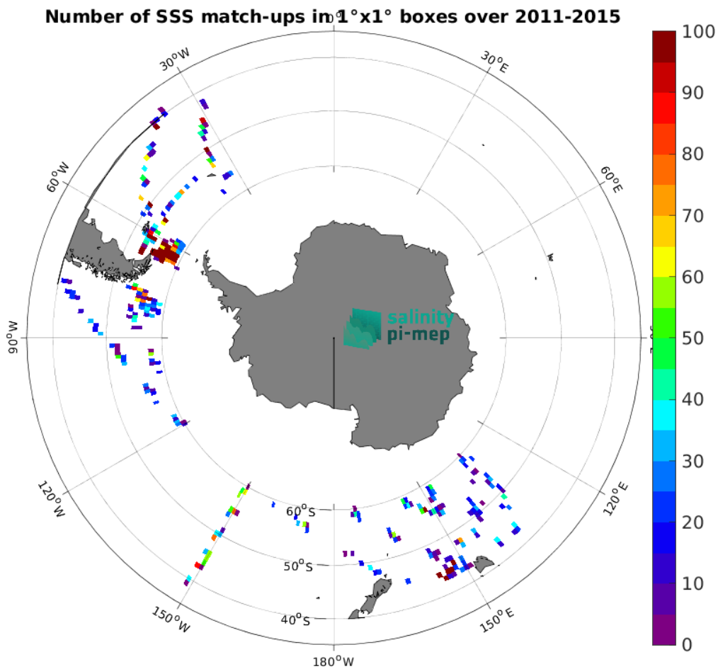
Figure 5: Number of SSS match-ups between TSG (SAMOS) SSS and the Aquarius SSS L2 CAP v5 (JPL) SSS product for the Roaring Forties and Furious Fifties Pi-MEP region over 1^\circ \times 1^\circ boxes and for the full satellite product period.
