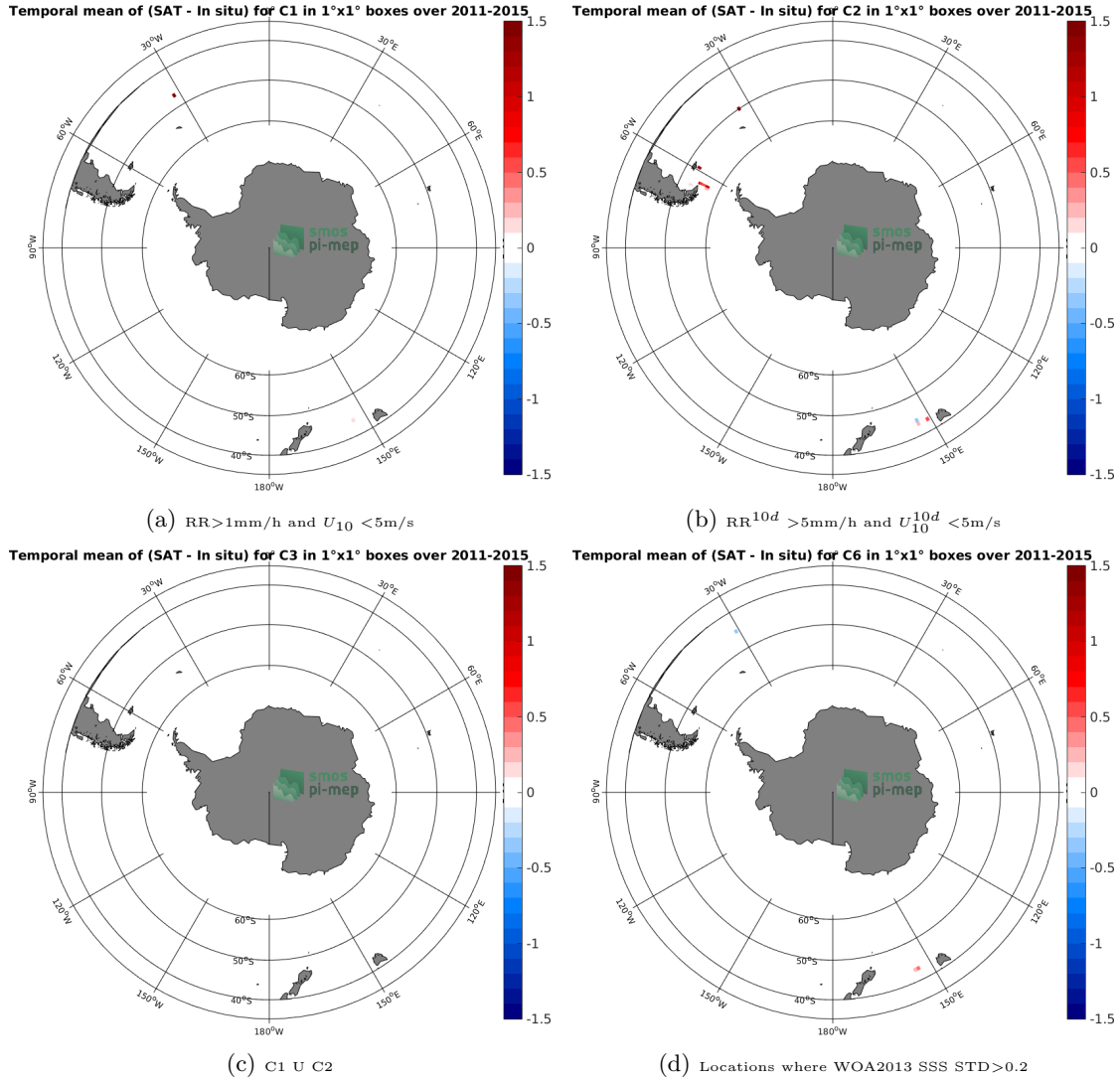
Figure 12: Temporal mean gridded over spatial boxes of size 1^\circ \times 1^\circ of \Delta SSS (Aquarius-L2-JPL-V5 - TSG-SAMOS) for 4 different subdatasets corresponding to: RR > 1\text{mm/h} and U_{10} < 5\text{m/s} (a), RR^{10d} > 5\text{mm/h} and U_{10}^{10d} < 5\text{m/s} (b), C1 U C2 (c), Locations where WOA2013 SSS STD > 0.2 (d).
