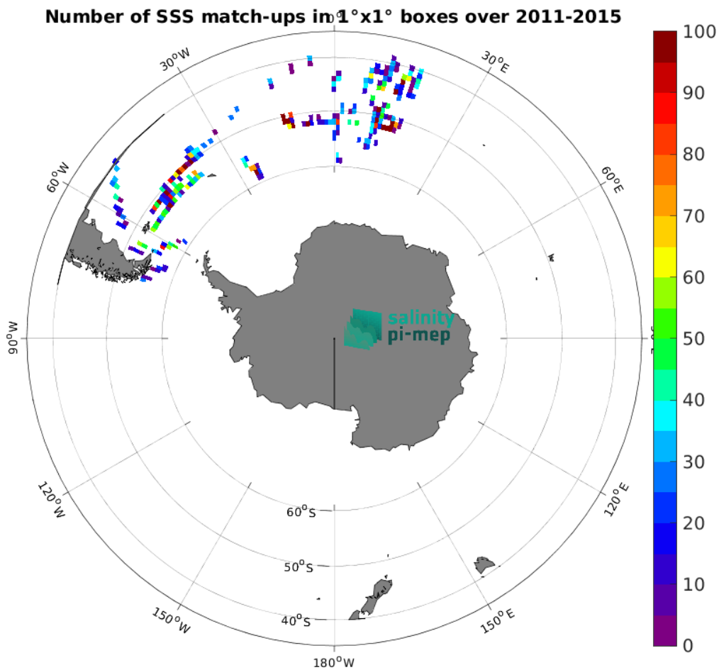
Figure 5: Number of SSS match-ups between TSG (Polarstern) SSS and the Aquarius SSS L2 CAP v5 (JPL) SSS product for the Roaring Forties and Furious Fifties Pi-MEP region over 1^\circ \times 1^\circ boxes and for the full satellite product period.
