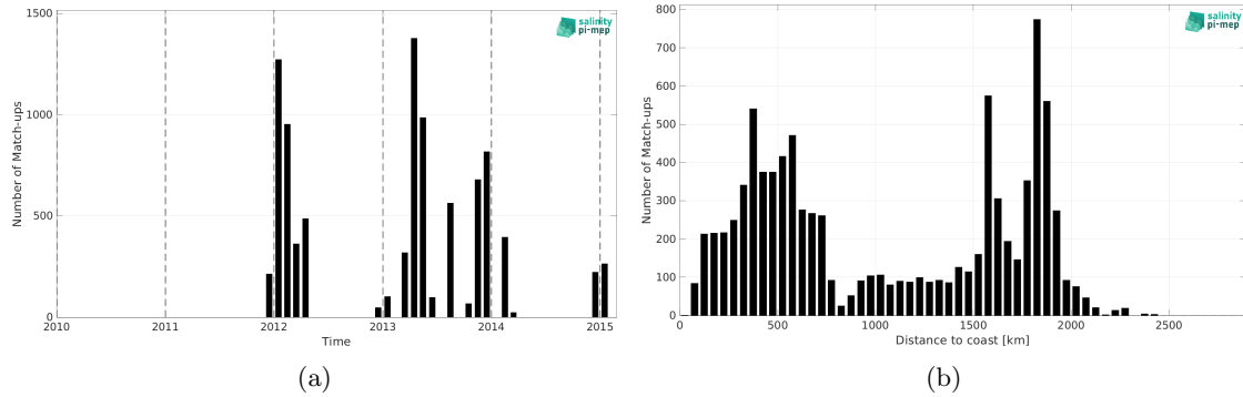
Figure 2: Number of match-ups between TSG (Polarstern) and Aquarius SSS L2 CAP v5 (JPL) SSS as a function of time (a) and as function of the distance to coast (b) over the Roaring Forties and Furious Fifties Pi-MEP region and for the full satellite product period.
