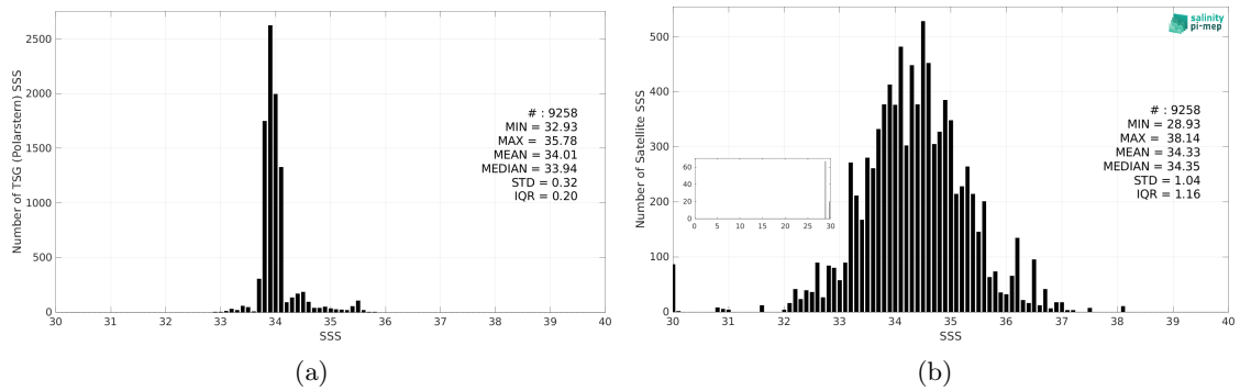
Figure 3: Histograms of SSS from TSG (Polarstern) (a) and Aquarius SSS L2 CAP v5 (JPL) (b) considering all match-up pairs per bins of 0.1 over the Roaring Forties and Furious Fifties Pi-MEP region and for the full satellite product period.
