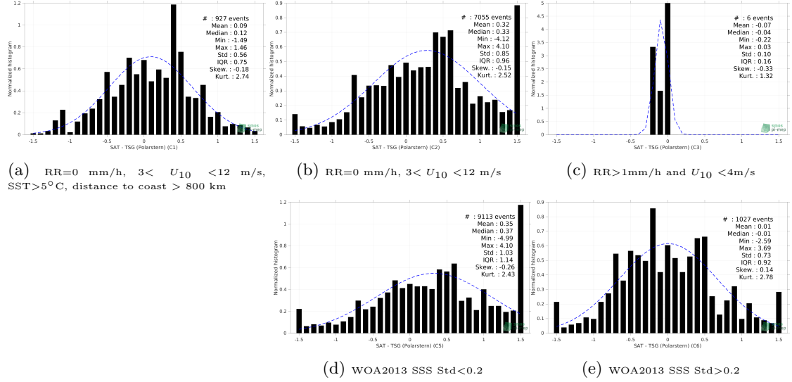
Figure 13: Normalized histogram of \Delta SSS (Aquarius SSS L2 CAP v5 (JPL) - TSG (Polarstern)) for 5 different subdatasets corresponding to: RR=0 mm/h, 3 < U_{10} < 12 m/s, SST>5°C, distance to coast > 800 km (a), RR=0 mm/h, 3 < U_{10} < 12 m/s (b), RR>1mm/h and U_{10} < 4 m/s (c), WOA2013 SSS Std<0.2 (d), WOA2013 SSS Std>0.2 (e).
