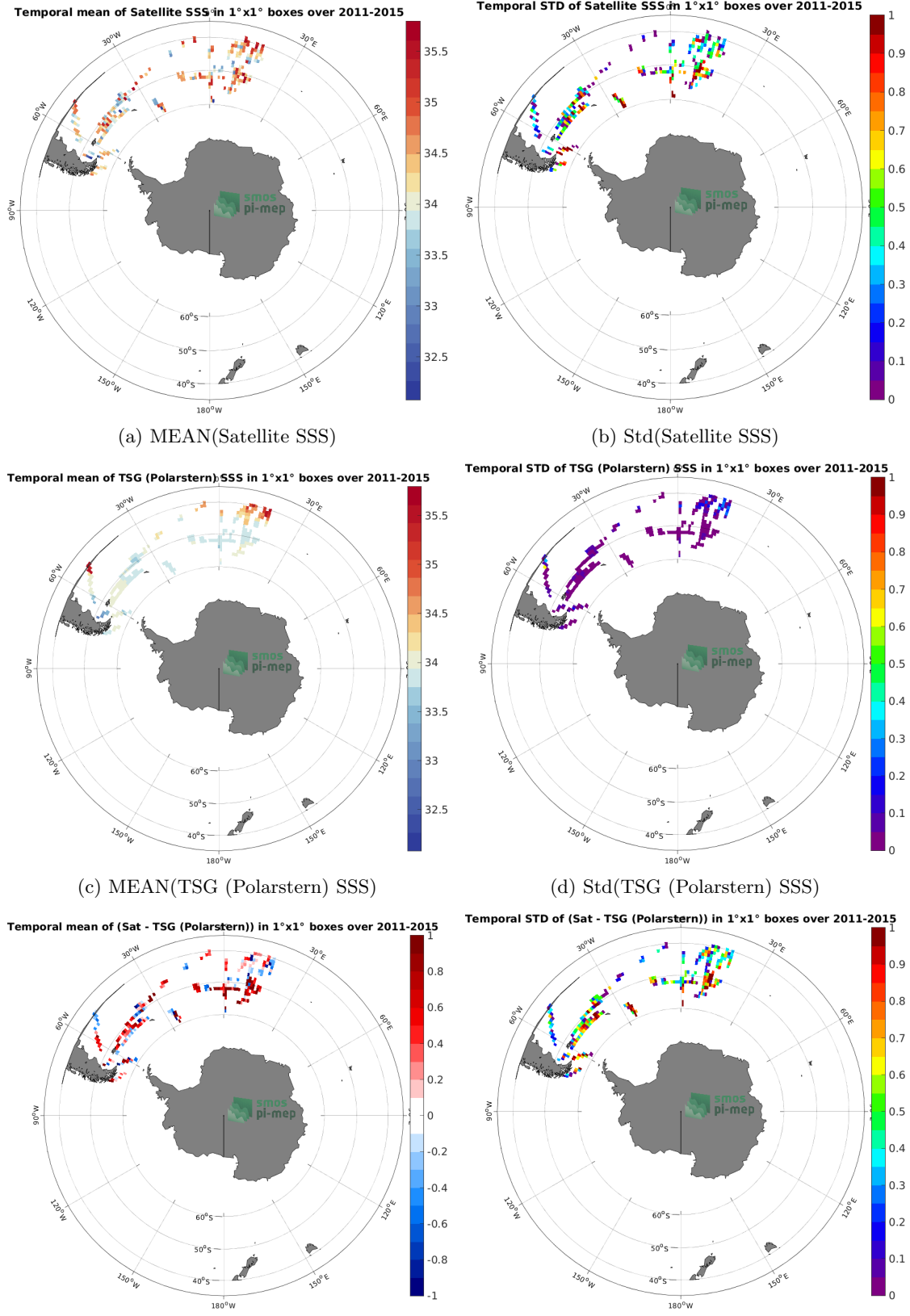
Figure 6: Temporal mean (left) and Std (right) of SSS from Aquarius SSS L2 CAP v5 (JPL) (top), TSG (Polarstern) (middle), and of \Delta SSS (Satellite - TSG (Polarstern)). Only match-up pairs are used to generate these maps.
