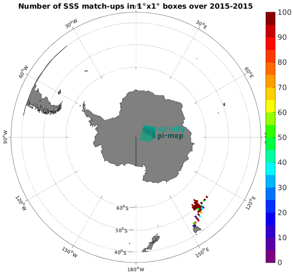
Figure 4: Number of SSS match-ups between TSG (GOSUD-Research-vessel) SSS and the Aquarius SSS L2 CAP v5 (JPL) SSS product for the Roaring Forties and Furious Fifties Pi-MEP region over 1^\circ \times 1^\circ boxes and for the full satellite product period.
