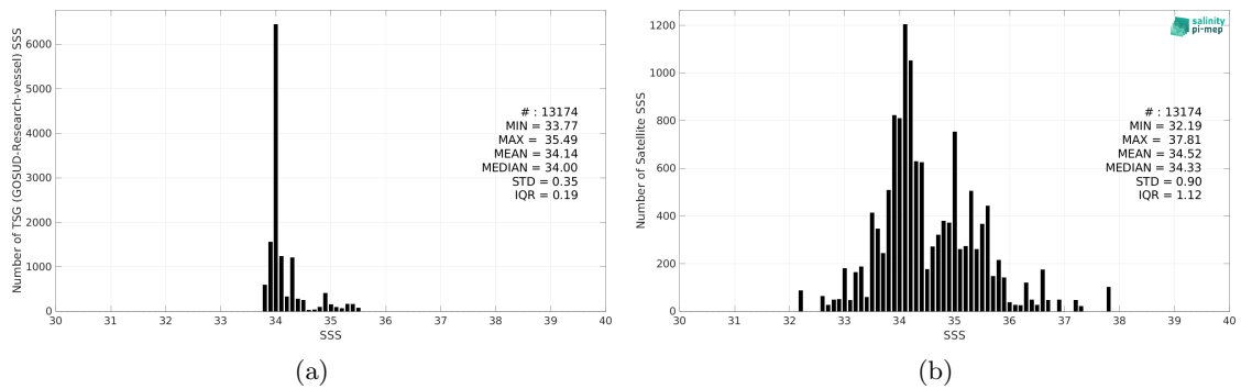
Figure 2: Histograms of SSS from TSG (GOSUD-Research-vessel) (a) and Aquarius SSS L2 CAP v5 (JPL) (b) considering all match-up pairs per bins of 0.1 over the Roaring Forties and Furious Fifties Pi-MEP region and for the full satellite product period.
