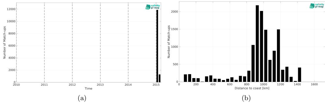
Figure 1: Number of match-ups between TSG (GOSUD-Research-vessel) and Aquarius SSS L2 CAP v5 (JPL) SSS as a function of time (a) and as function of the distance to coast (b) over the Roaring Forties and Furious Fifties Pi-MEP region and for the full satellite product period.
