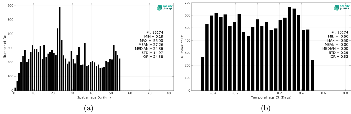
Figure 5: Histograms of the spatial (a) and temporal (b) lags between the location/time of the TSG (GOSUD-Research-vessel) measurement and the date of the corresponding Aquarius SSS L2 CAP v5 (JPL) SSS pixel.
