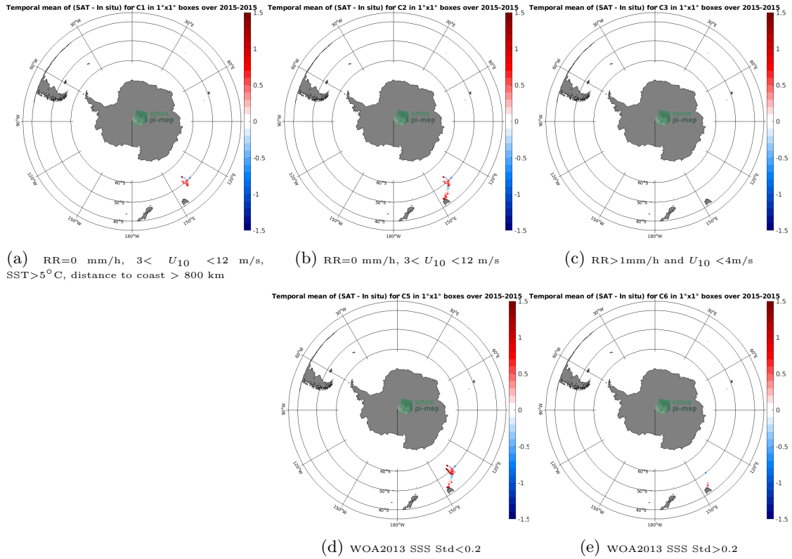
Figure 12: Temporal mean gridded over spatial boxes of size 1°x1° of \Delta SSS (Aquarius SSS L2 CAP v5 (JPL) - TSG (GOSUD-Research-vessel)) for 5 different subdatasets corresponding to:RR=0 mm/h, 3 < U_{10} < 12 m/s, SST>5°C, distance to coast > 800 km (a), RR=0 mm/h, 3 < U_{10} < 12 m/s (b), RR>1mm/h and U_{10} < 4 m/s (c), WOA2013 SSS Std<0.2 (d), WOA2013 SSS Std>0.2 (e).
