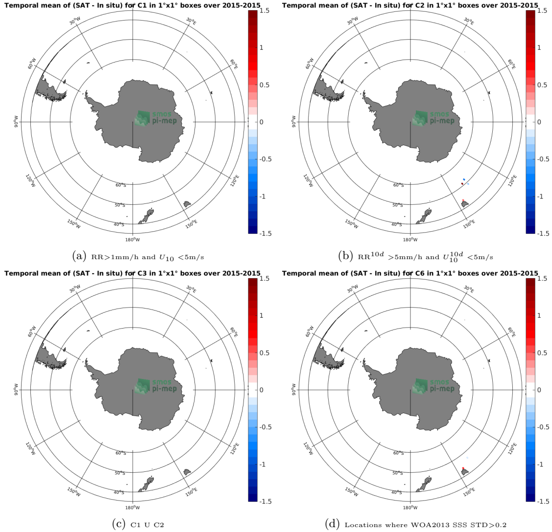
Figure 12: Temporal mean gridded over spatial boxes of size 1^\circ \times 1^\circ of \Delta SSS (Aquarius-L2-JPL-V5 - TSG-GOSUD-Research-vessel) for 4 different subdatasets corresponding to: RR > 1mm/h and U_{10} < 5 m/s (a), RR^{10d} > 5 mm/h and U_{10}^{10d} < 5 m/s (b), C1 U C2 (c), Locations where WOA2013 SSS STD > 0.2 (d).
