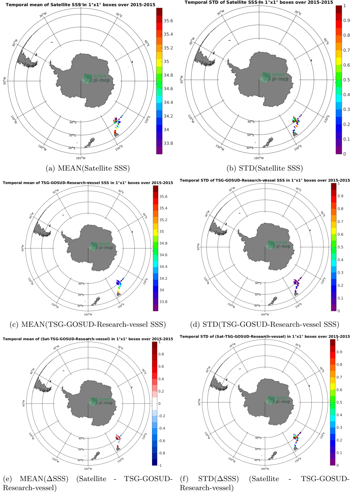
Figure 6: Temporal mean (left) and STD (right) of SSS from Aquarius-L2-JPL-V5 (top), TSG-GOSUD-Research-vessel (middle), and of \Delta SSS 18 (Satellite - TSG-GOSUD-Research-vessel). Only match-up pairs are used to generate these maps.
