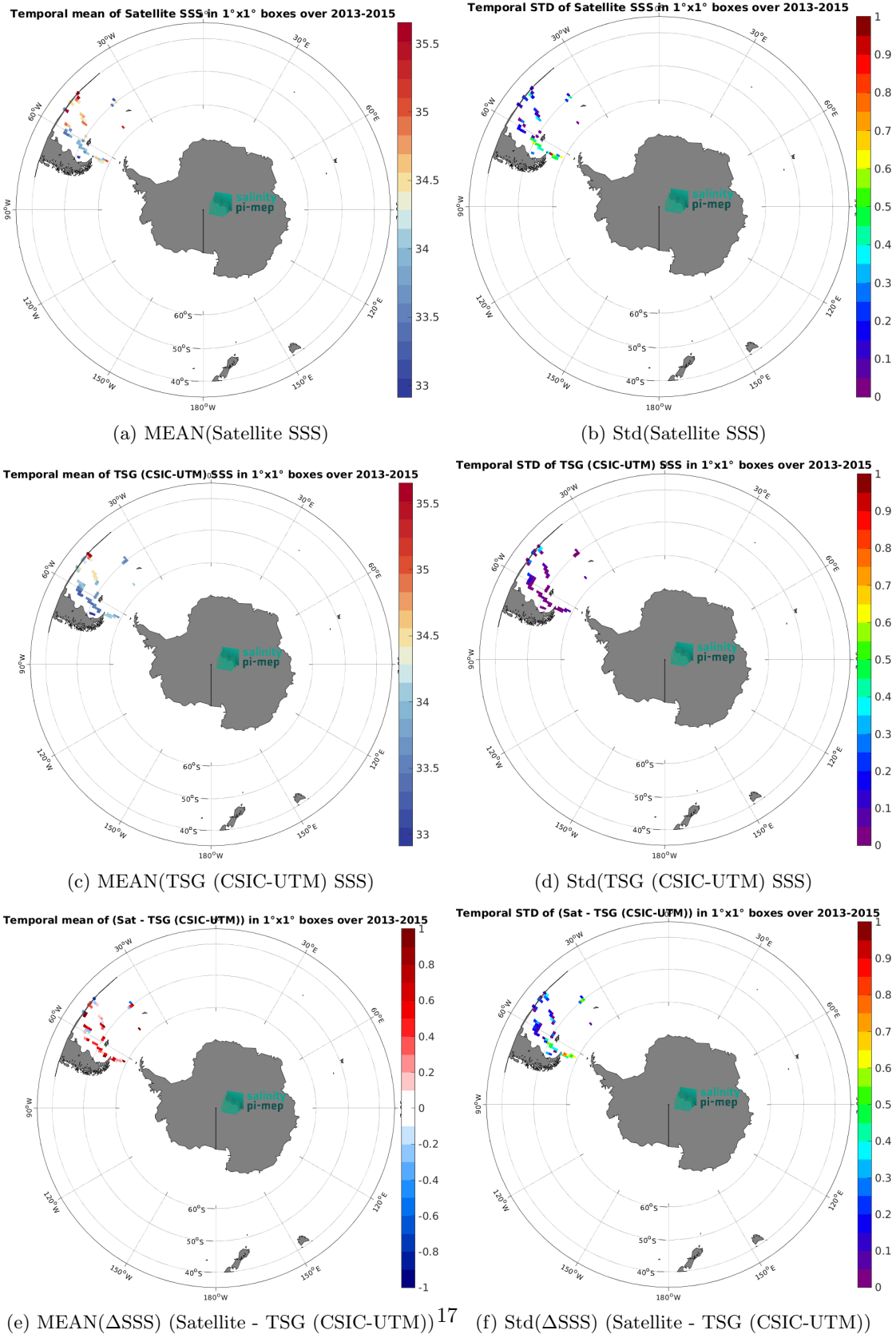
Figure 7: Temporal mean (left) and Std (right) of SSS from Aquarius SSS L2 CAP v5 (JPL) (top), TSG (CSIC-UTM) (middle), and of \Delta SSS (Satellite - TSG (CSIC-UTM)). Only match-up pairs are used to generate these maps.
