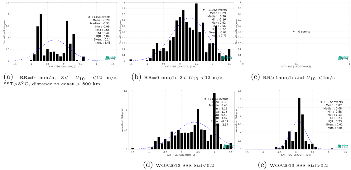
Figure 15: Normalized histogram of \Delta SSS (Aquarius SSS L2 CAP v5 (JPL) - TSG (CSIC-UTM)) for 5 different subdatasets corresponding to: RR=0 mm/h, 3 < U_{10} < 12 m/s, SST > 5°C, distance to coast > 800 km (a), RR=0 mm/h, 3 < U_{10} < 12 m/s (b), RR > 1mm/h and U_{10} < 4 m/s (c), WOA2013 SSS Std < 0.2 (d), WOA2013 SSS Std > 0.2 (e).
