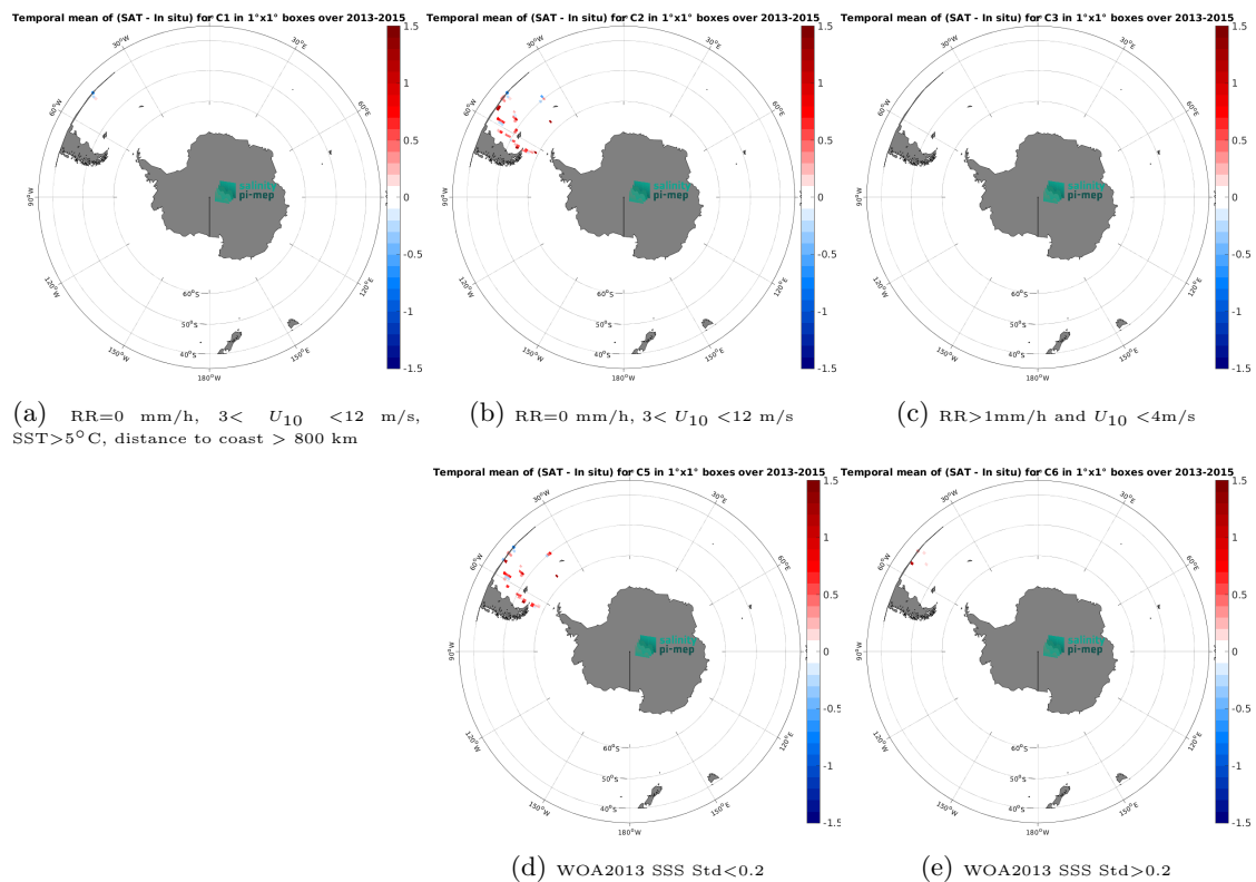
Figure 14: Temporal mean gridded over spatial boxes of size 1^\circ \times 1^\circ of \Delta SSS (Aquarius SSS L2 CAP v5 (JPL) - TSG (CSIC-UTM)) for 5 different subdatasets corresponding to: RR=0 mm/h, 3 < U_{10} < 12 m/s, SST > 5^\circ\text{C} , distance to coast > 800 km (a), RR=0 mm/h, 3 < U_{10} < 12 m/s (b), RR > 1 mm/h and U_{10} < 4 m/s (c), WOA2013 SSS Std < 0.2 (d), WOA2013 SSS Std > 0.2 (e).
