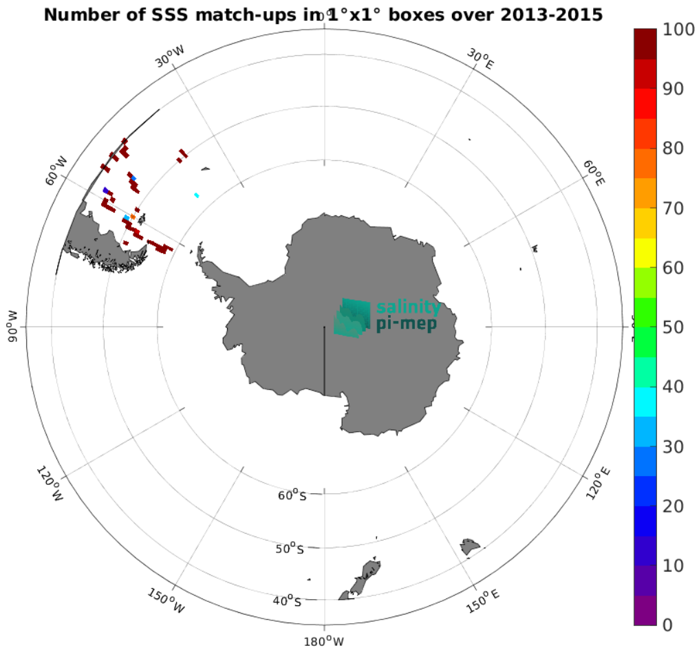
Figure 5: Number of SSS match-ups between TSG (CSIC-UTM) SSS and the Aquarius SSS L2 CAP v5 (JPL) SSS product for the Roaring Forties and Furious Fifties Pi-MEP region over 1^\circ \times 1^\circ boxes and for the full satellite product period.
