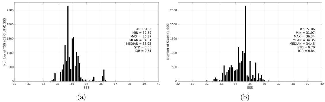
Figure 3: Histograms of SSS from TSG (CSIC-UTM) (a) and Aquarius SSS L2 CAP v5 (JPL) (b) considering all match-up pairs per bins of 0.1 over the Roaring Forties and Furious Fifties Pi-MEP region and for the full satellite product period.
