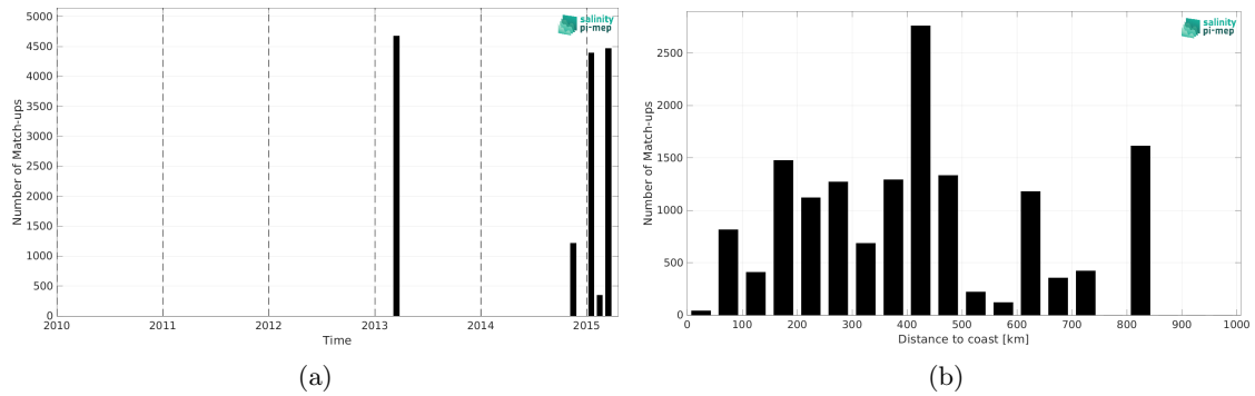
Figure 2: Number of match-ups between TSG (CSIC-UTM) and Aquarius SSS L2 CAP v5 (JPL) SSS as a function of time (a) and as function of the distance to coast (b) over the Roaring Forties and Furious Fifties Pi-MEP region and for the full satellite product period.
