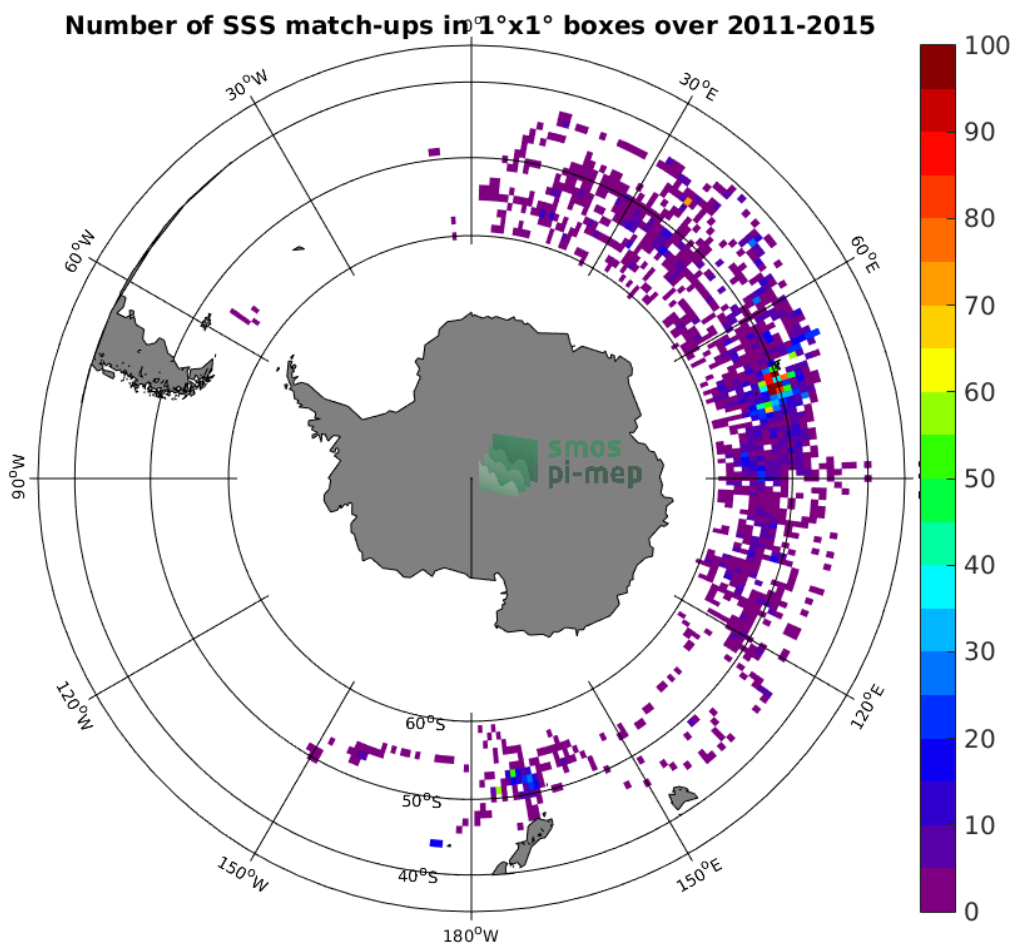
Figure 4: Number of SSS match-ups between Sea mammals SSS and the Aquarius-L2-JPL-V5 SSS product for the Roaring Forties and Furious Fifties Pi-MEP region over 1^\circ \times 1^\circ boxes and for the full satellite product period.
