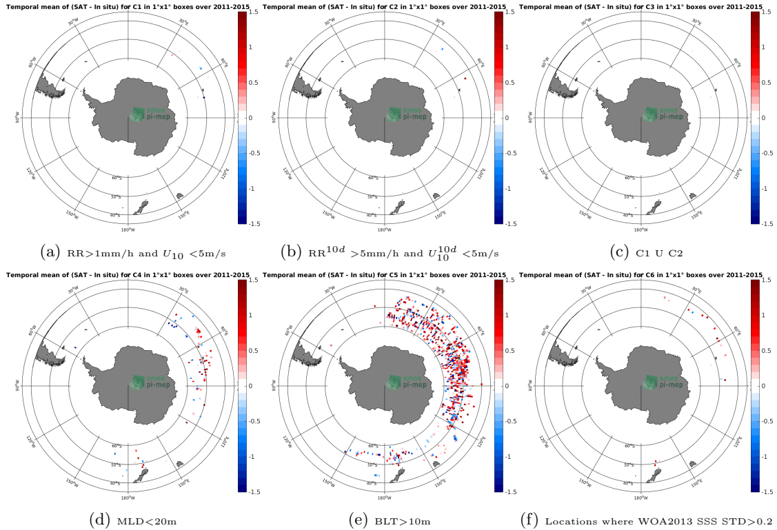
Figure 12: Temporal mean gridded over spatial boxes of size 1^\circ \times 1^\circ of \Delta SSS (Aquarius-L2-JPL-V5 - Sea mammals) for 6 different subdatasets corresponding to: RR > 1\text{mm/h} and U_{10} < 5\text{m/s} (a), RR^{10d} > 5\text{mm/h} and U_{10}^{10d} < 5\text{m/s} (b), C1 U C2 (c), MLD < 20\text{m} (d), BLT > 10\text{m} (e), Locations where WOA2013 SSS STD > 0.2 (f).
