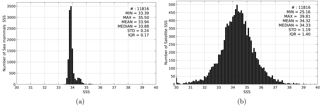
Figure 2: Histograms of SSS from Sea mammals (a) and AQUARIUS-L2-JPL-V4 (b) considering all match-up pairs per bins of 0.1 over the Roaring Forties and Furious Fifties Pi-MEP region and for the full satellite product period.
