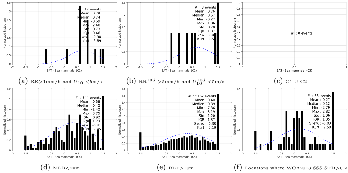
Figure 13: Normalized histogram of \Delta SSS (AQUARIUS-L2-JPL-V4 - Sea mammals) for 6 different subdatasets corresponding to: RR>1mm/h and U_{10} < 5\text{m/s} (a), RR^{10d} > 5\text{mm/h} and U_{10}^{10d} < 5\text{m/s} (b), C1 U C2 (c), MLD<20m (d), BLT>10m (e), Locations where WOA2013 SSS STD>0.2 (f).
