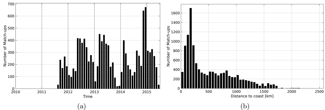
Figure 1: Number of match-ups between Sea mammals and AQUARIUS-L2-JPL-V4 SSS as a function of time (a) and as function of the distance to coast (b) over the Roaring Forties and Furious Fifties Pi-MEP region and for the full satellite product period.
