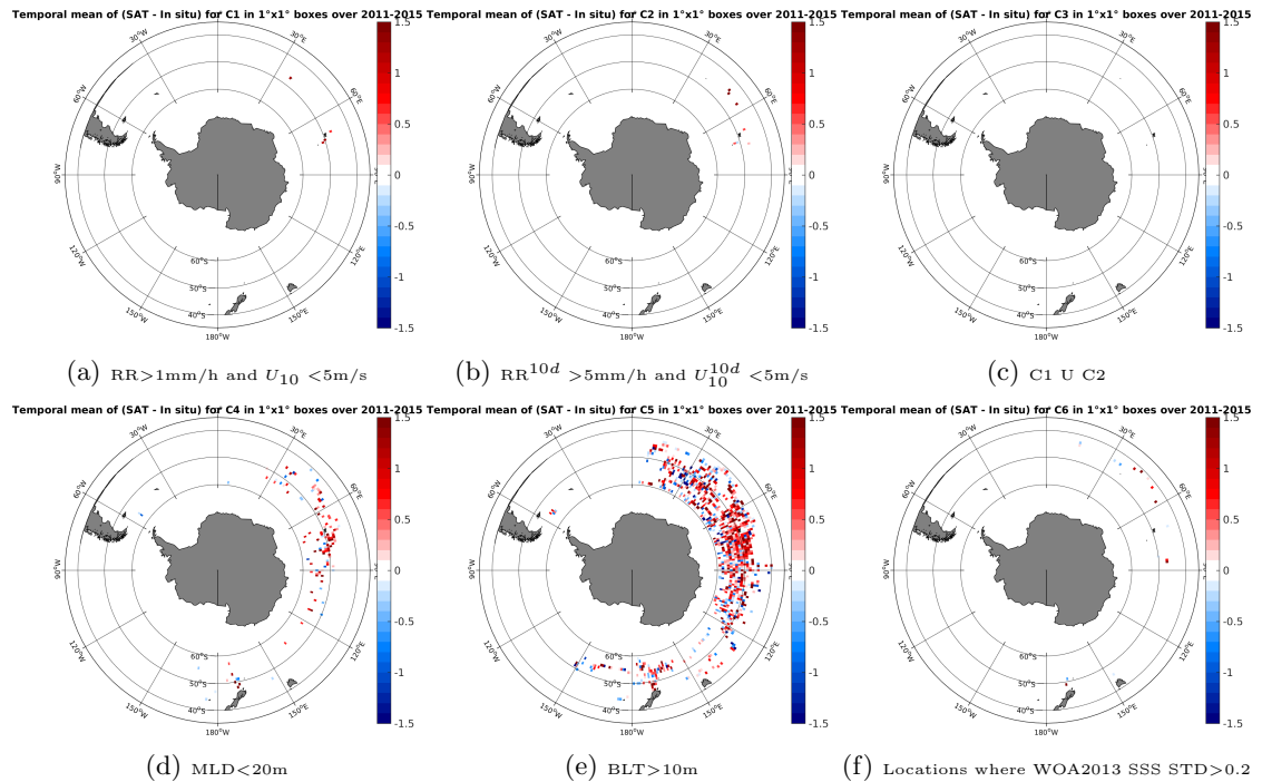
Figure 12: Temporal mean gridded over spatial boxes of size 1°x1° of \Delta SSS (AQUARIUS-L2-JPL-V4 - Sea mammals) for 6 different subdatasets corresponding to: RR > 1\text{mm/h} and U_{10} < 5\text{m/s} (a), RR^{10d} > 5\text{mm/h} and U_{10}^{10d} < 5\text{m/s} (b), C1 U C2 (c), MLD < 20\text{m} (d), BLT > 10\text{m} (e), Locations where WOA2013 SSS STD > 0.2 (f).
