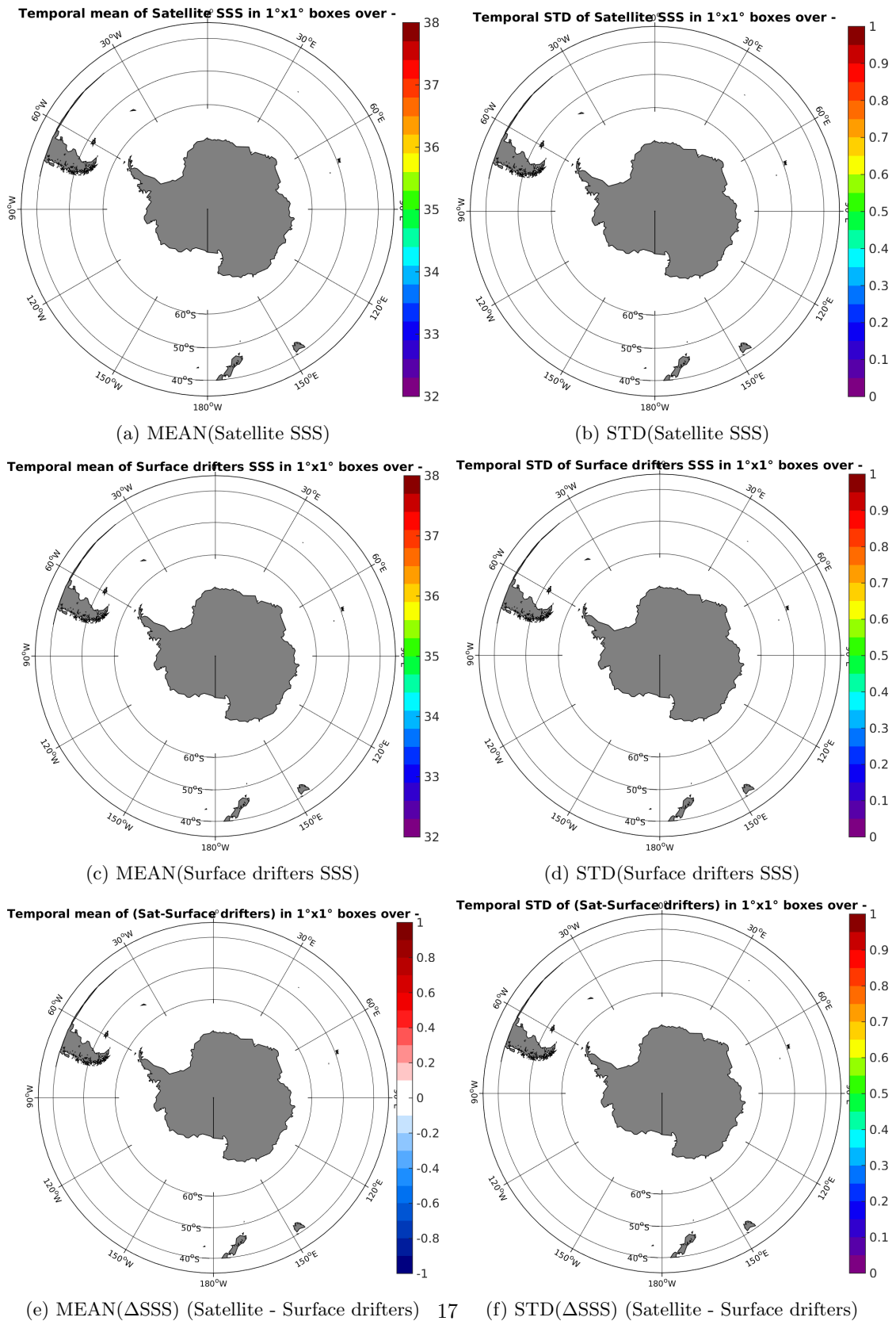
Figure 5: Temporal mean (left) and STD (right) of SSS from AQUARIUS-L2-JPL-V4 (top), Surface drifters (middle), and of \Delta SSS (Satellite - Surface drifters). Only match-up pairs are used to generate these maps.
