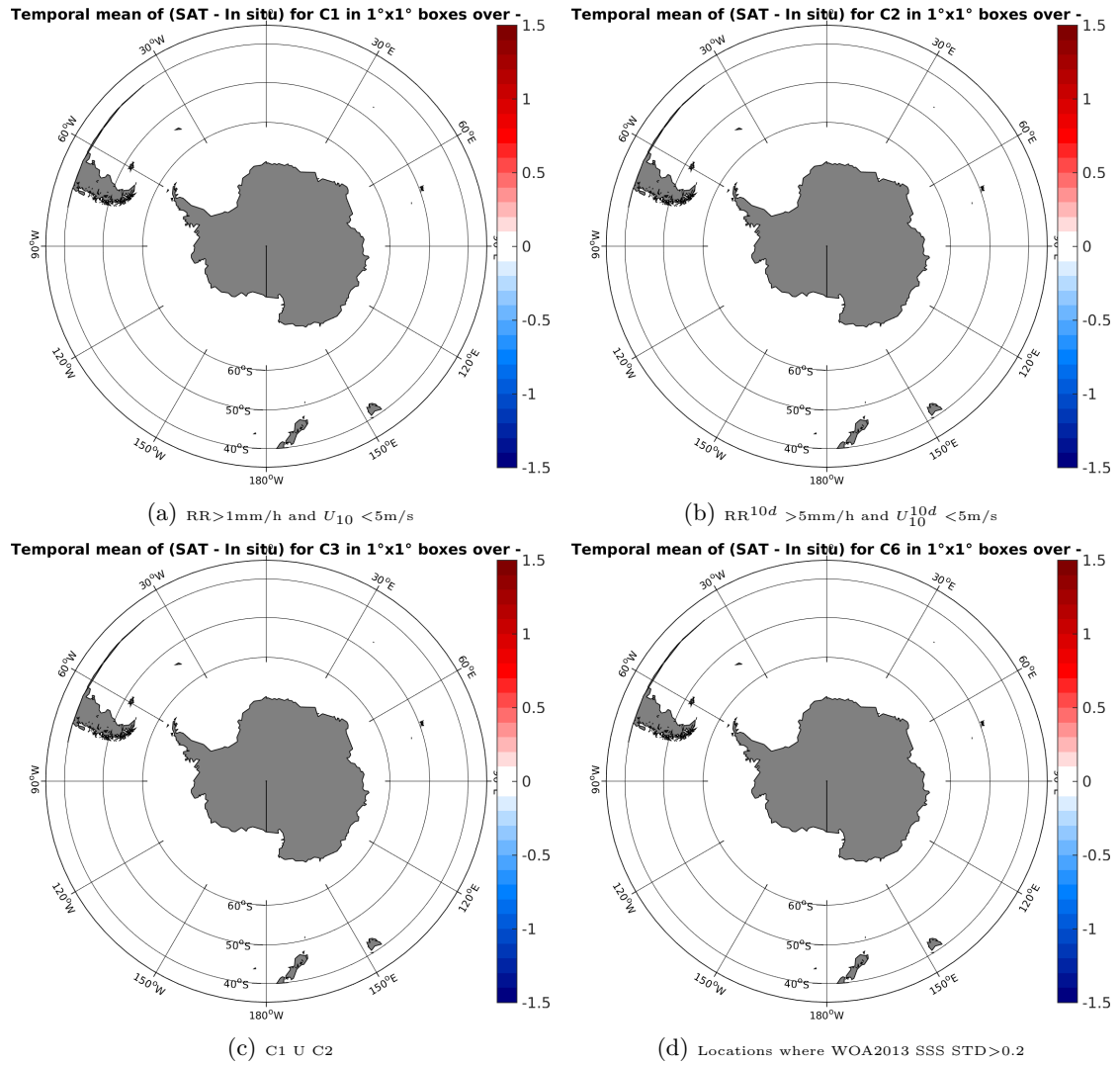
Figure 11: Temporal mean gridded over spatial boxes of size 1°x1° of \Delta SSS (AQUARIUS-L2-JPL-V4 - Surface drifters) for 4 different subdatasets corresponding to:RR>1mm/h and U_{10} < 5\text{m/s} (a), RR^{10d} > 5\text{mm/h} and U_{10}^{10d} < 5\text{m/s} (b), C1 U C2 (c),Locations where WOA2013 SSS STD>0.2 (d).
