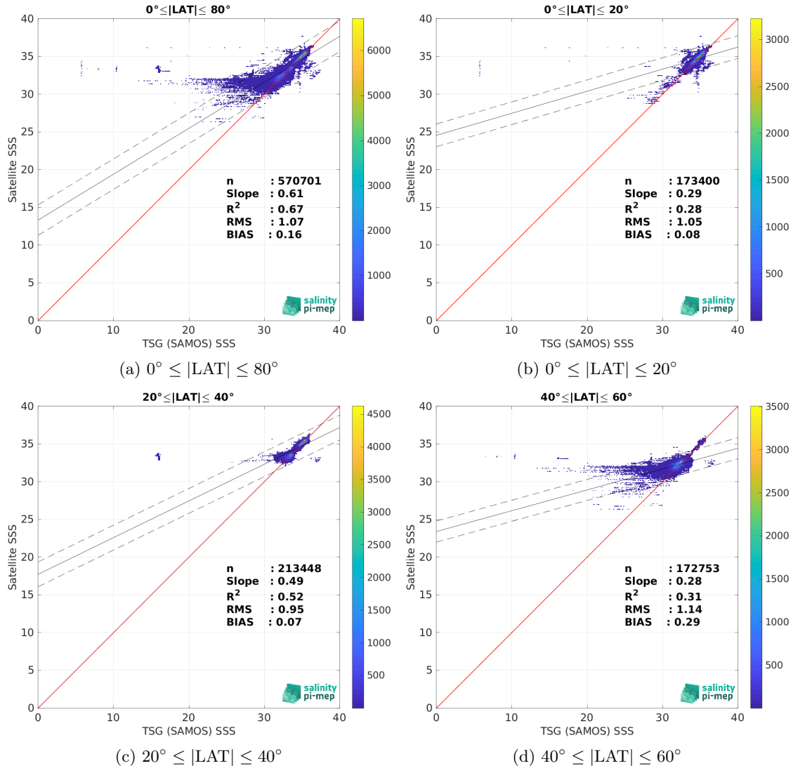
Figure 9: Contour maps of the concentration of SMOS and SMAP SSS L4 OI v1 - 7 Days (LOPS) SSS (y-axis) versus TSG (SAMOS) SSS (x-axis) at match-up pairs for different latitude bands. For each plot, the red line shows x=y . The black thin and dashed lines indicate a linear fit through the data cloud and the \pm 95\% confidence levels, respectively. The number match-up pairs n , the slope and R^2 coefficient of the linear fit, the root mean square (RMS) and the mean bias between satellite and in situ data are indicated for each latitude band in each plots.
