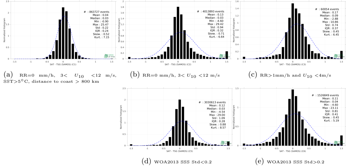
Figure 13: Normalized histogram of \Delta SSS (SMOS and SMAP SSS L4 OI v1 - 7 Days (LOPS) - TSG (SAMOS)) for 5 different subdatasets corresponding to: RR=0 mm/h, 3 < U_{10} < 12 m/s, SST > 5°C, distance to coast > 800 km (a), RR=0 mm/h, 3 < U_{10} < 12 m/s (b), RR > 1mm/h and U_{10} < 4 m/s (c), WOA2013 SSS Std < 0.2 (d), WOA2013 SSS Std > 0.2 (e).
