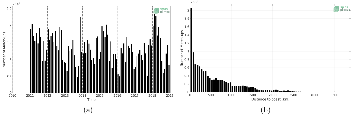
Figure 1: Number of match-ups between TSG (LEGOS-DM) and SMOS and SMAP SSS L4 OI v1 - 7 Days (LOPS) SSS as a function of time (a) and as function of the distance to coast (b) over the Pacific Ocean Pi-MEP region and for the full satellite product period.
