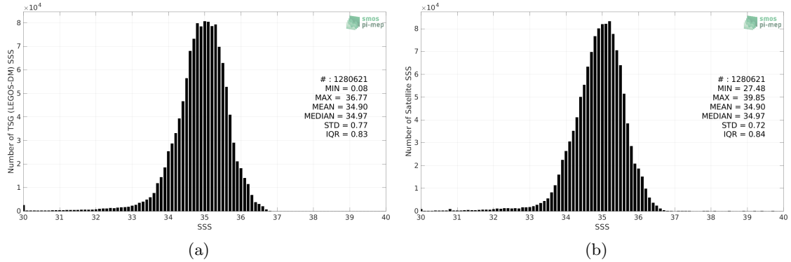
Figure 2: Histograms of SSS from TSG (LEGOS-DM) (a) and SMOS and SMAP SSS L4 OI v1 - 7 Days (LOPS) (b) considering all match-up pairs per bins of 0.1 over the Pacific Ocean Pi-MEP region and for the full satellite product period.
