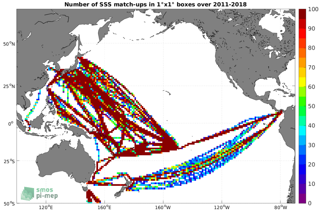
Figure 4: Number of SSS match-ups between TSG (LEGOS-DM) SSS and the SMOS and SMAP SSS L4 OI v1 - 7 Days (LOPS) SSS product for the Pacific Ocean Pi-MEP region over 1^\circ \times 1^\circ boxes and for the full satellite product period.
