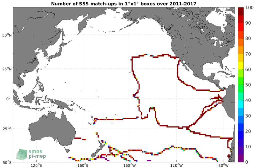
Figure 4: Number of SSS match-ups between TSG (GOSUD-Sailing-ship) SSS and the SMOS and SMAP SSS L4 OI v1 - 7 Days (LOPS) SSS product for the Pacific Ocean Pi-MEP region over 1^\circ \times 1^\circ boxes and for the full satellite product period.
