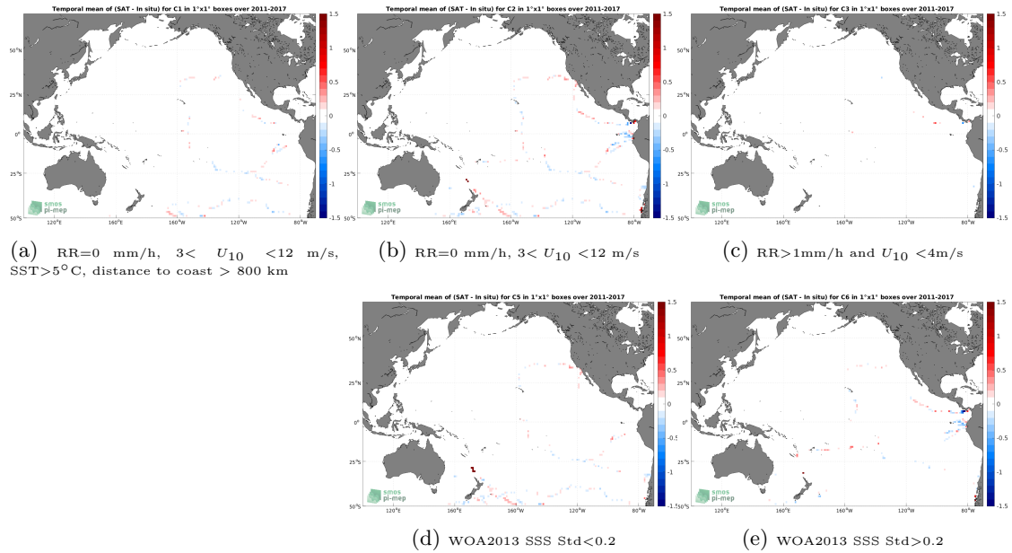
Figure 12: Temporal mean gridded over spatial boxes of size 1^\circ \times 1^\circ of \Delta SSS (SMOS and SMAP SSS L4 OI v1 - 7 Days (LOPS) - TSG (GOSUD-Sailing-ship)) for 5 different subdatasets corresponding to:RR=0 mm/h, 3 < U_{10} < 12 m/s, SST >5^\circ\text{C} , distance to coast > 800 km (a), RR=0 mm/h, 3 < U_{10} < 12 m/s (b), RR >1 mm/h and U_{10} < 4 m/s (c), WOA2013 SSS Std <0.2 (d), WOA2013 SSS Std >0.2 (e).
