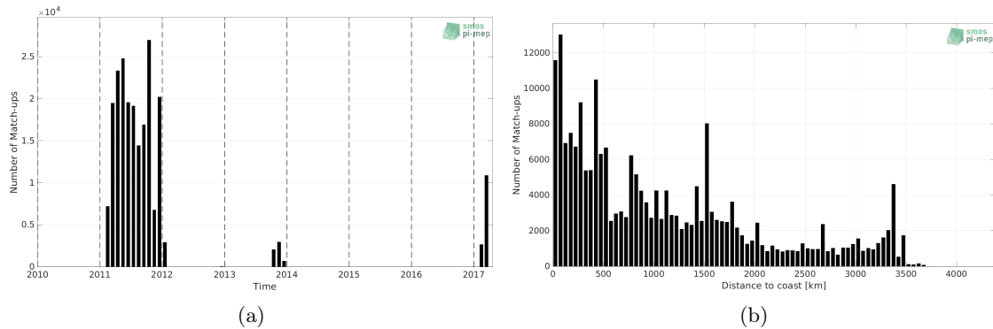
Figure 1: Number of match-ups between TSG (GOSUD-Sailing-ship) and SMOS and SMAP SSS L4 OI v1 - 7 Days (LOPS) SSS as a function of time (a) and as function of the distance to coast (b) over the Pacific Ocean Pi-MEP region and for the full satellite product period.
