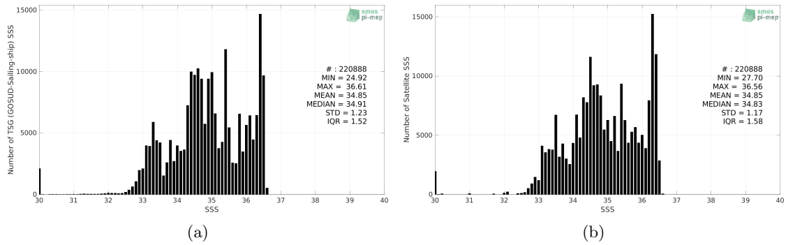
Figure 2: Histograms of SSS from TSG (GOSUD-Sailing-ship) (a) and SMOS and SMAP SSS L4 OI v1 - 7 Days (LOPS) (b) considering all match-up pairs per bins of 0.1 over the Pacific Ocean Pi-MEP region and for the full satellite product period.
