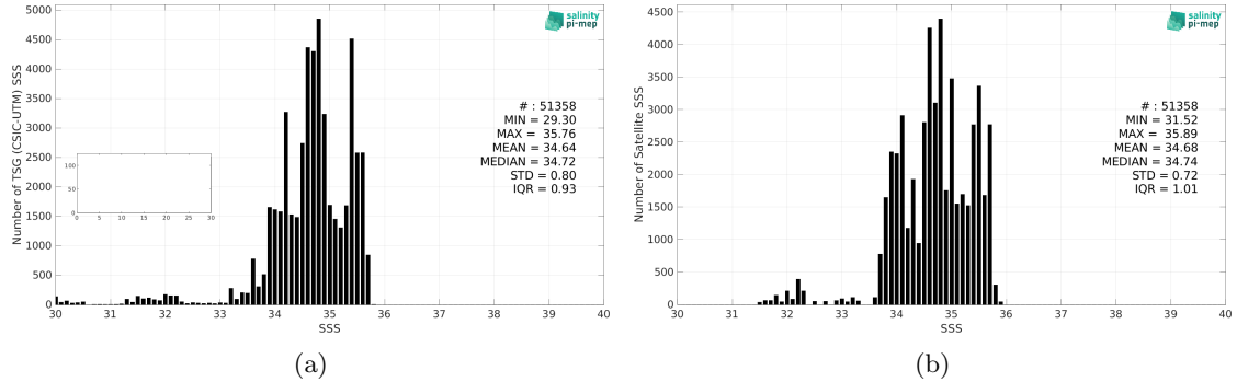
Figure 2: Histograms of SSS from TSG (CSIC-UTM) (a) and SMOS and SMAP SSS L4 OI v1 - 7 Days (LOPS) (b) considering all match-up pairs per bins of 0.1 over the Pacific Ocean Pi-MEP region and for the full satellite product period.
