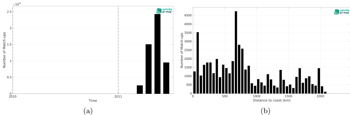
Figure 1: Number of match-ups between TSG (CSIC-UTM) and SMOS and SMAP SSS L4 OI v1 - 7 Days (LOPS) SSS as a function of time (a) and as function of the distance to coast (b) over the Pacific Ocean Pi-MEP region and for the full satellite product period.
