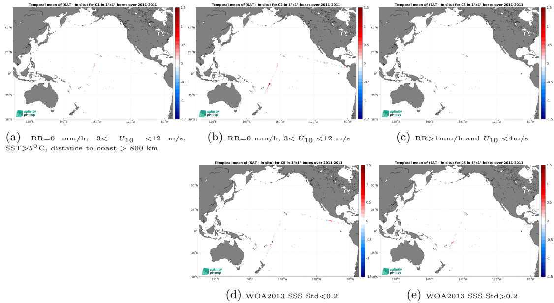
Figure 12: Temporal mean gridded over spatial boxes of size 1^\circ \times 1^\circ of \Delta SSS (SMOS and SMAP SSS L4 OI v1 - 7 Days (LOPS) - TSG (CSIC-UTM)) for 5 different subdatasets corresponding to:RR=0 mm/h, 3 < U_{10} < 12 m/s, SST >5^\circ C, distance to coast > 800 km (a), RR=0 mm/h, 3 < U_{10} < 12 m/s (b), RR >1 mm/h and U_{10} < 4 m/s (c), WOA2013 SSS Std <0.2 (d), WOA2013 SSS Std >0.2 (e).
