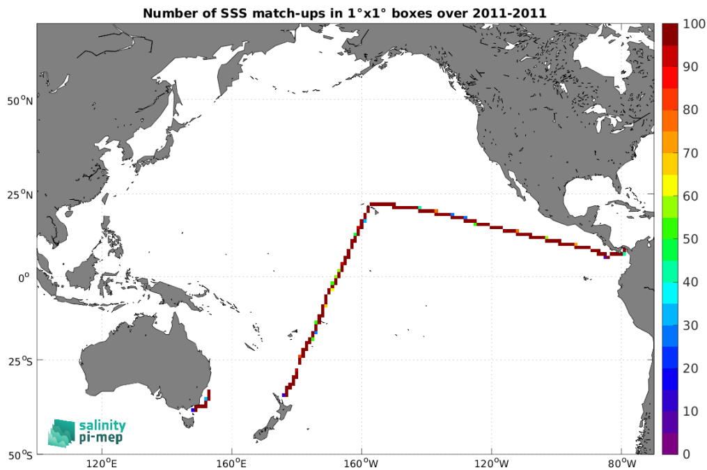
Figure 4: Number of SSS match-ups between TSG (CSIC-UTM) SSS and the SMOS and SMAP SSS L4 OI v1 - 7 Days (LOPS) SSS product for the Pacific Ocean Pi-MEP region over 1^\circ \times 1^\circ boxes and for the full satellite product period.
