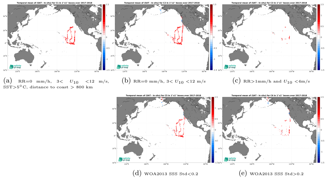
Figure 12: Temporal mean gridded over spatial boxes of size 1^\circ \times 1^\circ of \Delta SSS (SMOS and SMAP SSS L4 OI v1 - 7 Days (LOPS) - Sairdrone) for 5 different subdatasets corresponding to:RR=0 mm/h, 3 < U_{10} < 12 m/s, SST >5^\circ C, distance to coast > 800 km (a), RR=0 mm/h, 3 < U_{10} < 12 m/s (b), RR >1 mm/h and U_{10} < 4 m/s (c), WOA2013 SSS Std <0.2 (d), WOA2013 SSS Std >0.2 (e).
