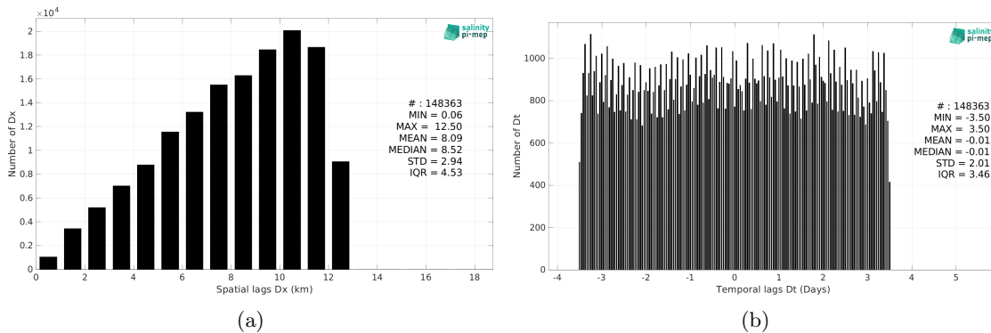
Figure 5: Histograms of the spatial (a) and temporal (b) lags between the location/time of the Saildrone measurement and the date of the corresponding SMOS and SMAP SSS L4 OI v1 - 7 Days (LOPS) SSS pixel.
