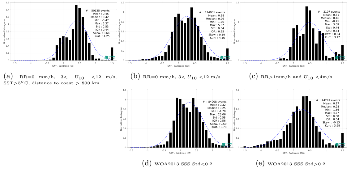
Figure 13: Normalized histogram of \Delta SSS (SMOS and SMAP SSS L4 OI v1 - 7 Days (LOPS) - Saildrone) for 5 different subdatasets corresponding to: RR=0 mm/h, 3 < U_{10} < 12 m/s, SST>5°C, distance to coast > 800 km (a), RR=0 mm/h, 3 < U_{10} < 12 m/s (b), RR>1mm/h and U_{10} < 4 m/s (c), WOA2013 SSS Std<0.2 (d), WOA2013 SSS Std>0.2 (e).
