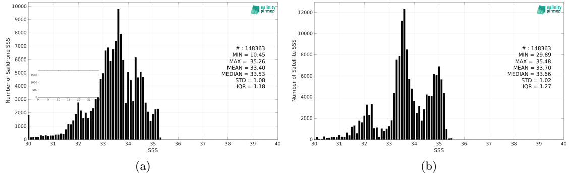
Figure 2: Histograms of SSS from Sairdrone (a) and SMOS and SMAP SSS L4 OI v1 - 7 Days (LOPS) (b) considering all match-up pairs per bins of 0.1 over the Pacific Ocean Pi-MEP region and for the full satellite product period.
