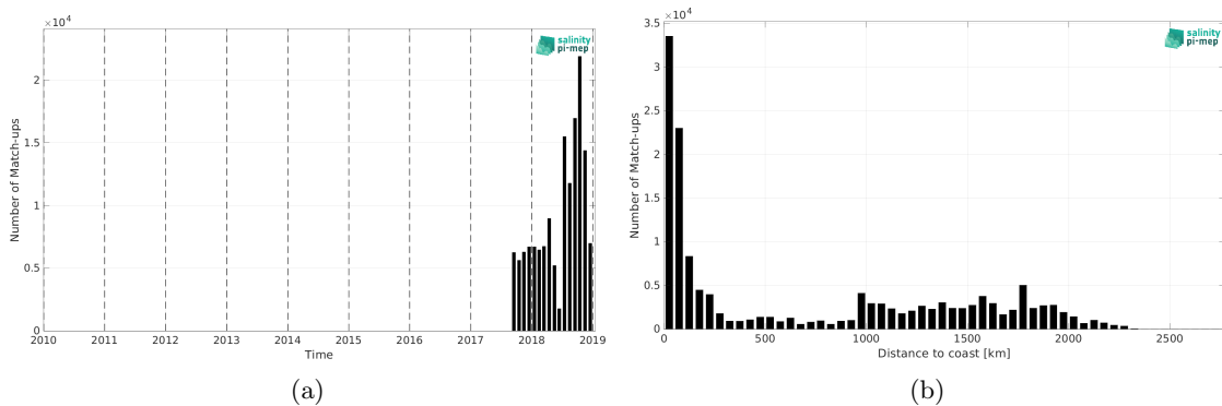
Figure 1: Number of match-ups between Saildrone and SMOS and SMAP SSS L4 OI v1 - 7 Days (LOPS) SSS as a function of time (a) and as function of the distance to coast (b) over the Pacific Ocean Pi-MEP region and for the full satellite product period.
