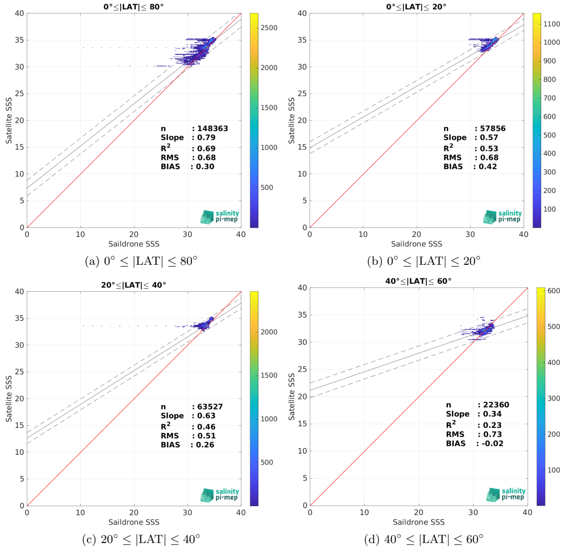
Figure 9: Contour maps of the concentration of SMOS and SMAP SSS L4 OI v1 - 7 Days (LOPS) SSS (y-axis) versus Saildrone SSS (x-axis) at match-up pairs for different latitude bands. For each plot, the red line shows x=y . The black thin and dashed lines indicate a linear fit through the data cloud and the \pm 95\% confidence levels, respectively. The number match-up pairs n , the slope and R^2 coefficient of the linear fit, the root mean square (RMS) and the mean bias between satellite and in situ data are indicated for each latitude band in each plots.
