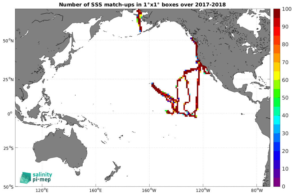
Figure 4: Number of SSS match-ups between Saildrone SSS and the SMOS and SMAP SSS L4 OI v1 - 7 Days (LOPS) SSS product for the Pacific Ocean Pi-MEP region over 1^\circ \times 1^\circ boxes and for the full satellite product period.
