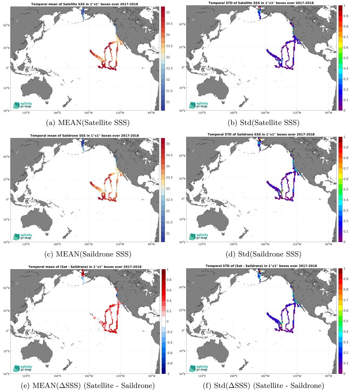
Figure 6: Temporal mean (left) and Std (right) of SSS from SMOS and SMAP SSS L4 OI v1 - 7 Days (LOPS) (top), Saildrone (middle), and of \Delta SSS (Satellite - Saildrone). Only match-up pairs are used to generate these maps.
