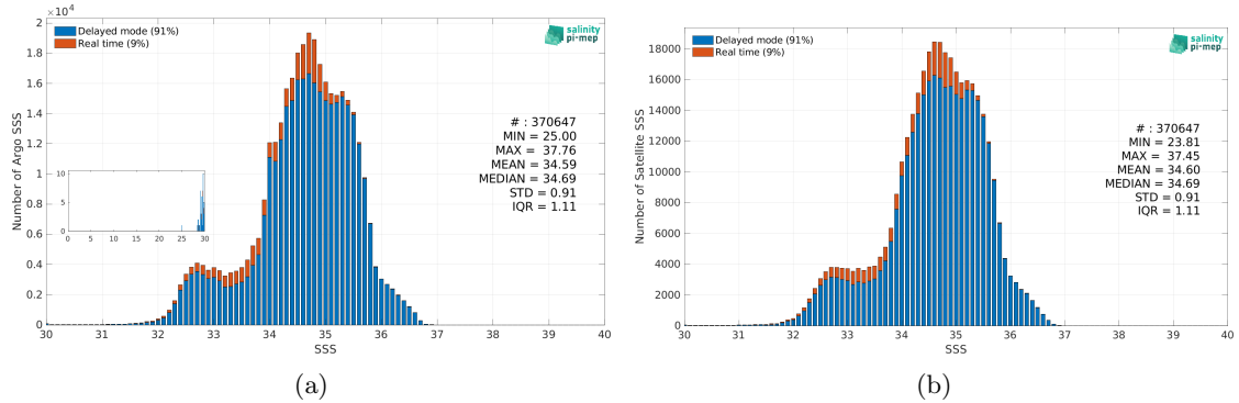
Figure 2: Histograms of SSS from Argo (a) and SMOS and SMAP SSS L4 OI v1 - 7 Days (LOPS) (b) considering all match-up pairs per bins of 0.1 over the Pacific Ocean Pi-MEP region and for the full satellite product period.
