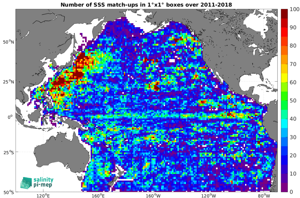
Figure 4: Number of SSS match-ups between Argo SSS and the SMOS and SMAP SSS L4 OI v1 - 7 Days (LOPS) SSS product for the Pacific Ocean Pi-MEP region over 1^\circ \times 1^\circ boxes and for the full satellite product period.
