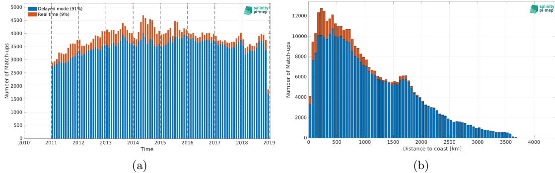
Figure 1: Number of match-ups between Argo and SMOS and SMAP SSS L4 OI v1 - 7 Days (LOPS) SSS as a function of time (a) and as function of the distance to coast (b) over the Pacific Ocean Pi-MEP region and for the full satellite product period.
