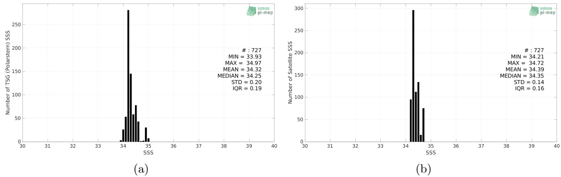
Figure 2: Histograms of SSS from TSG (Polarstern) (a) and SMOS SSS L4 v1 - Weekly (CMEMS-CNR) (b) considering all match-up pairs per bins of 0.1 over the Pacific Ocean Pi-MEP region and for the full satellite product period.
