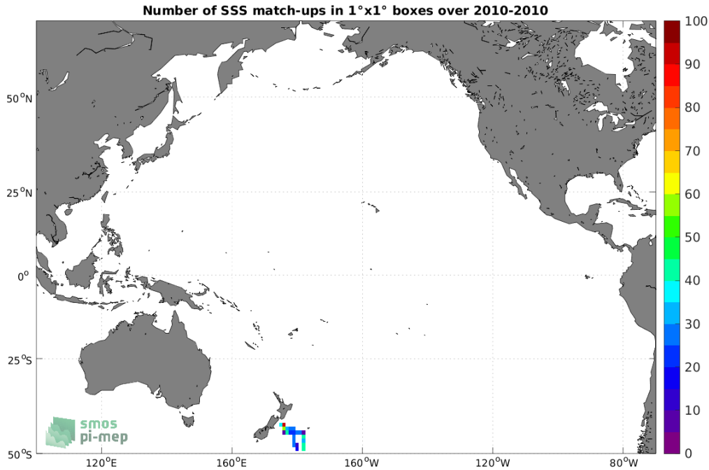
Figure 4: Number of SSS match-ups between TSG (Polarstern) SSS and the SMOS SSS L4 v1 - Weekly (CMEMS-CNR) SSS product for the Pacific Ocean Pi-MEP region over 1^\circ \times 1^\circ boxes and for the full satellite product period.
