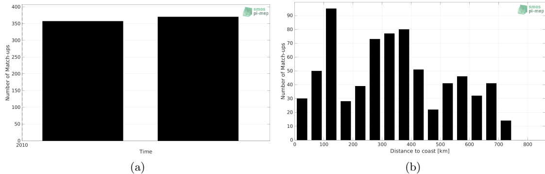
Figure 1: Number of match-ups between TSG (Polarstern) and SMOS SSS L4 v1 - Weekly (CMEMS-CNR) SSS as a function of time (a) and as function of the distance to coast (b) over the Pacific Ocean Pi-MEP region and for the full satellite product period.
