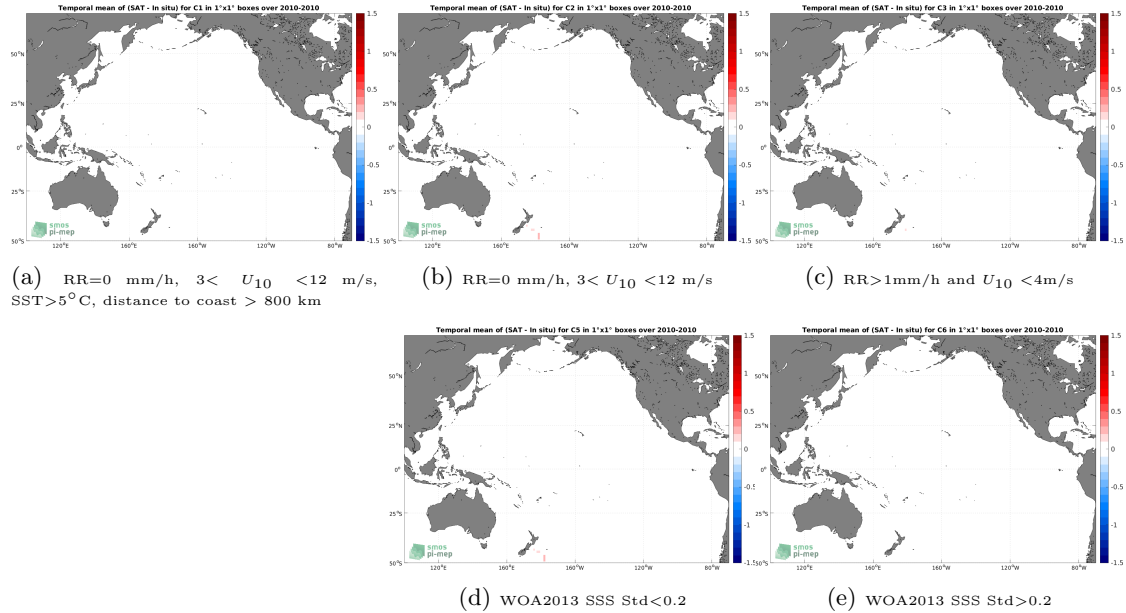
Figure 12: Temporal mean gridded over spatial boxes of size 1^{\circ}\times 1^{\circ} of \Delta\text{SSS} (SMOS SSS L4 v1 - Weekly (CMEMS-CNR) - TSG (Polarstern)) for 5 different subdatasets corresponding to: \text{RR}=0 mm/h, 3 < U_{10} < 12 m/s, \text{SST} > 5^{\circ}\text{C} , distance to coast > 800 km (a), \text{RR}=0 mm/h, 3 < U_{10} < 12 m/s (b), \text{RR} > 1 mm/h and U_{10} < 4 m/s (c), WOA2013 SSS Std < 0.2 (d), WOA2013 SSS Std > 0.2 (e).
