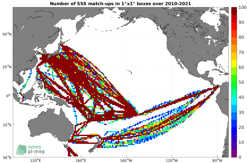
Figure 4: Number of SSS match-ups between TSG (LEGOS-DM) SSS and the SMOS SSS L4 v1 - Weekly (CMEMS-CNR) SSS product for the Pacific Ocean Pi-MEP region over 1^\circ \times 1^\circ boxes and for the full satellite product period.
