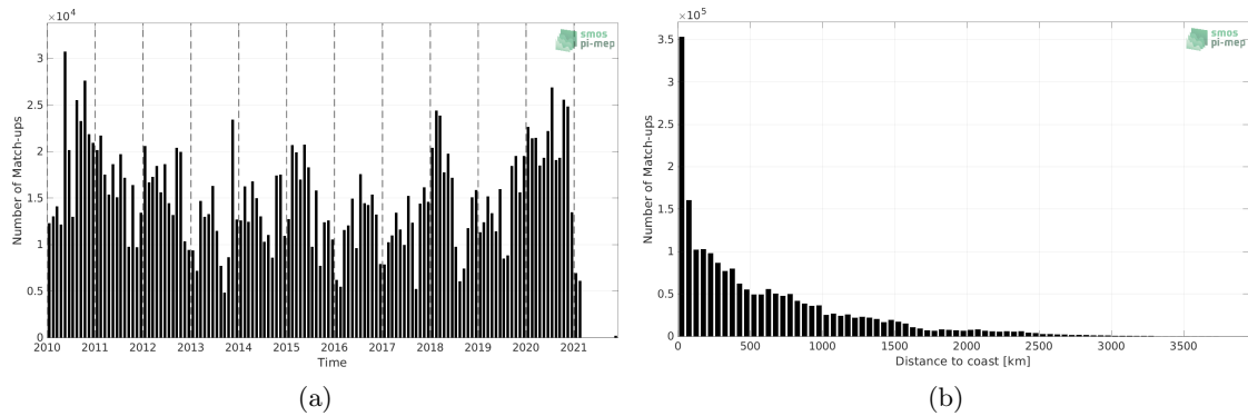
Figure 1: Number of match-ups between TSG (LEGOS-DM) and SMOS SSS L4 v1 - Weekly (CMEMS-CNR) SSS as a function of time (a) and as function of the distance to coast (b) over the Pacific Ocean Pi-MEP region and for the full satellite product period.
