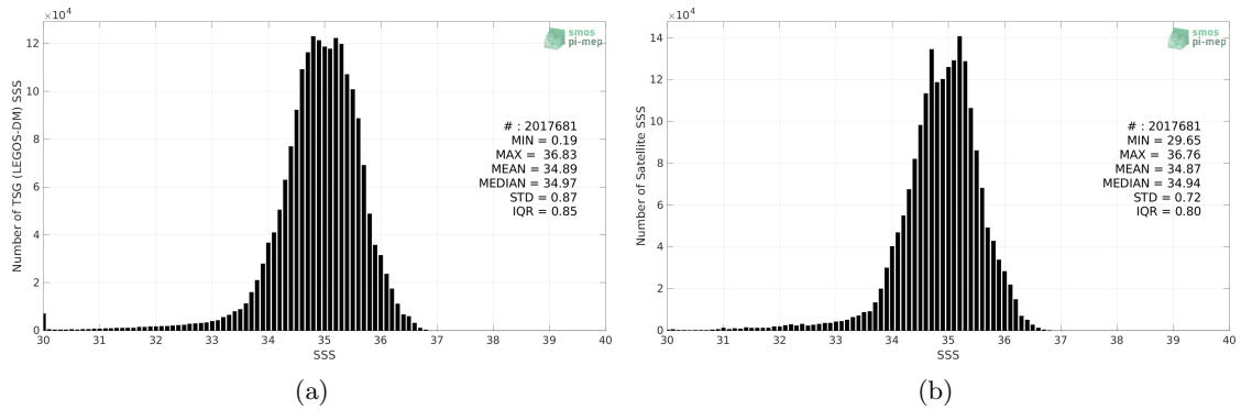
Figure 2: Histograms of SSS from TSG (LEGOS-DM) (a) and SMOS SSS L4 v1 - Weekly (CMEMS-CNR) (b) considering all match-up pairs per bins of 0.1 over the Pacific Ocean Pi-MEP region and for the full satellite product period.
