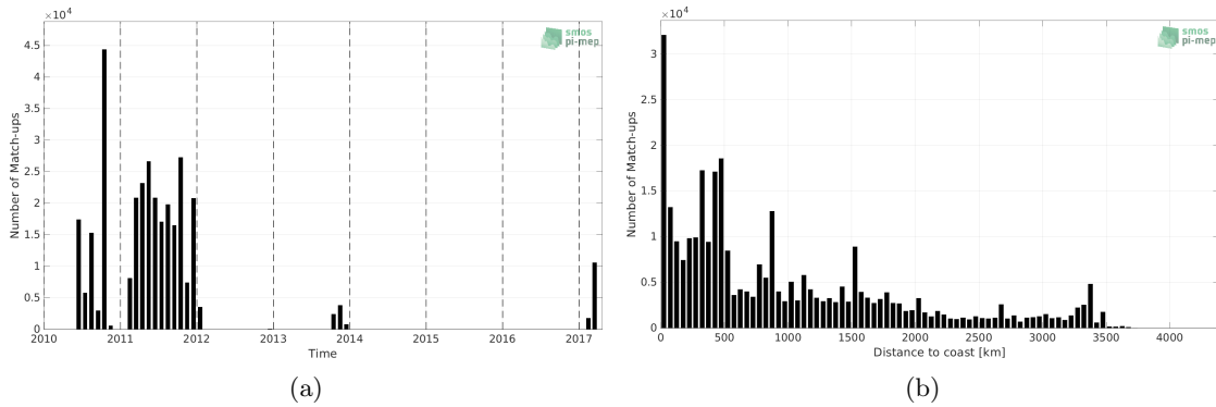
Figure 1: Number of match-ups between TSG (GOSUD-Sailing-ship) and SMOS SSS L4 v1 - Weekly (CMEMS-CNR) SSS as a function of time (a) and as function of the distance to coast (b) over the Pacific Ocean Pi-MEP region and for the full satellite product period.
