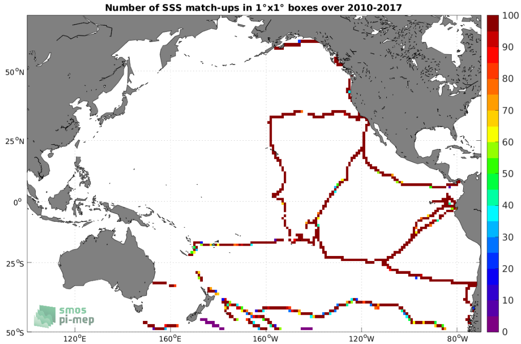
Figure 4: Number of SSS match-ups between TSG (GOSUD-Sailing-ship) SSS and the SMOS SSS L4 v1 - Weekly (CMEMS-CNR) SSS product for the Pacific Ocean Pi-MEP region over 1^\circ \times 1^\circ boxes and for the full satellite product period.
