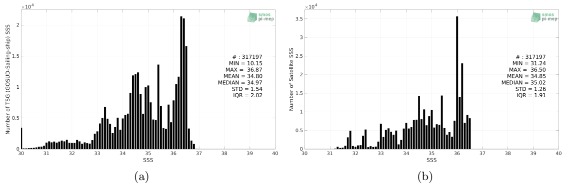
Figure 2: Histograms of SSS from TSG (GOSUD-Sailing-ship) (a) and SMOS SSS L4 v1 - Weekly (CMEMS-CNR) (b) considering all match-up pairs per bins of 0.1 over the Pacific Ocean Pi-MEP region and for the full satellite product period.
