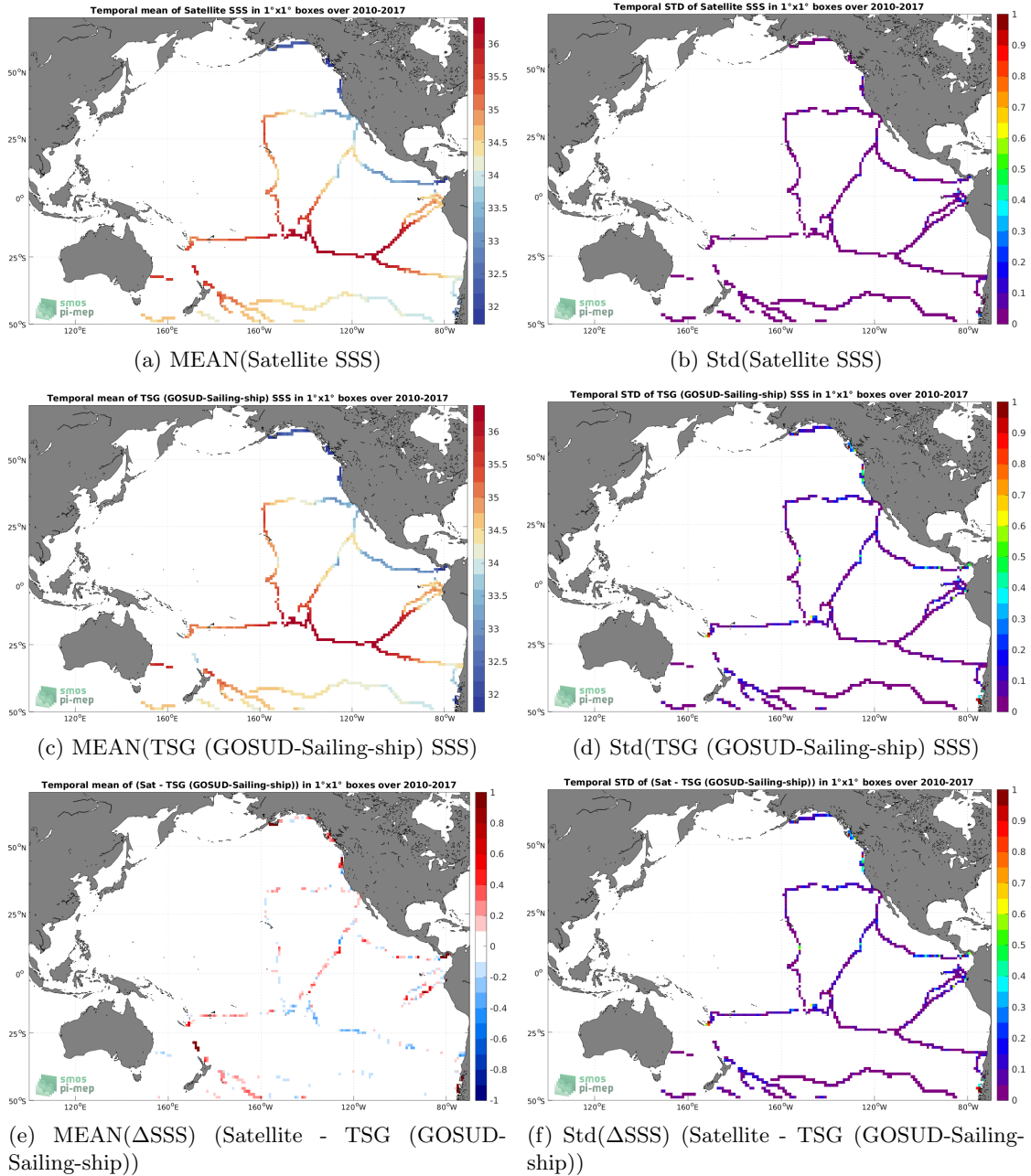
Figure 6: Temporal mean (left) and Std (right) of SSS from SMOS SSS L4 v1 - Weekly (CMEMS-CNR) (top), TSG (GOSUD-Sailing-ship) (middle), and of \Delta SSS (Satellite - TSG (GOSUD-Sailing-ship)). Only match-up pairs are used to generate these maps.
