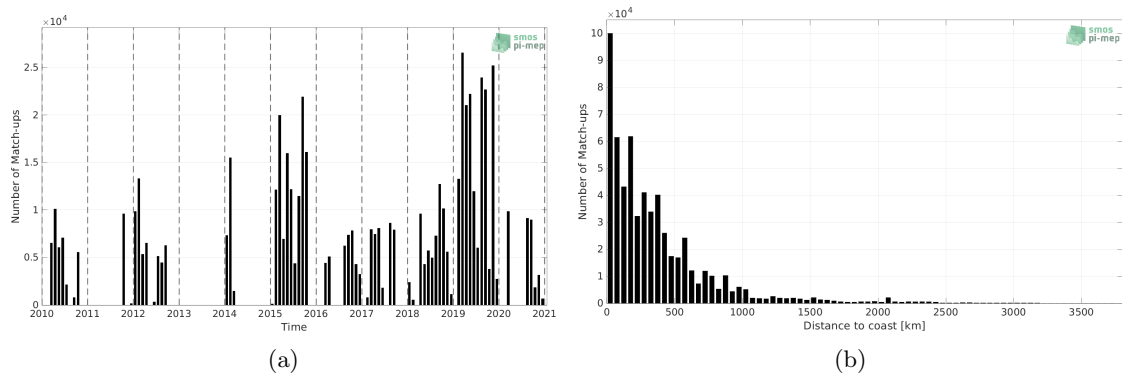
Figure 1: Number of match-ups between TSG (GOSUD-Research-vessel) and SMOS SSS L4 v1 - Weekly (CMEMS-CNR) SSS as a function of time (a) and as function of the distance to coast (b) over the Pacific Ocean Pi-MEP region and for the full satellite product period.
