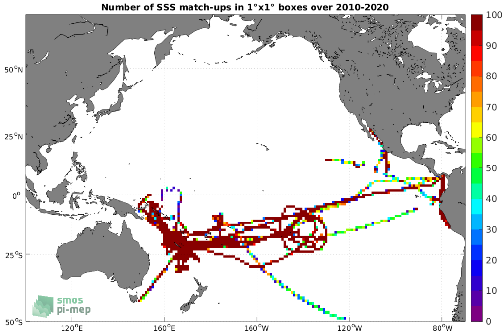
Figure 4: Number of SSS match-ups between TSG (GOSUD-Research-vessel) SSS and the SMOS SSS L4 v1 - Weekly (CMEMS-CNR) SSS product for the Pacific Ocean Pi-MEP region over 1^\circ \times 1^\circ boxes and for the full satellite product period.
