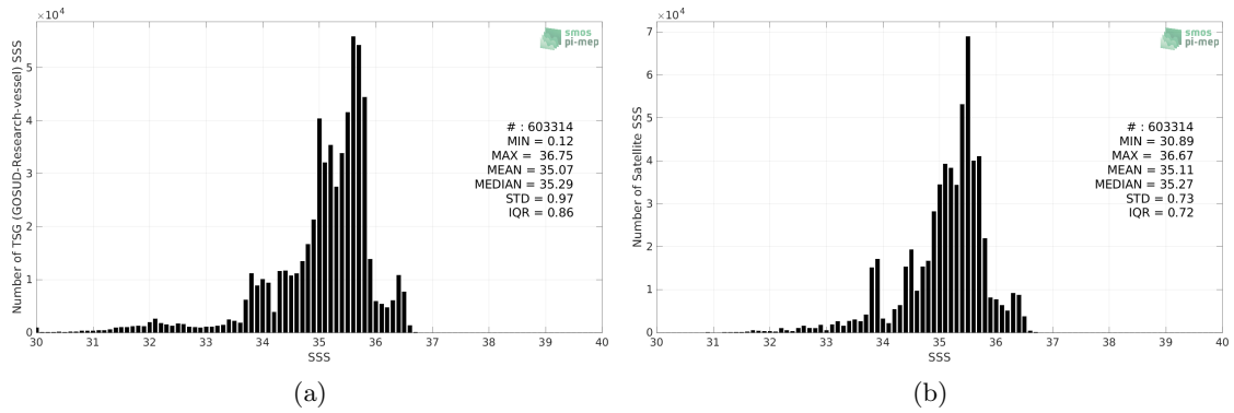
Figure 2: Histograms of SSS from TSG (GOSUD-Research-vessel) (a) and SMOS SSS L4 v1 - Weekly (CMEMS-CNR) (b) considering all match-up pairs per bins of 0.1 over the Pacific Ocean Pi-MEP region and for the full satellite product period.
