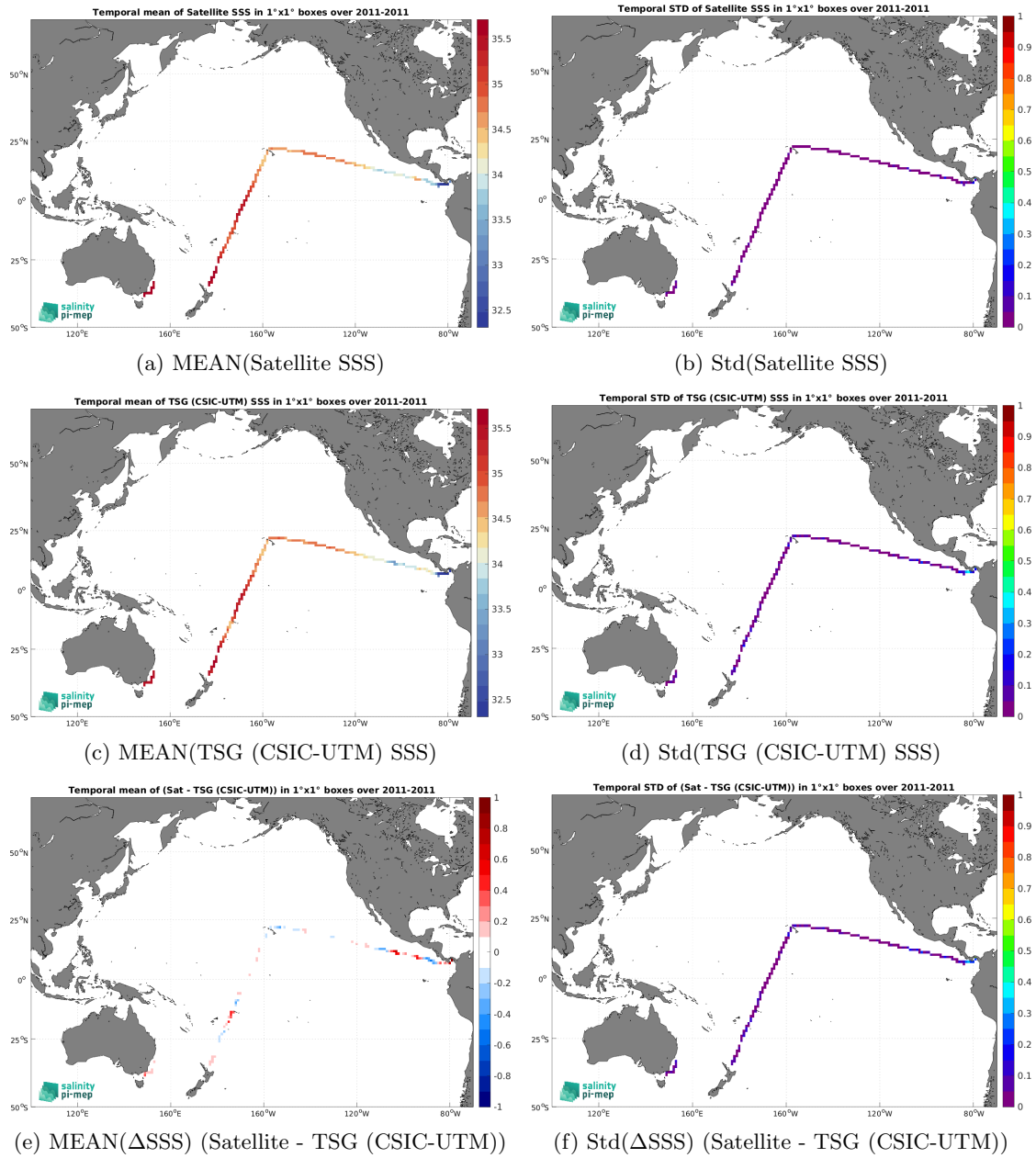
Figure 6: Temporal mean (left) and Std (right) of SSS from SMOS SSS L4 v1 - Weekly (CMEMS-CNR) (top), TSG (CSIC-UTM) (middle), and of \Delta SSS (Satellite - TSG (CSIC-UTM)). Only match-up pairs are used to generate these maps.
