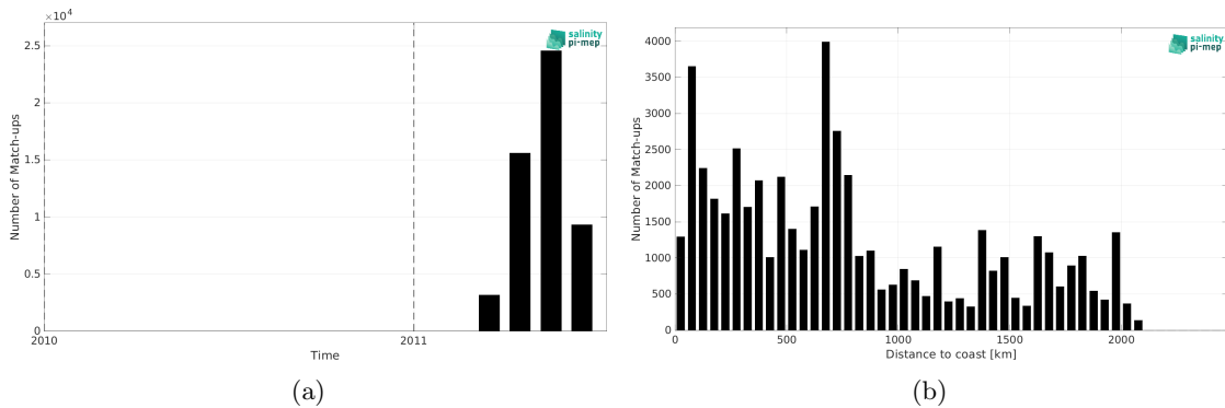
Figure 1: Number of match-ups between TSG (CSIC-UTM) and SMOS SSS L4 v1 - Weekly (CMEMS-CNR) SSS as a function of time (a) and as function of the distance to coast (b) over the Pacific Ocean Pi-MEP region and for the full satellite product period.
