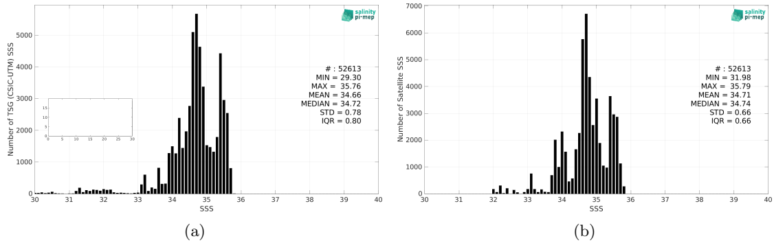
Figure 2: Histograms of SSS from TSG (CSIC-UTM) (a) and SMOS SSS L4 v1 - Weekly (CMEMS-CNR) (b) considering all match-up pairs per bins of 0.1 over the Pacific Ocean Pi-MEP region and for the full satellite product period.
