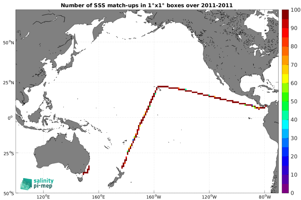
Figure 4: Number of SSS match-ups between TSG (CSIC-UTM) SSS and the SMOS SSS L4 v1 - Weekly (CMEMS-CNR) SSS product for the Pacific Ocean Pi-MEP region over 1^{\circ} \times 1^{\circ} boxes and for the full satellite product period.
