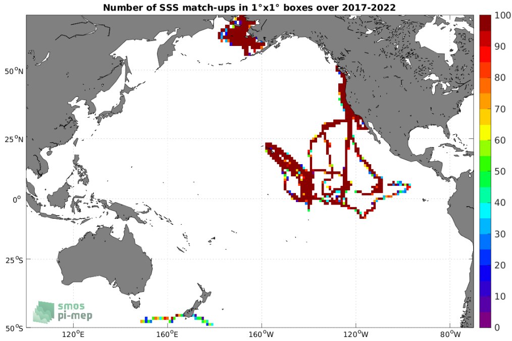
Figure 4: Number of SSS match-ups between Saildrone SSS and the SMOS SSS L4 v1 - Weekly (CMEMS-CNR) SSS product for the Pacific Ocean Pi-MEP region over 1^\circ \times 1^\circ boxes and for the full satellite product period.
