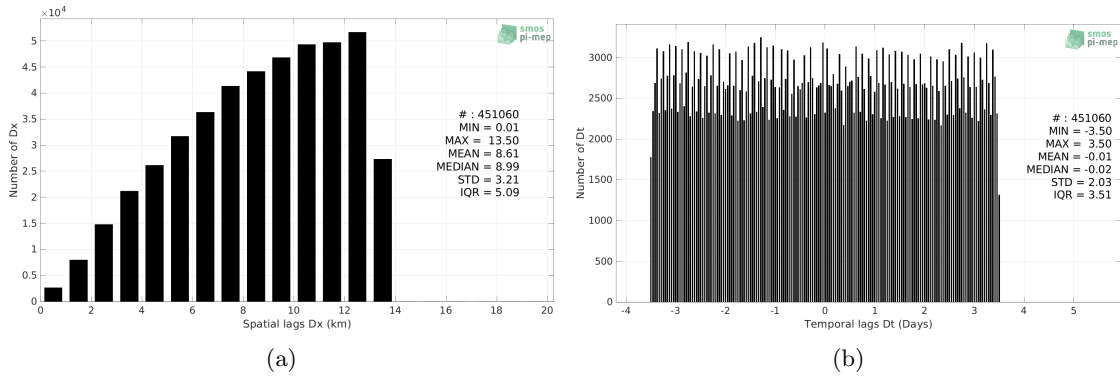
Figure 5: Histograms of the spatial (a) and temporal (b) lags between the location/time of the Saildrone measurement and the date of the corresponding SMOS SSS L4 v1 - Weekly (CMEMS-CNR) SSS pixel.
