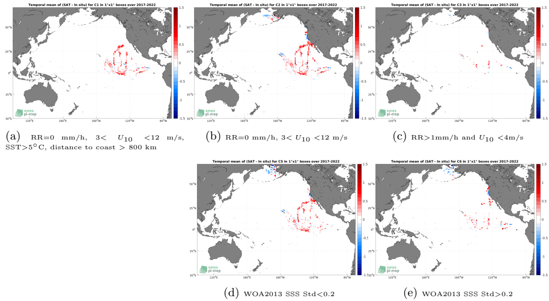
Figure 12: Temporal mean gridded over spatial boxes of size 1^\circ \times 1^\circ of \Delta SSS (SMOS SSS L4 v1 - Weekly (CMEMS-CNR) - Saifdrone) for 5 different subdatasets corresponding to:RR=0 mm/h, 3 < U_{10} < 12 m/s, SST >5^\circ\text{C} , distance to coast > 800 km (a), RR=0 mm/h, 3 < U_{10} < 12 m/s (b), RR >1 mm/h and U_{10} < 4 m/s (c), WOA2013 SSS Std <0.2 (d), WOA2013 SSS Std >0.2 (e).
