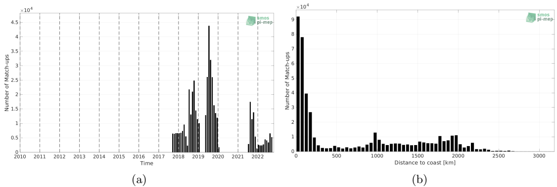
Figure 1: Number of match-ups between Saildrone and SMOS SSS L4 v1 - Weekly (CMEMS-CNR) SSS as a function of time (a) and as function of the distance to coast (b) over the Pacific Ocean Pi-MEP region and for the full satellite product period.
