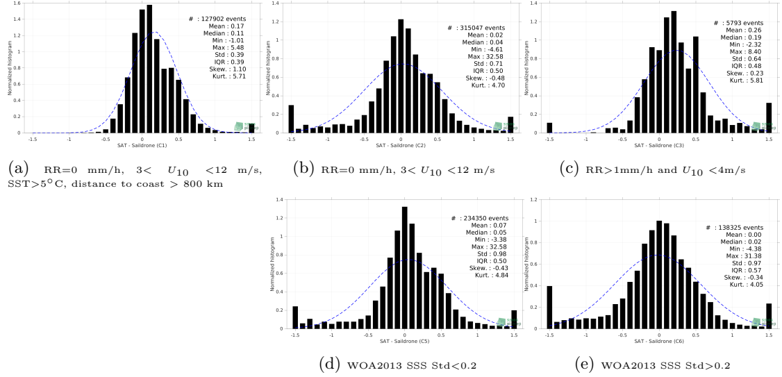
Figure 13: Normalized histogram of \Delta SSS (SMOS SSS L4 v1 - Weekly (CMEMS-CNR) - Saildrone) for 5 different subdatasets corresponding to: RR=0 mm/h, 3 < U_{10} < 12 m/s, SST>5°C, distance to coast > 800 km (a), RR=0 mm/h, 3 < U_{10} < 12 m/s (b), RR>1mm/h and U_{10} < 4 m/s (c), WOA2013 SSS Std<0.2 (d), WOA2013 SSS Std>0.2 (e).
