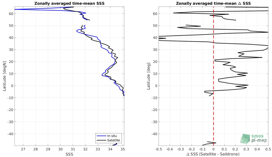
Figure 8: Left panel: Zonal mean SSS from SMOS SSS L4 v1 - Weekly (CMEMS-CNR) satellite product (black) and from Sairdrone (blue). Right panel: Zonal mean of \Delta SSS (Satellite - Sairdrone) for all the collected Pi-MEP match-up pairs estimated over the full satellite product period.
