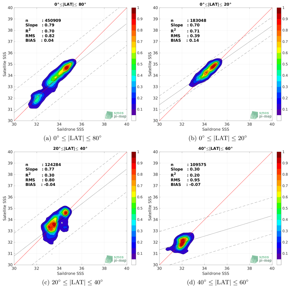
Figure 9: Contour maps of the concentration of SMOS SSS L4 v1 - Weekly (CMEMS-CNR) SSS (y-axis) versus Saildrone SSS (x-axis) at match-up pairs for different latitude bands. For each plot, the red line shows x=y . The black thin and dashed lines indicate a linear fit through the data cloud and the \pm 95\% confidence levels, respectively. The number match-up pairs n , the slope and R^2 coefficient of the linear fit, the root mean square (RMS) and the mean bias between satellite and in situ data are indicated for each latitude band in each plots.
