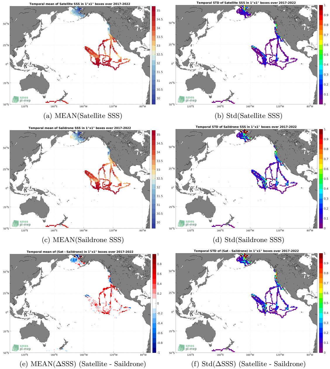
Figure 6: Temporal mean (left) and Std (right) of SSS from SMOS SSS L4 v1 - Weekly (CMEMS-CNR) (top), Saildrone (middle), and of \Delta SSS (Satellite - Saildrone). Only match-up pairs are used to generate these maps.
