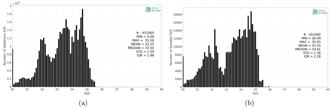
Figure 2: Histograms of SSS from Saildrone (a) and SMOS SSS L4 v1 - Weekly (CMEMS-CNR) (b) considering all match-up pairs per bins of 0.1 over the Pacific Ocean Pi-MEP region and for the full satellite product period.
