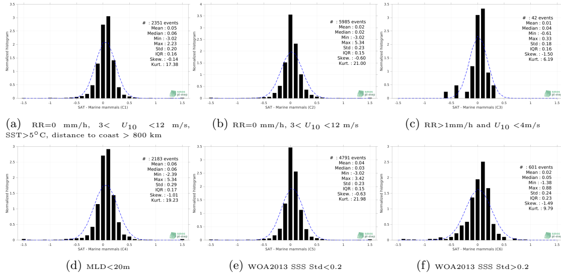
Figure 13: Normalized histogram of \Delta\text{SSS} (SMOS SSS L4 v1 - Weekly (CMEMS-CNR) - Marine mammals) for 6 different subdatasets corresponding to: RR=0 mm/h, 3 < U_{10} < 12 m/s, SST>5°C, distance to coast > 800 km (a), RR=0 mm/h, 3 < U_{10} < 12 m/s (b), RR>1mm/h and U_{10} < 4 m/s (c), MLD<20m (d), WOA2013 SSS Std<0.2 (e), WOA2013 SSS Std>0.2 (f).
