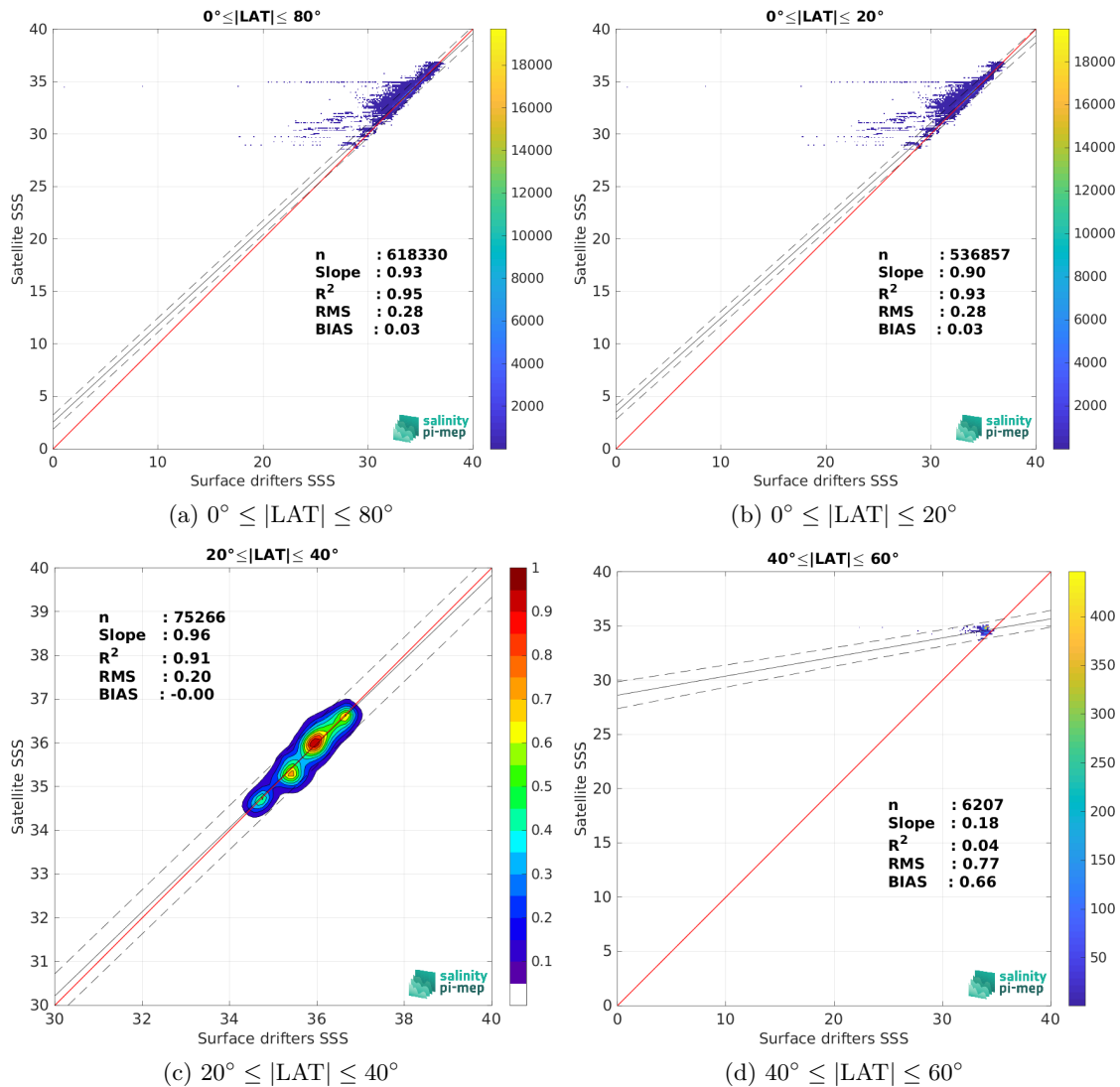
Figure 8: Contour maps of the concentration of SMOS SSS L4 v1 - Weekly (CMEMS-CNR) SSS (y-axis) versus Surface drifters SSS (x-axis) at match-up pairs for different latitude bands. For each plot, the red line shows x=y . The black thin and dashed lines indicate a linear fit through the data cloud and the \pm 95\% confidence levels, respectively. The number match-up pairs n , the slope and R^2 coefficient of the linear fit, the root mean square (RMS) and the mean bias between satellite and in situ data are indicated for each latitude band in each plots.
