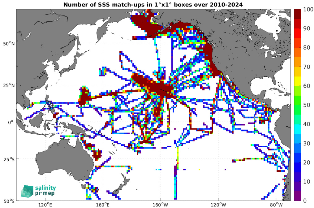
Figure 5: Number of SSS match-ups between TSG (SAMOS) SSS and the SMOS SSS L4 v1 - Monthly (CMEMS-CNR) SSS product for the Pacific Ocean Pi-MEP region over 1^\circ \times 1^\circ boxes and for the full satellite product period.
