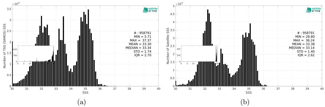
Figure 3: Histograms of SSS from TSG (SAMOS) (a) and SMOS SSS L4 v1 - Monthly (CMEMS-CNR) (b) considering all match-up pairs per bins of 0.1 over the Pacific Ocean Pi-MEP region and for the full satellite product period.
