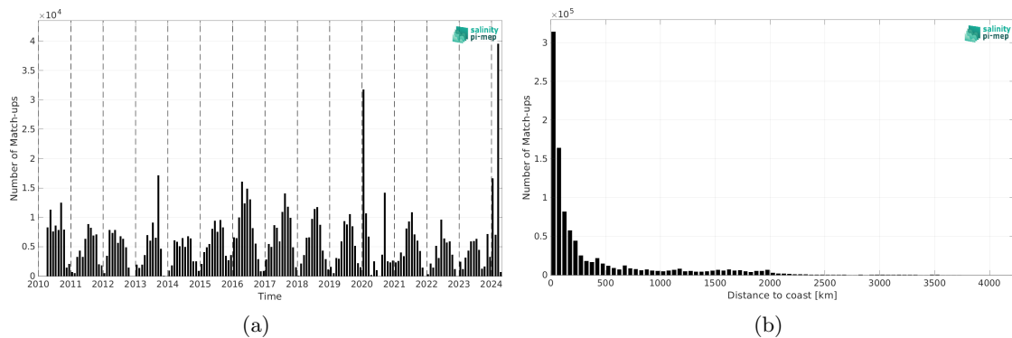
Figure 2: Number of match-ups between TSG (SAMOS) and SMOS SSS L4 v1 - Monthly (CMEMS-CNR) SSS as a function of time (a) and as function of the distance to coast (b) over the Pacific Ocean Pi-MEP region and for the full satellite product period.
