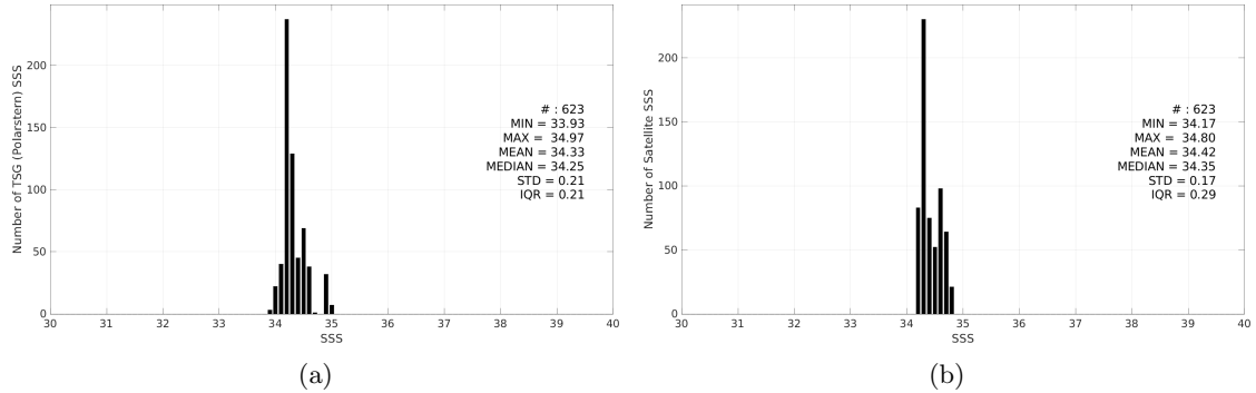
Figure 3: Histograms of SSS from TSG (Polarstern) (a) and SMOS SSS L4 v1 - Monthly (CMEMS-CNR) (b) considering all match-up pairs per bins of 0.1 over the Pacific Ocean Pi-MEP region and for the full satellite product period.
