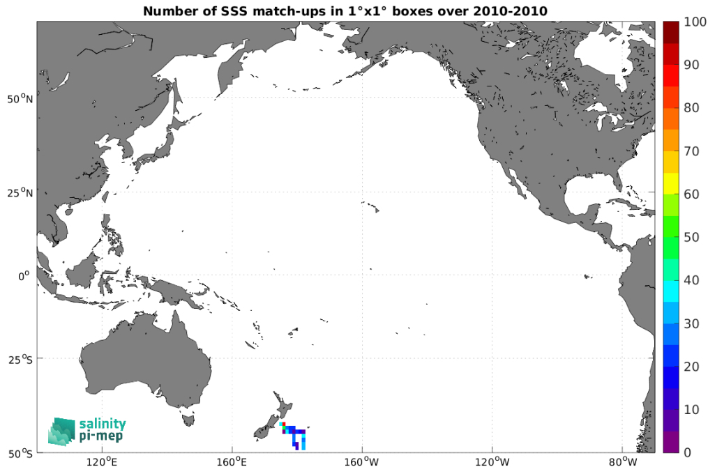
Figure 5: Number of SSS match-ups between TSG (Polarstern) SSS and the SMOS SSS L4 v1 - Monthly (CMEMS-CNR) SSS product for the Pacific Ocean Pi-MEP region over 1^\circ \times 1^\circ boxes and for the full satellite product period.
