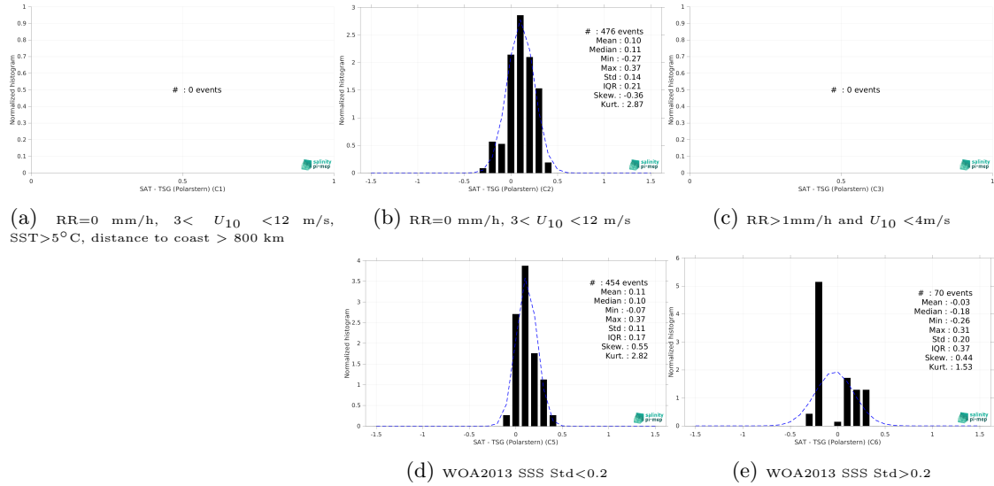
Figure 15: Normalized histogram of \Delta SSS (SMOS SSS L4 v1 - Monthly (CMEMS-CNR) - TSG (Polarstern)) for 5 different subdatasets corresponding to: RR=0 mm/h, 3 < U_{10} < 12 m/s, SST > 5°C, distance to coast > 800 km (a), RR=0 mm/h, 3 < U_{10} < 12 m/s (b), RR > 1mm/h and U_{10} < 4 m/s (c), WOA2013 SSS Std < 0.2 (d), WOA2013 SSS Std > 0.2 (e).
