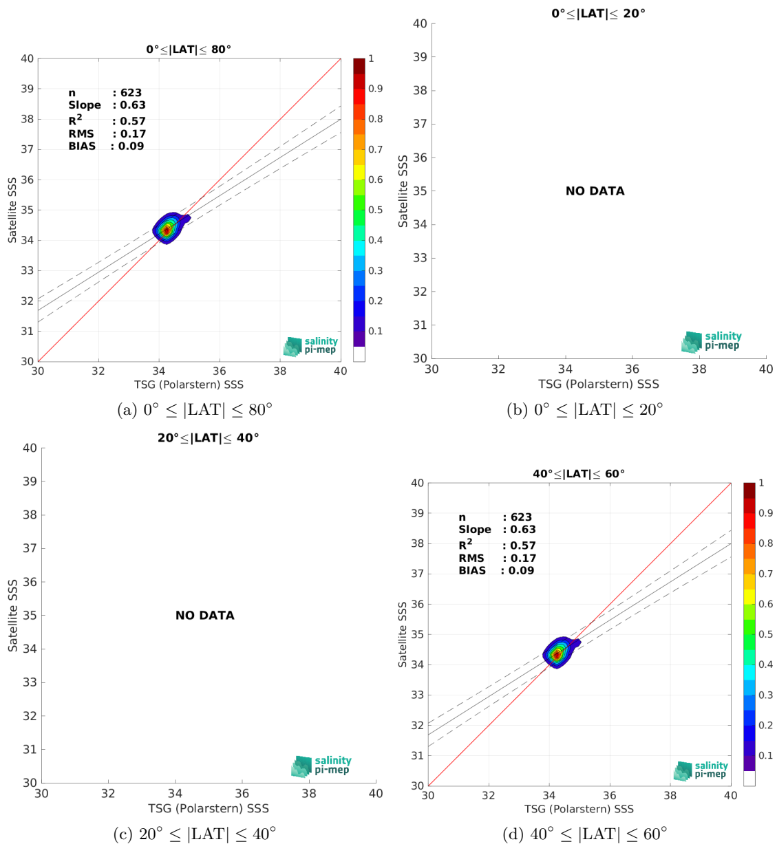
Figure 10: Contour maps of the concentration of SMOS SSS L4 v1 - Monthly (CMEMS-CNR) SSS (y-axis) versus TSG (Polarstern) SSS (x-axis) at match-up pairs for different latitude bands. For each plot, the red line shows x=y . The black thin and dashed lines indicate a linear fit through the data cloud and the \pm 95\% confidence levels, respectively. The number match-up pairs n , the slope and R^2 coefficient of the linear fit, the root mean square (RMS) and the mean bias between satellite and in situ data are indicated for each latitude band in each plot.
