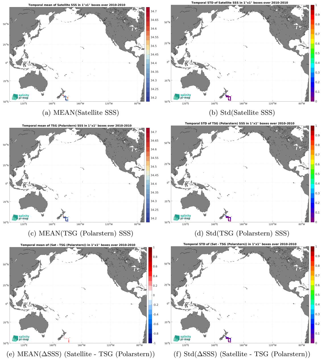
Figure 7: Temporal mean (left) and Std (right) of SSS from SMOS SSS L4 v1 - Monthly (CMEMS-CNR) (top), TSG (Polarstern) (middle), and of \Delta SSS (Satellite - TSG (Polarstern)). Only match-up pairs are used to generate these maps.
