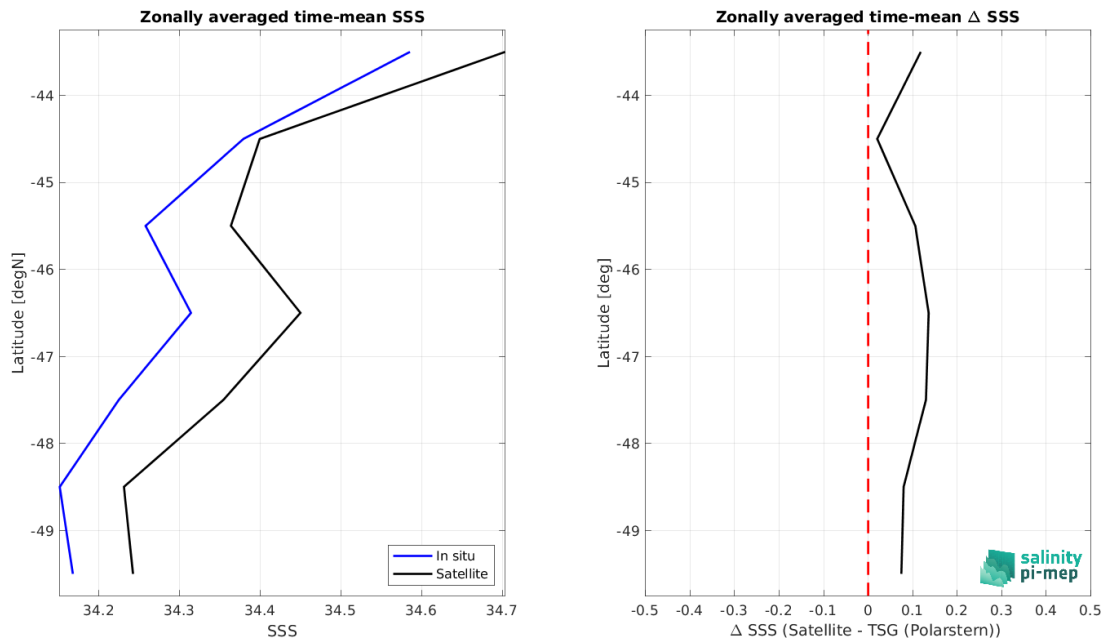
Figure 9: Left panel: Zonal mean SSS from SMOS SSS L4 v1 - Monthly (CMEMS-CNR) satellite product (black) and from TSG (Polarstern) (blue). Right panel: Zonal mean of \Delta SSS (Satellite - TSG (Polarstern)) for all the collected Pi-MEP match-up pairs estimated over the full satellite product period.
