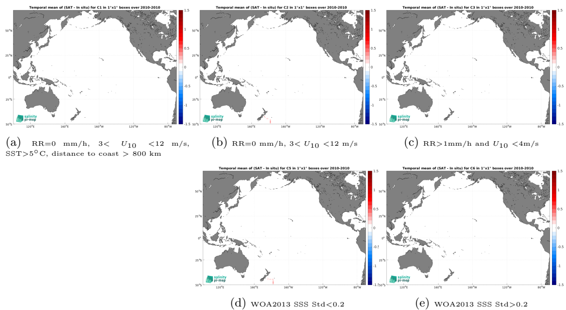
Figure 14: Temporal mean gridded over spatial boxes of size 1^\circ \times 1^\circ of \Delta SSS (SMOS SSS L4 v1 - Monthly (CMEMS-CNR) - TSG (Polarstern)) for 5 different subdatasets corresponding to:RR=0 mm/h, 3 < U_{10} < 12 m/s, SST >5^\circ\text{C} , distance to coast > 800 km (a), RR=0 mm/h, 3 < U_{10} < 12 m/s (b), RR >1 mm/h and U_{10} < 4 m/s (c), WOA2013 SSS Std <0.2 (d), WOA2013 SSS Std >0.2 (e).
