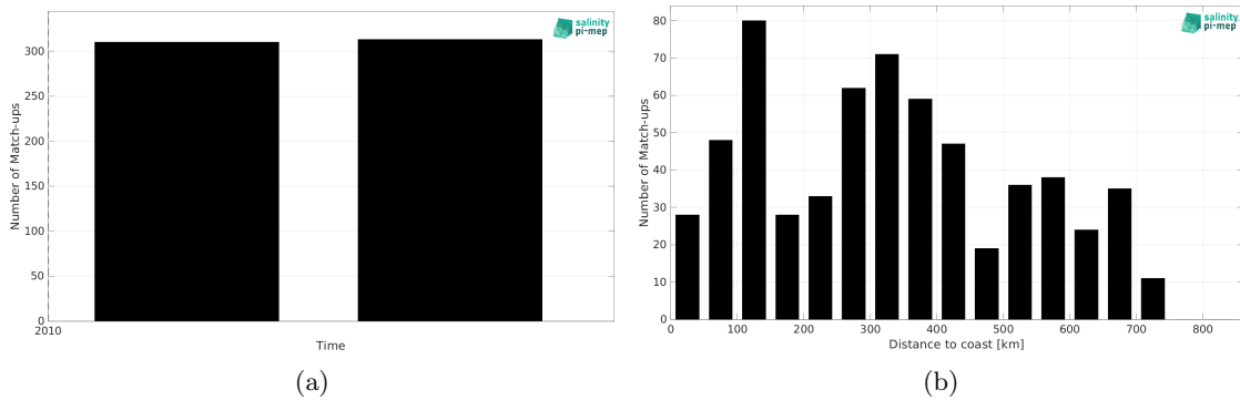
Figure 2: Number of match-ups between TSG (Polarstern) and SMOS SSS L4 v1 - Monthly (CMEMS-CNR) SSS as a function of time (a) and as function of the distance to coast (b) over the Pacific Ocean Pi-MEP region and for the full satellite product period.
