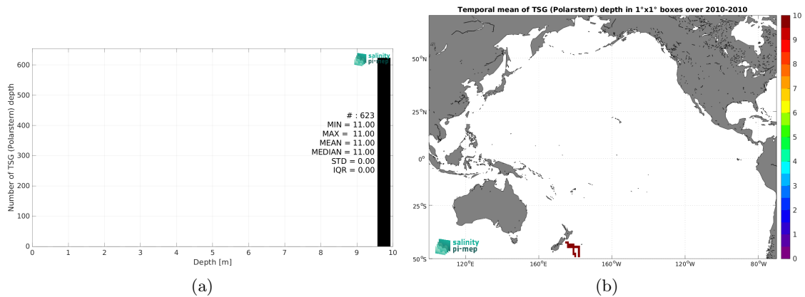
Figure 4: Histograms of the depth of the upper level SSS measurements from TSG (Polarstern) in the Match-up DataBase for the Pacific Ocean Pi-MEP region (a) and temporal mean spatial distribution of pressure of the in situ SSS data over 1^\circ \times 1^\circ boxes and for the full satellite product period (b).
