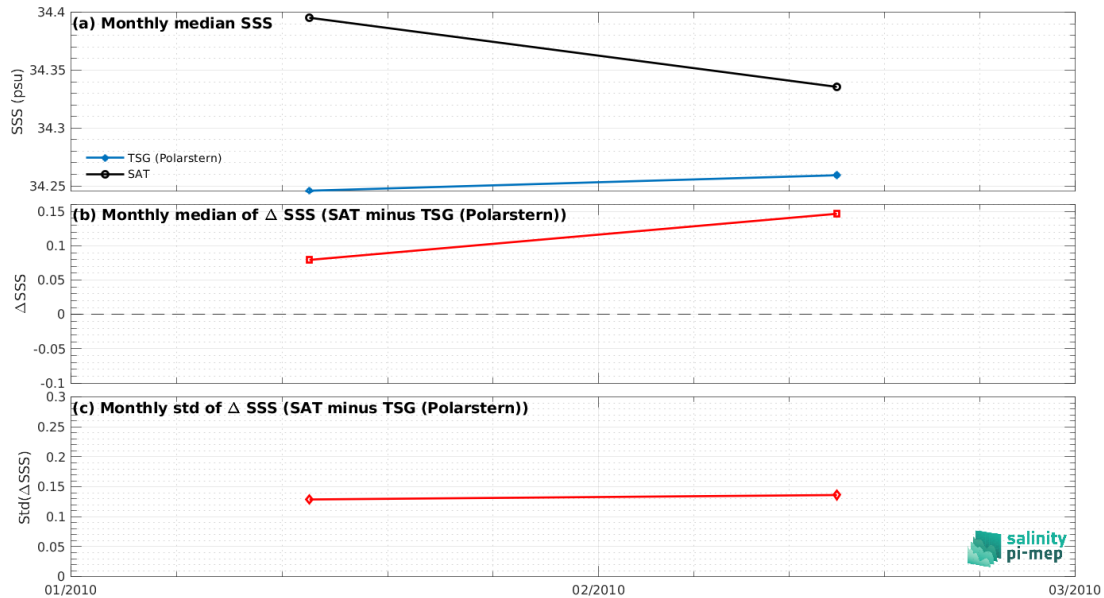
Figure 8: Time series of the monthly median SSS (top), median of \Delta SSS (Satellite - TSG (Polarstern)) and Std of \Delta SSS (Satellite - TSG (Polarstern)) over the Pacific Ocean Pi-MEP region considering all match-ups collected by the Pi-MEP.
