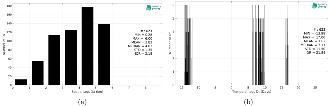
Figure 6: Histograms of the spatial (a) and temporal (b) lags between the location/time of the TSG (Polarstern) measurement and the date of the corresponding SMOS SSS L4 v1 - Monthly (CMEMS-CNR) SSS pixel.
