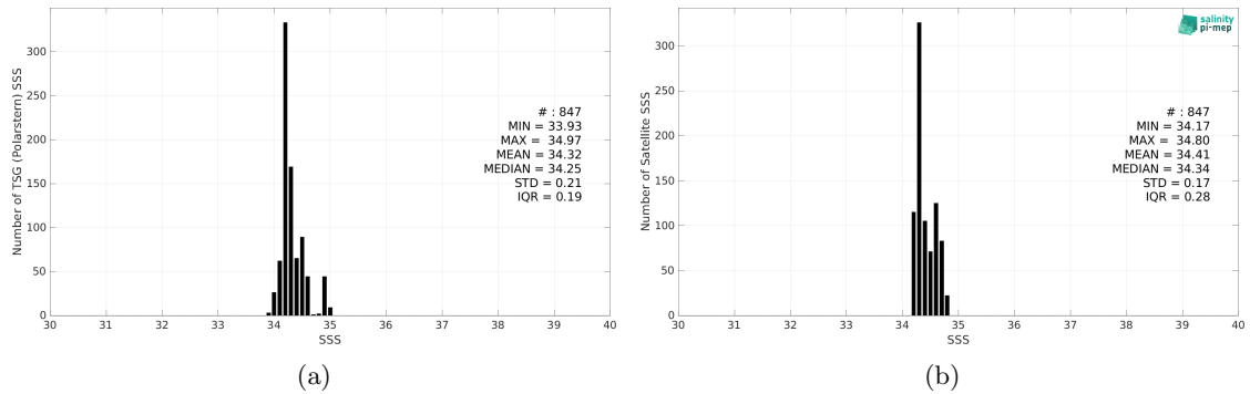
Figure 2: Histograms of SSS from TSG (Polarstern) (a) and SMOS SSS L4 v1 - Monthly (CMEMS-CNR) (b) considering all match-up pairs per bins of 0.1 over the Pacific Ocean Pi-MEP region and for the full satellite product period.
