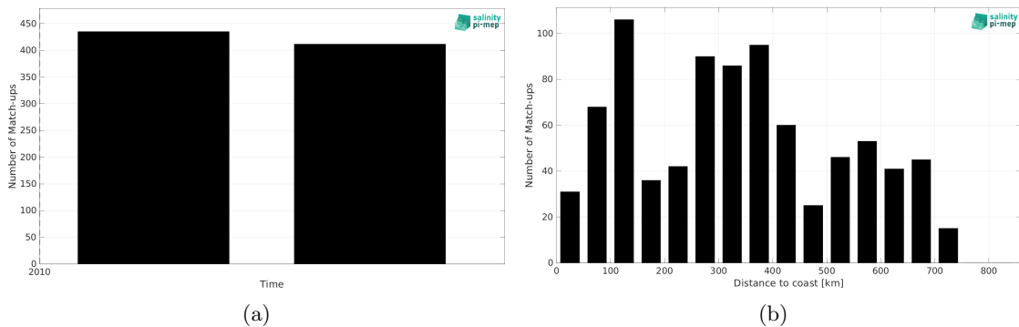
Figure 1: Number of match-ups between TSG (Polarstern) and SMOS SSS L4 v1 - Monthly (CMEMS-CNR) SSS as a function of time (a) and as function of the distance to coast (b) over the Pacific Ocean Pi-MEP region and for the full satellite product period.
