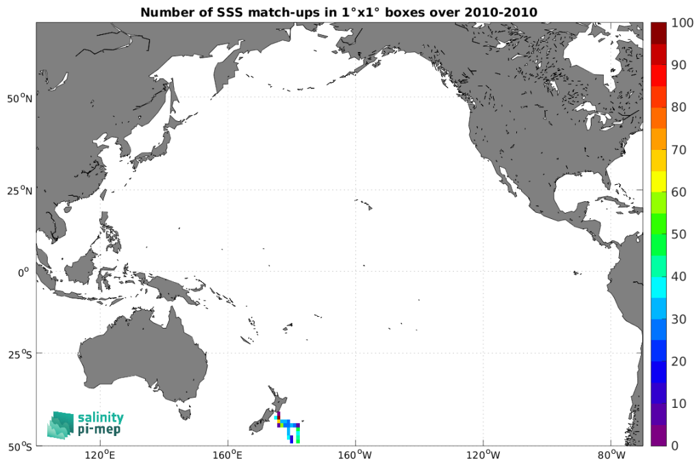
Figure 4: Number of SSS match-ups between TSG (Polarstern) SSS and the SMOS SSS L4 v1 - Monthly (CMEMS-CNR) SSS product for the Pacific Ocean Pi-MEP region over 1^\circ \times 1^\circ boxes and for the full satellite product period.
