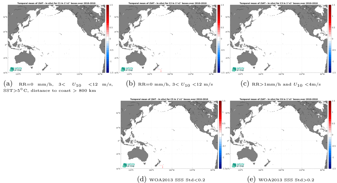
Figure 12: Temporal mean gridded over spatial boxes of size 1^{\circ}\times 1^{\circ} of \Delta\text{SSS} (SMOS SSS L4 v1 - Monthly (CMEMS-CNR) - TSG (Polarstern)) for 5 different subdatasets corresponding to:RR=0 mm/h, 3 < U_{10} < 12 m/s, SST >5^{\circ}\text{C} , distance to coast > 800 km (a), RR=0 mm/h, 3 < U_{10} < 12 m/s (b), RR >1 mm/h and U_{10} < 4 m/s (c), WOA2013 SSS Std <0.2 (d), WOA2013 SSS Std >0.2 (e).
