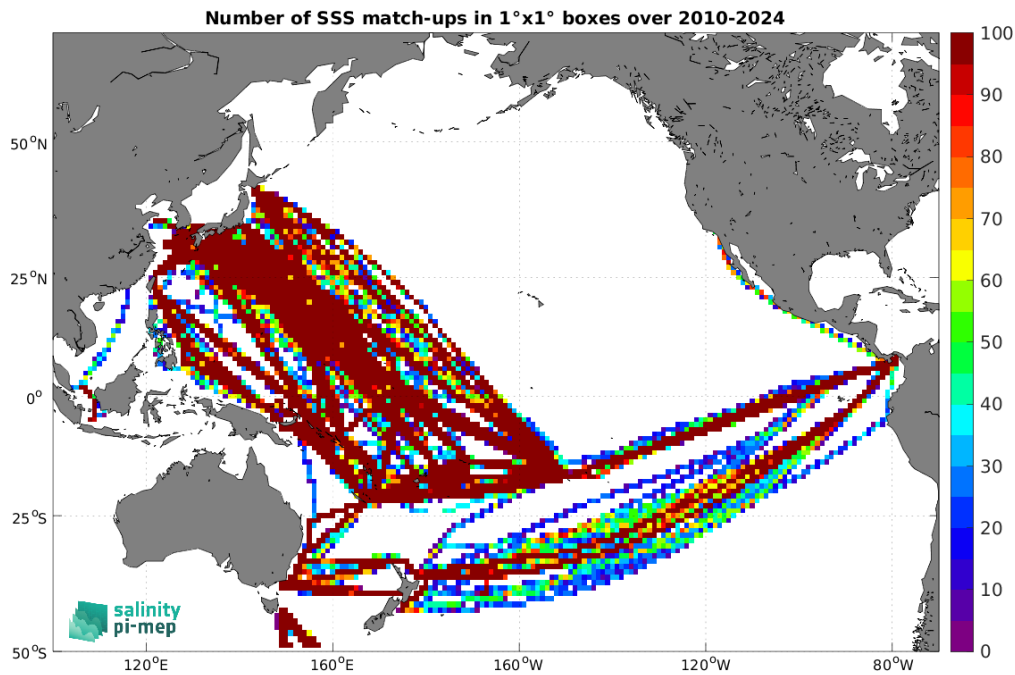
Figure 5: Number of SSS match-ups between TSG (LEGOS-DM) SSS and the SMOS SSS L4 v1 - Monthly (CMEMS-CNR) SSS product for the Pacific Ocean Pi-MEP region over 1^{\circ} \times 1^{\circ} boxes and for the full satellite product period.
