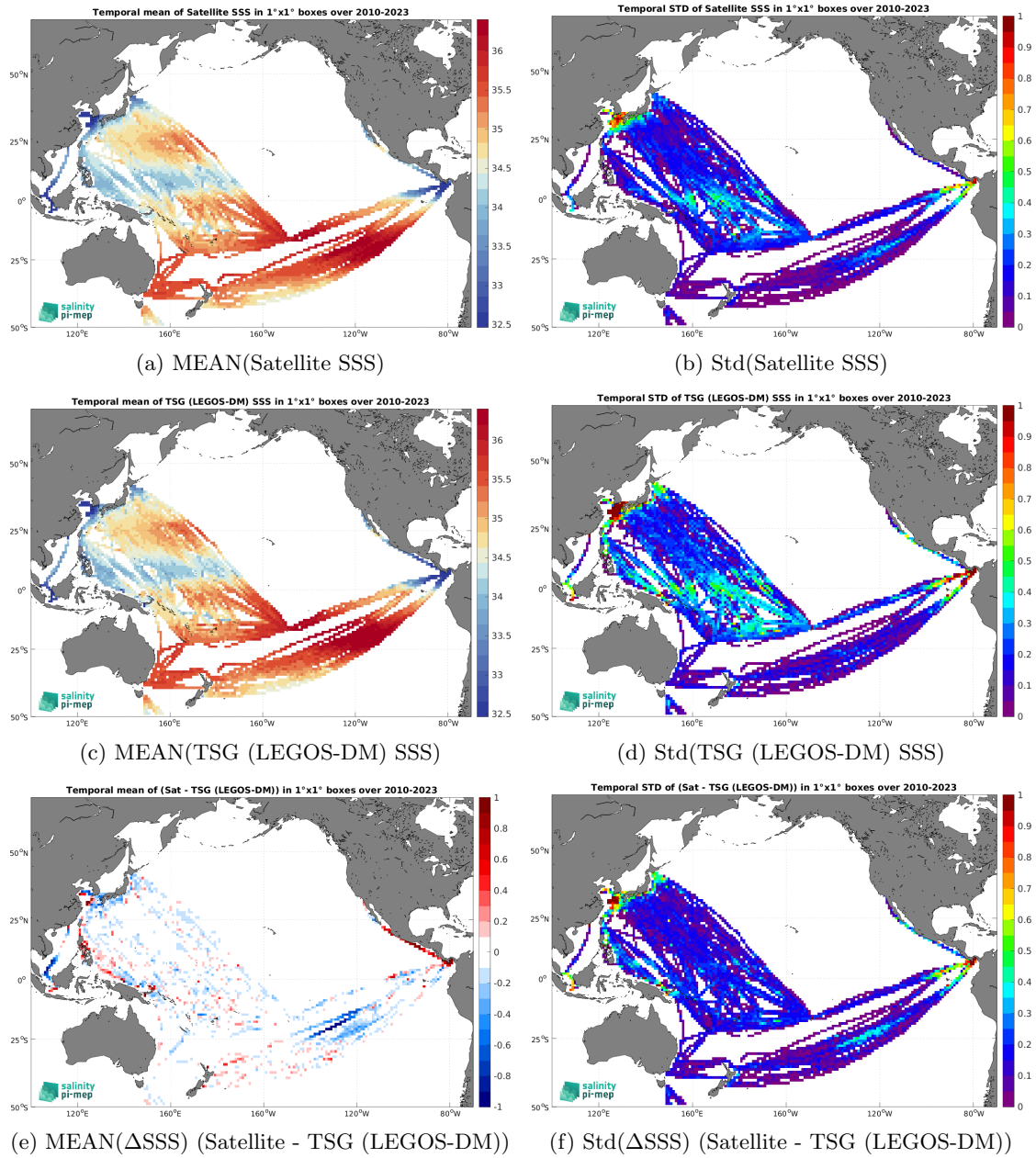
Figure 7: Temporal mean (left) and Std (right) of SSS from SMOS SSS L4 v1 - Monthly (CMEMS-CNR) (top), TSG (LEGOS-DM) (middle), and of \Delta SSS (Satellite - TSG (LEGOS-DM)). Only match-up pairs are used to generate these maps.
