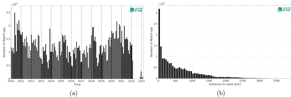
Figure 2: Number of match-ups between TSG (LEGOS-DM) and SMOS SSS L4 v1 - Monthly (CMEMS-CNR) SSS as a function of time (a) and as function of the distance to coast (b) over the Pacific Ocean Pi-MEP region and for the full satellite product period.
