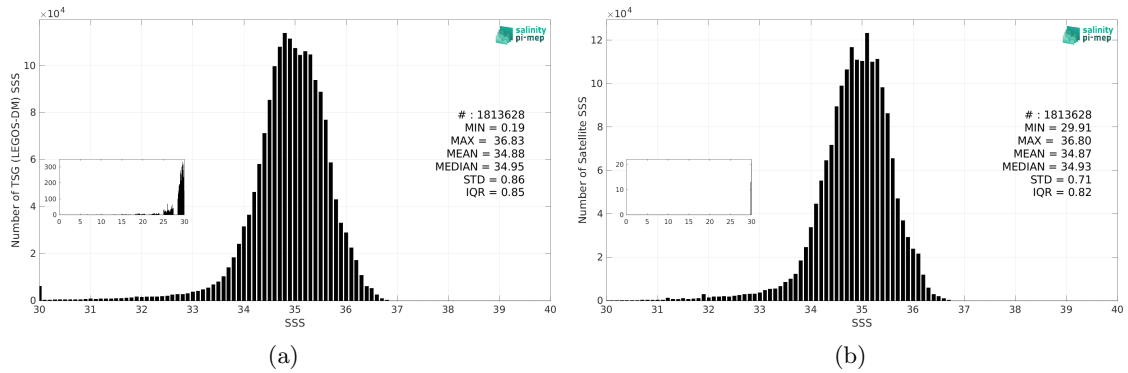
Figure 3: Histograms of SSS from TSG (LEGOS-DM) (a) and SMOS SSS L4 v1 - Monthly (CMEMS-CNR) (b) considering all match-up pairs per bins of 0.1 over the Pacific Ocean Pi-MEP region and for the full satellite product period.
