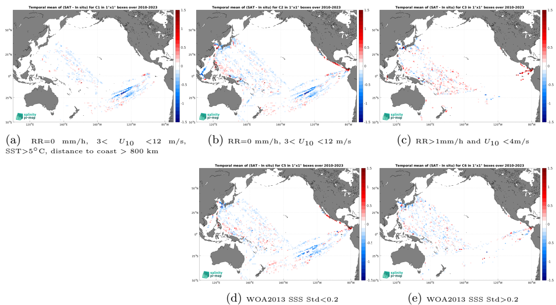
Figure 14: Temporal mean gridded over spatial boxes of size 1^\circ \times 1^\circ of \Delta SSS (SMOS SSS L4 v1 - Monthly (CMEMS-CNR) - TSG (LEGOS-DM)) for 5 different subdatasets corresponding to:RR=0 mm/h, 3 < U_{10} < 12 m/s, SST >5^\circ\text{C} , distance to coast > 800 km (a), RR=0 mm/h, 3 < U_{10} < 12 m/s (b), RR >1 mm/h and U_{10} < 4 m/s (c), WOA2013 SSS Std <0.2 (d), WOA2013 SSS Std >0.2 (e).
