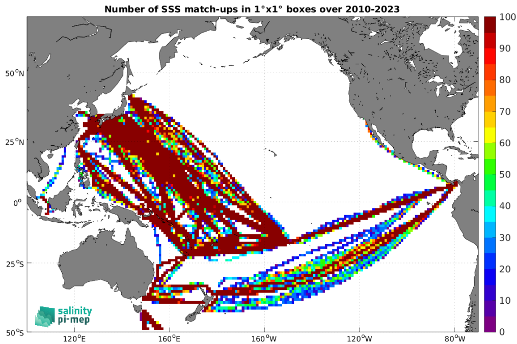
Figure 5: Number of SSS match-ups between TSG (LEGOS-DM) SSS and the SMOS SSS L4 v1 - Monthly (CMEMS-CNR) SSS product for the Pacific Ocean Pi-MEP region over 1^\circ \times 1^\circ boxes and for the full satellite product period.
