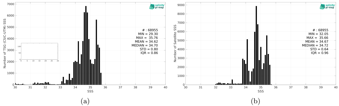
Figure 2: Histograms of SSS from TSG (CSIC-UTM) (a) and SMOS SSS L4 v1 - Monthly (CMEMS-CNR) (b) considering all match-up pairs per bins of 0.1 over the Pacific Ocean Pi-MEP region and for the full satellite product period.
