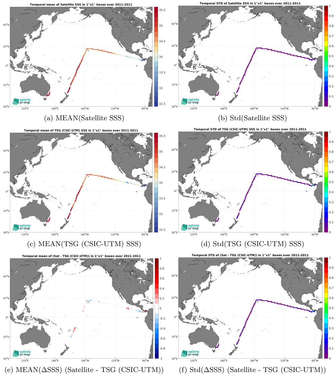
Figure 6: Temporal mean (left) and Std (right) of SSS from SMOS SSS L4 v1 - Monthly (CMEMS-CNR) (top), TSG (CSIC-UTM) (middle), and of \Delta SSS (Satellite - TSG (CSIC-UTM)). Only match-up pairs are used to generate these maps.
