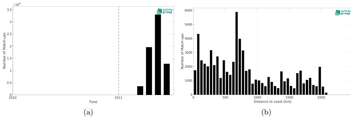
Figure 1: Number of match-ups between TSG (CSIC-UTM) and SMOS SSS L4 v1 - Monthly (CMEMS-CNR) SSS as a function of time (a) and as function of the distance to coast (b) over the Pacific Ocean Pi-MEP region and for the full satellite product period.
