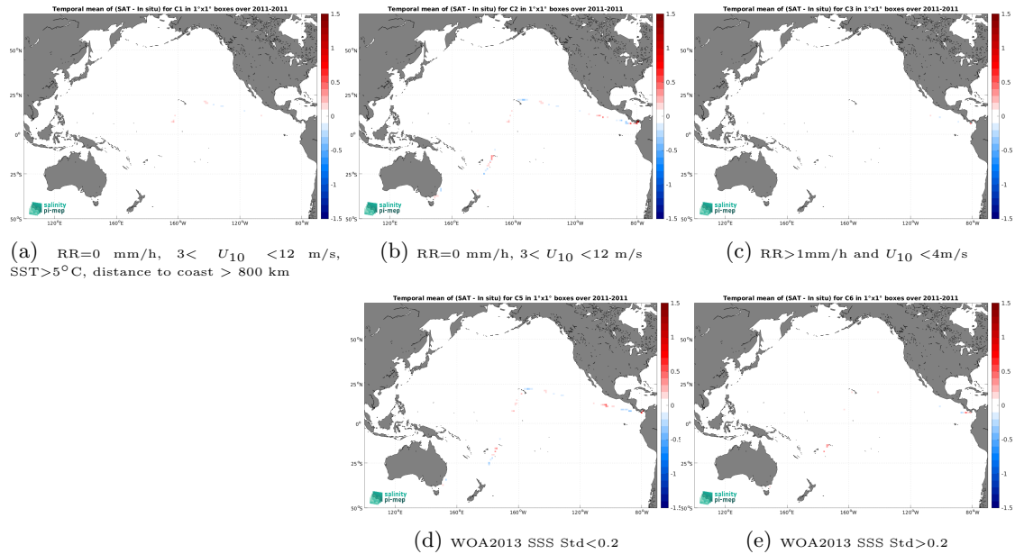
Figure 12: Temporal mean gridded over spatial boxes of size 1^\circ \times 1^\circ of \Delta SSS (SMOS SSS L4 v1 - Monthly (CMEMS-CNR) - TSG (CSIC-UTM)) for 5 different subdatasets corresponding to: RR=0 mm/h, 3 < U_{10} < 12 m/s, SST > 5^\circ\text{C} , distance to coast > 800 km (a), RR=0 mm/h, 3 < U_{10} < 12 m/s (b), RR > 1 mm/h and U_{10} < 4 m/s (c), WOA2013 SSS Std < 0.2 (d), WOA2013 SSS Std > 0.2 (e).
