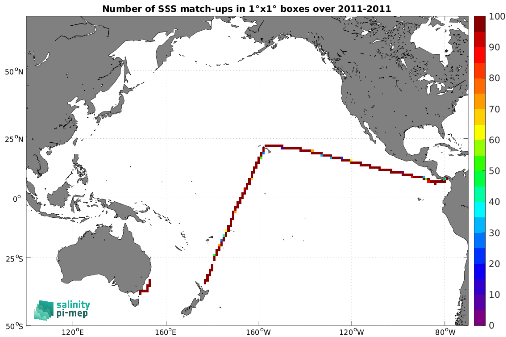
Figure 4: Number of SSS match-ups between TSG (CSIC-UTM) SSS and the SMOS SSS L4 v1 - Monthly (CMEMS-CNR) SSS product for the Pacific Ocean Pi-MEP region over 1^\circ \times 1^\circ boxes and for the full satellite product period.
