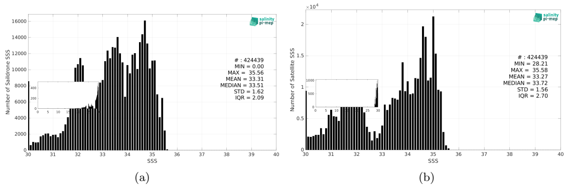
Figure 3: Histograms of SSS from Saildrone (a) and SMOS SSS L4 v1 - Monthly (CMEMS-CNR) (b) considering all match-up pairs per bins of 0.1 over the Pacific Ocean Pi-MEP region and for the full satellite product period.
