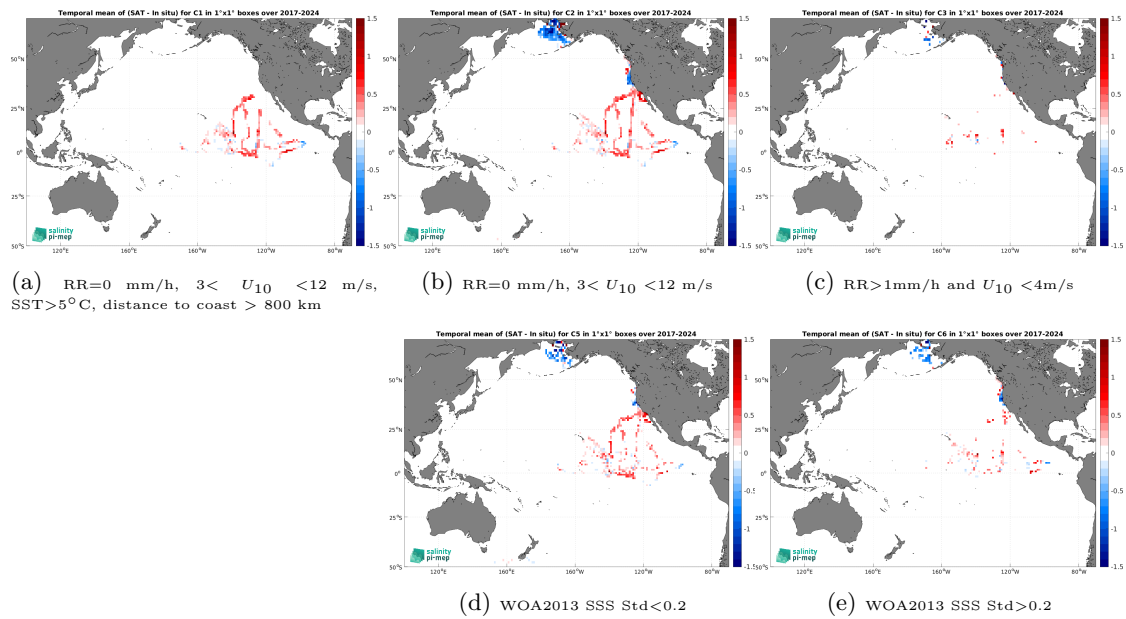
Figure 14: Temporal mean gridded over spatial boxes of size 1^\circ \times 1^\circ of \Delta SSS (SMOS SSS L4 v1 - Monthly (CMEMS-CNR) - Saifdrone) for 5 different subdatasets corresponding to:RR=0 mm/h, 3 < U_{10} < 12 m/s, SST >5^\circ C, distance to coast > 800 km (a), RR=0 mm/h, 3 < U_{10} < 12 m/s (b), RR >1 mm/h and U_{10} < 4 m/s (c), WOA2013 SSS Std <0.2 (d), WOA2013 SSS Std >0.2 (e).
