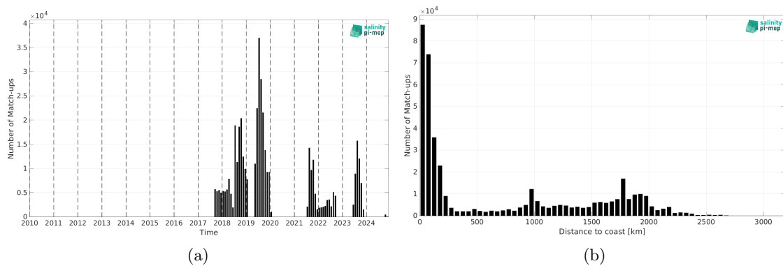
Figure 2: Number of match-ups between Saildrone and SMOS SSS L4 v1 - Monthly (CMEMS-CNR) SSS as a function of time (a) and as function of the distance to coast (b) over the Pacific Ocean Pi-MEP region and for the full satellite product period.
