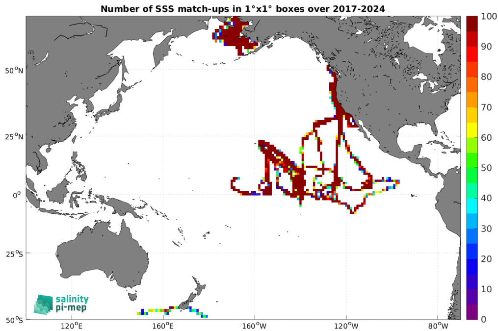
Figure 5: Number of SSS match-ups between Saildrone SSS and the SMOS SSS L4 v1 - Monthly (CMEMS-CNR) SSS product for the Pacific Ocean Pi-MEP region over 1^\circ \times 1^\circ boxes and for the full satellite product period.
