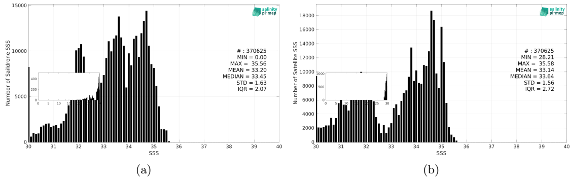
Figure 3: Histograms of SSS from Saildrone (a) and SMOS SSS L4 v1 - Monthly (CMEMS-CNR) (b) considering all match-up pairs per bins of 0.1 over the Pacific Ocean Pi-MEP region and for the full satellite product period.
