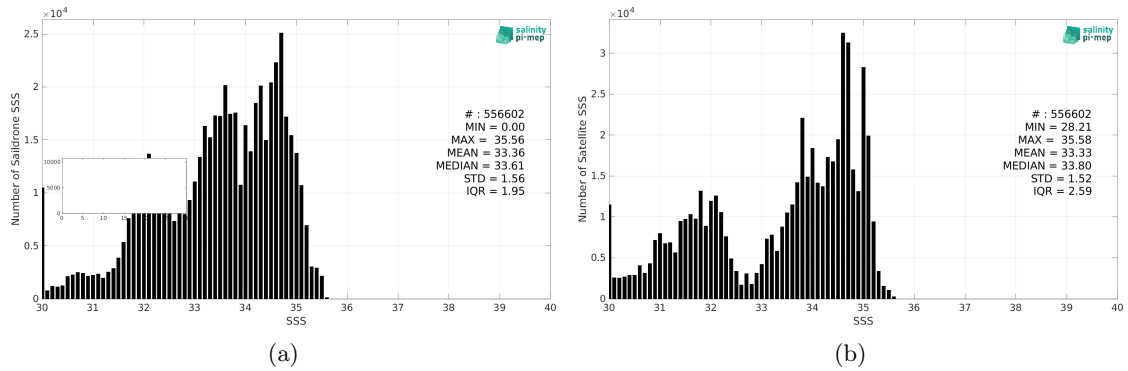
Figure 2: Histograms of SSS from Saildrone (a) and SMOS SSS L4 v1 - Monthly (CMEMS-CNR) (b) considering all match-up pairs per bins of 0.1 over the Pacific Ocean Pi-MEP region and for the full satellite product period.
