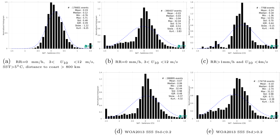
Figure 13: Normalized histogram of \Delta SSS (SMOS SSS L4 v1 - Monthly (CMEMS-CNR) - Saildrone) for 5 different subdatasets corresponding to: RR=0 mm/h, 3 < U_{10} < 12 m/s, SST > 5°C, distance to coast > 800 km (a), RR=0 mm/h, 3 < U_{10} < 12 m/s (b), RR > 1mm/h and U_{10} < 4 m/s (c), WOA2013 SSS Std < 0.2 (d), WOA2013 SSS Std > 0.2 (e).
