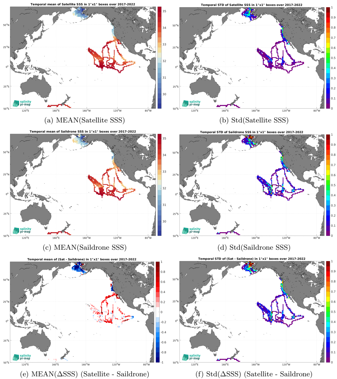
Figure 6: Temporal mean (left) and Std (right) of SSS from SMOS SSS L4 v1 - Monthly (CMEMS-CNR) (top), Saildrone (middle), and of \Delta SSS (Satellite - Saildrone). Only match-up pairs are used to generate these maps.
