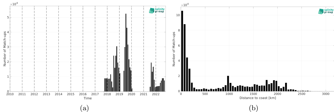
Figure 1: Number of match-ups between Saildrone and SMOS SSS L4 v1 - Monthly (CMEMS-CNR) SSS as a function of time (a) and as function of the distance to coast (b) over the Pacific Ocean Pi-MEP region and for the full satellite product period.
