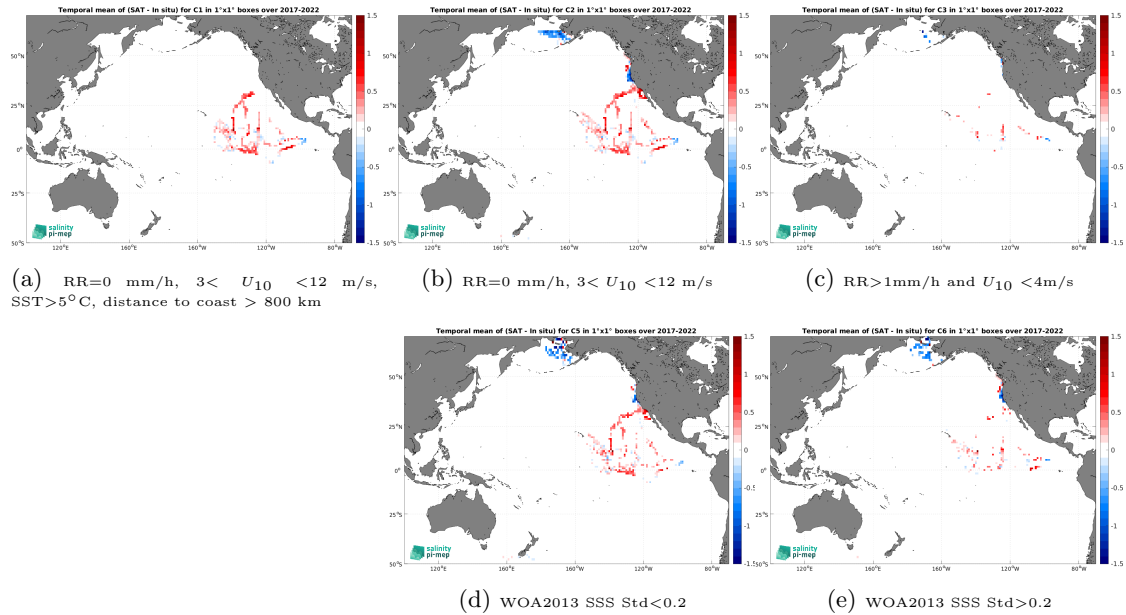
Figure 12: Temporal mean gridded over spatial boxes of size 1^\circ \times 1^\circ of \Delta SSS (SMOS SSS L4 v1 - Monthly (CMEMS-CNR) - Saifdrone) for 5 different subdatasets corresponding to:RR=0 mm/h, 3 < U_{10} < 12 m/s, SST >5^\circ\text{C} , distance to coast > 800 km (a), RR=0 mm/h, 3 < U_{10} < 12 m/s (b), RR >1 mm/h and U_{10} < 4 m/s (c), WOA2013 SSS Std <0.2 (d), WOA2013 SSS Std >0.2 (e).
