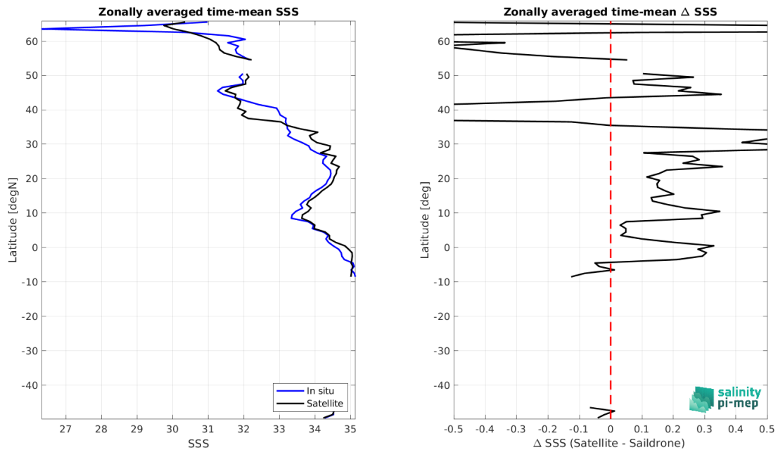
Figure 8: Left panel: Zonal mean SSS from SMOS SSS L4 v1 - Monthly (CMEMS-CNR) satellite product (black) and from Saildrone (blue). Right panel: Zonal mean of \Delta SSS (Satellite - Saildrone) for all the collected Pi-MEP match-up pairs estimated over the full satellite product period.
