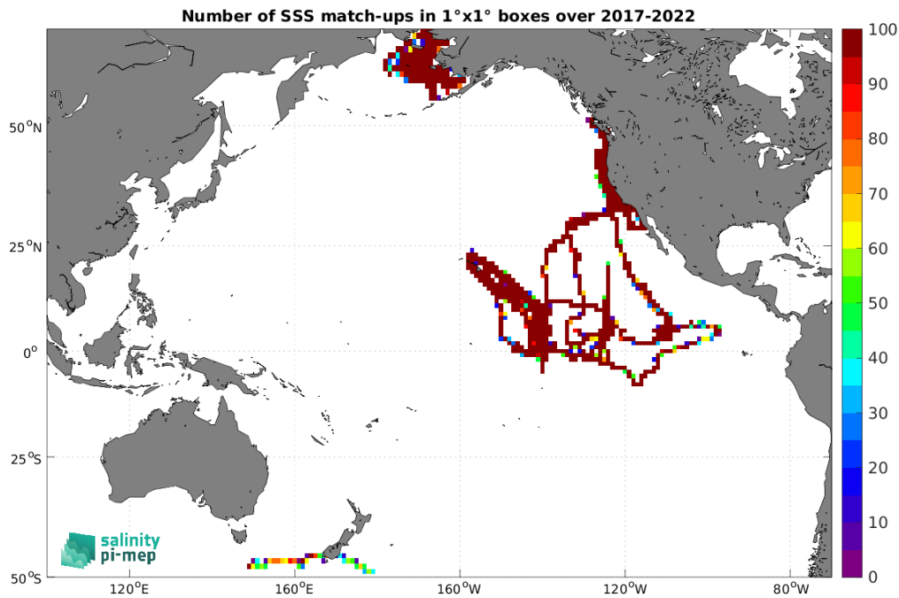
Figure 4: Number of SSS match-ups between Saildrone SSS and the SMOS SSS L4 v1 - Monthly (CMEMS-CNR) SSS product for the Pacific Ocean Pi-MEP region over 1^\circ \times 1^\circ boxes and for the full satellite product period.
