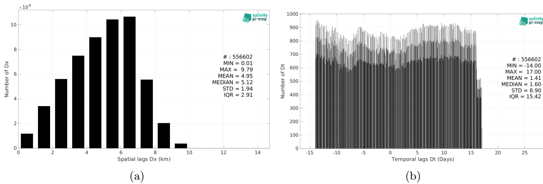
Figure 5: Histograms of the spatial (a) and temporal (b) lags between the location/time of the Saildrone measurement and the date of the corresponding SMOS SSS L4 v1 - Monthly (CMEMS-CNR) SSS pixel.
