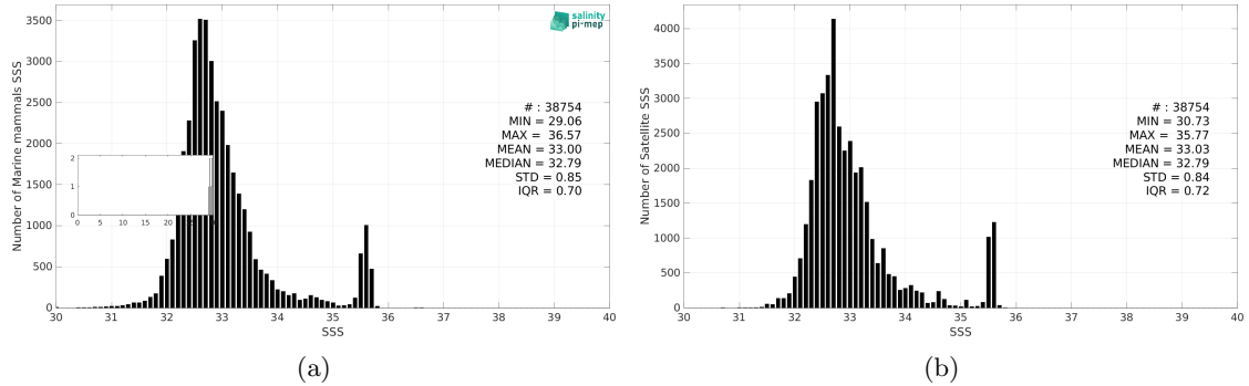
Figure 3: Histograms of SSS from Marine mammals (a) and SMOS SSS L4 v1 - Monthly (CMEMS-CNR) (b) considering all match-up pairs per bins of 0.1 over the Pacific Ocean Pi-MEP region and for the full satellite product period.
