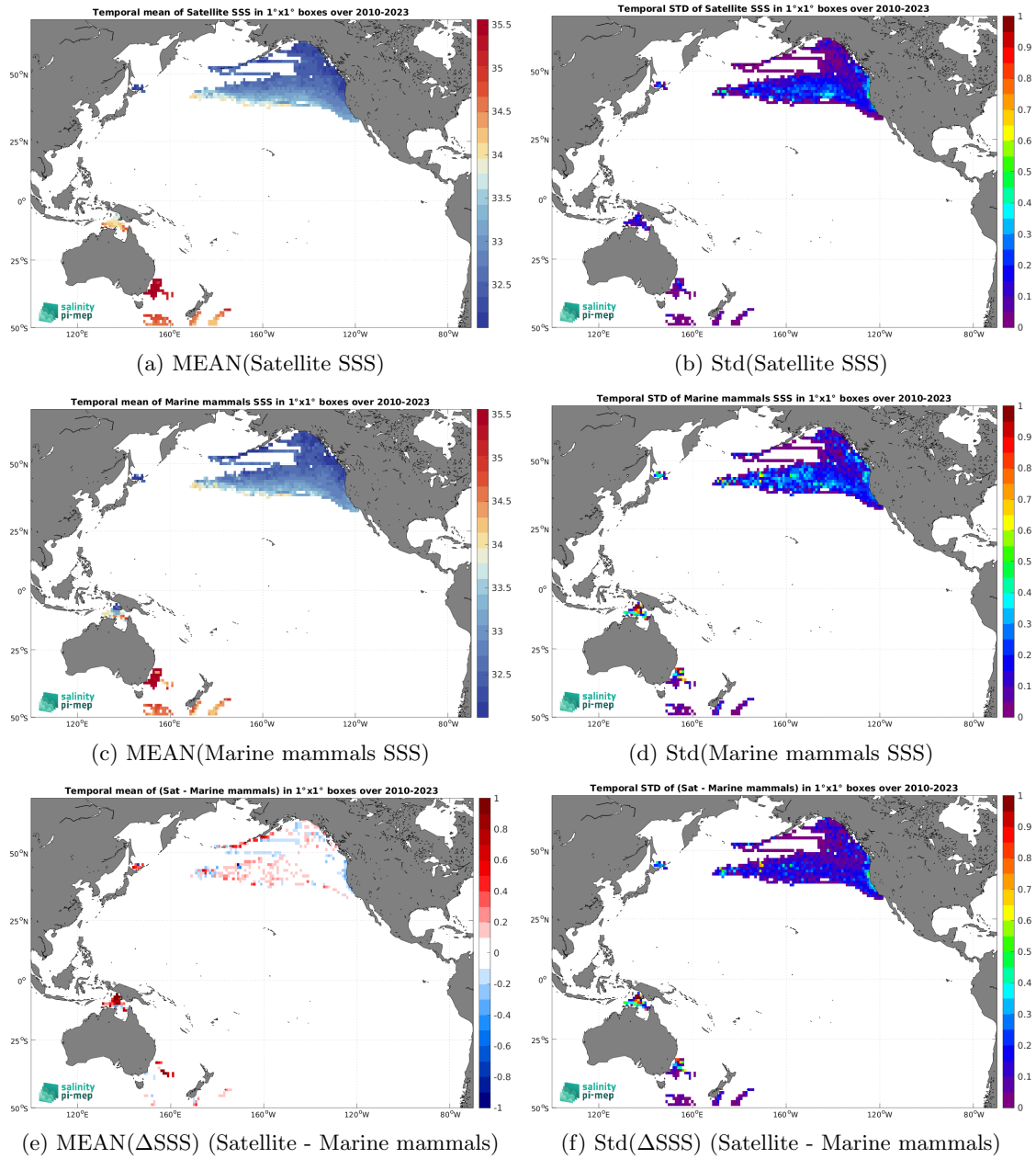
Figure 7: Temporal mean (left) and Std (right) of SSS from SMOS SSS L4 v1 - Monthly (CMEMS-CNR) (top), Marine mammals (middle), and of \Delta SSS (Satellite - Marine mammals). Only match-up pairs are used to generate these maps.
