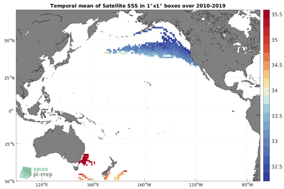
(a) MEAN(Satellite SSS)
