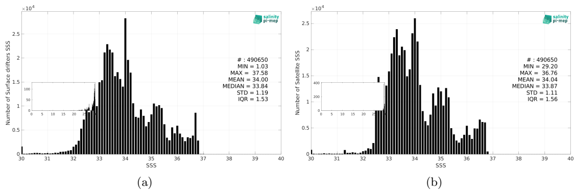
Figure 3: Histograms of SSS from Surface drifters (a) and SMOS SSS L4 v1 - Monthly (CMEMS-CNR) (b) considering all match-up pairs per bins of 0.1 over the Pacific Ocean Pi-MEP region and for the full satellite product period.
