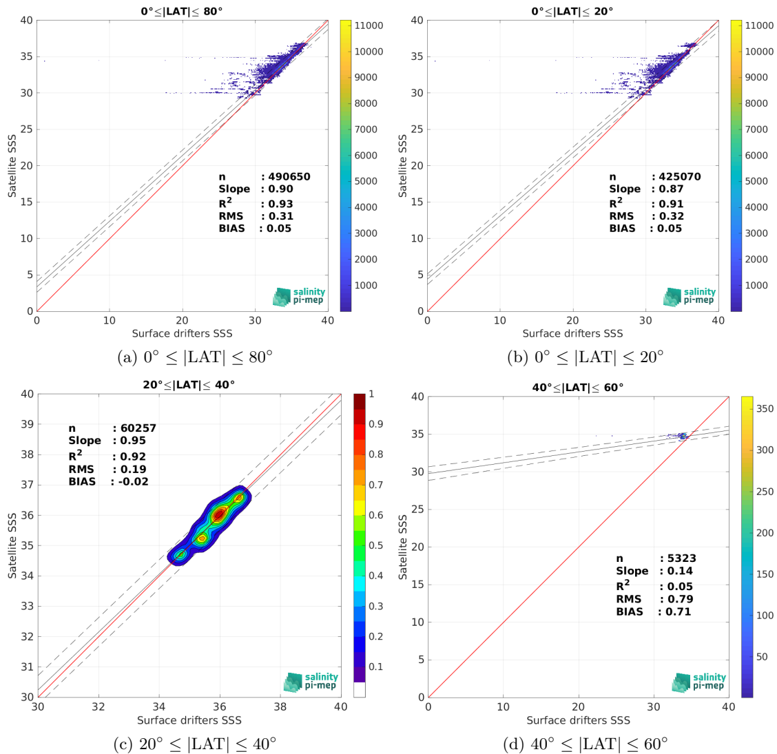
Figure 9: Contour maps of the concentration of SMOS SSS L4 v1 - Monthly (CMEMS-CNR) SSS (y-axis) versus Surface drifters SSS (x-axis) at match-up pairs for different latitude bands. For each plot, the red line shows x=y . The black thin and dashed lines indicate a linear fit through the data cloud and the \pm 95\% confidence levels, respectively. The number match-up pairs n , the slope and R^2 coefficient of the linear fit, the root mean square (RMS) and the mean bias between satellite and in situ data are indicated for each latitude band in each plot.
