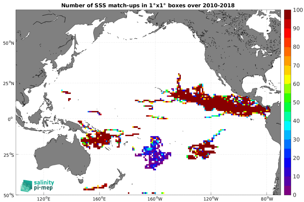
Figure 4: Number of SSS match-ups between Surface drifters SSS and the SMOS SSS L4 v1 - Monthly (CMEMS-CNR) SSS product for the Pacific Ocean Pi-MEP region over 1^\circ \times 1^\circ boxes and for the full satellite product period.
