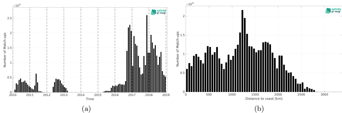
Figure 2: Number of match-ups between Surface drifters and SMOS SSS L4 v1 - Monthly (CMEMS-CNR) SSS as a function of time (a) and as function of the distance to coast (b) over the Pacific Ocean Pi-MEP region and for the full satellite product period.
