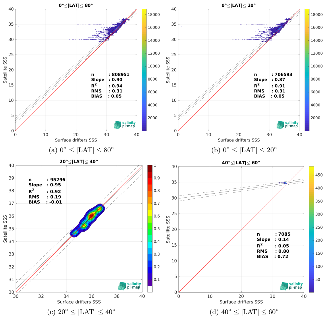
Figure 8: Contour maps of the concentration of SMOS SSS L4 v1 - Monthly (CMEMS-CNR) SSS (y-axis) versus Surface drifters SSS (x-axis) at match-up pairs for different latitude bands. For each plot, the red line shows x=y . The black thin and dashed lines indicate a linear fit through the data cloud and the \pm 95\% confidence levels, respectively. The number match-up pairs n , the slope and R^2 coefficient of the linear fit, the root mean square (RMS) and the mean bias between satellite and in situ data are indicated for each latitude band in each plots.
