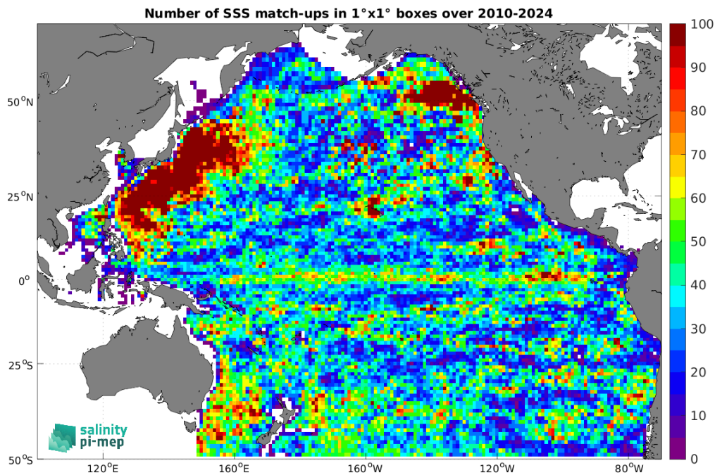
Figure 5: Number of SSS match-ups between Argo SSS and the SMOS SSS L4 v1 - Monthly (CMEMS-CNR) SSS product for the Pacific Ocean Pi-MEP region over 1^\circ \times 1^\circ boxes and for the full satellite product period.
