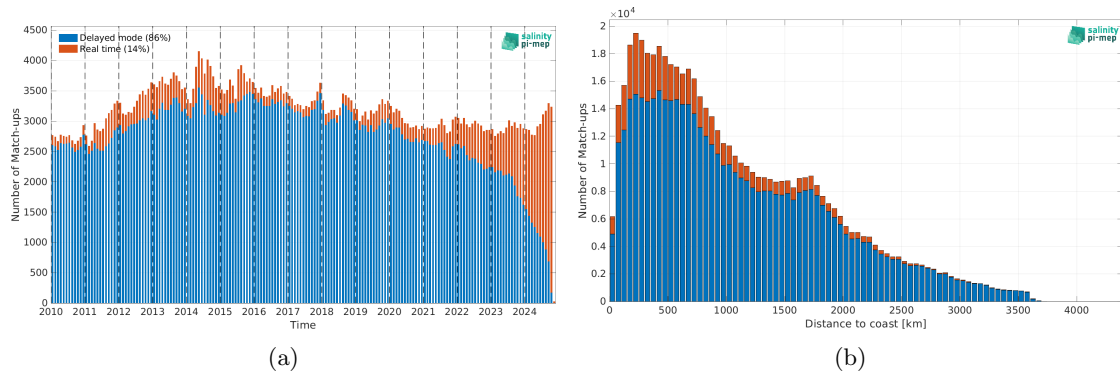
Figure 2: Number of match-ups between Argo and SMOS SSS L4 v1 - Monthly (CMEMS-CNR) SSS as a function of time (a) and as function of the distance to coast (b) over the Pacific Ocean Pi-MEP region and for the full satellite product period.
