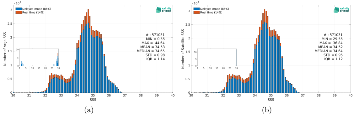
Figure 3: Histograms of SSS from Argo (a) and SMOS SSS L4 v1 - Monthly (CMEMS-CNR) (b) considering all match-up pairs per bins of 0.1 over the Pacific Ocean Pi-MEP region and for the full satellite product period.
