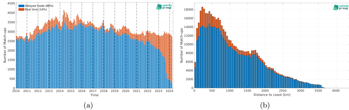
Figure 2: Number of match-ups between Argo and SMOS SSS L4 v1 - Monthly (CMEMS-CNR) SSS as a function of time (a) and as function of the distance to coast (b) over the Pacific Ocean Pi-MEP region and for the full satellite product period.
