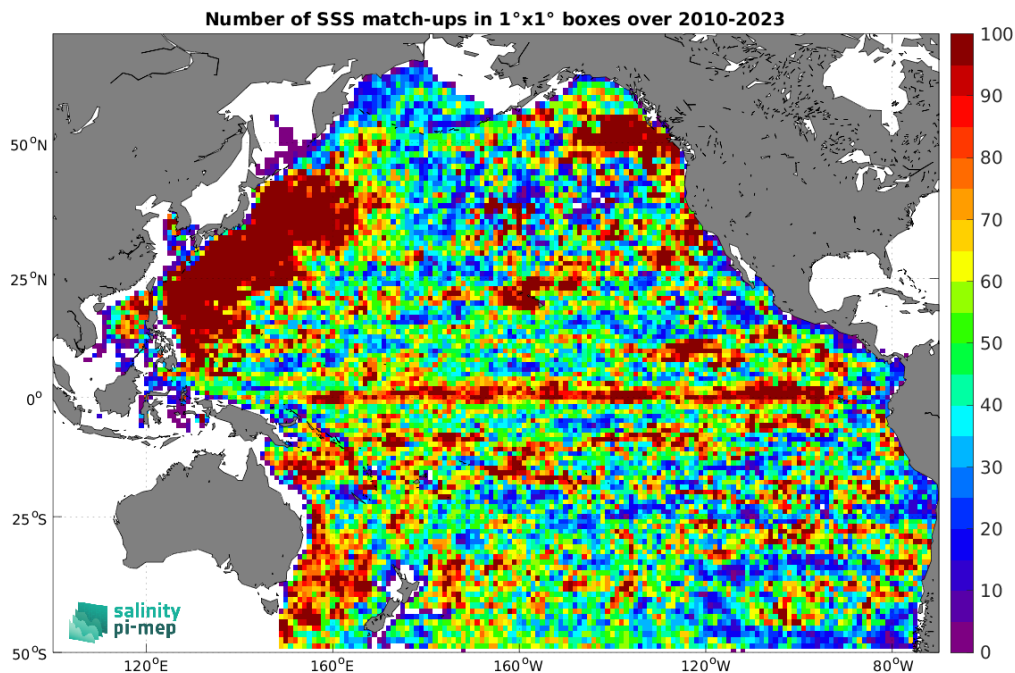
Figure 4: Number of SSS match-ups between Argo SSS and the SMOS SSS L4 v1 - Monthly (CMEMS-CNR) SSS product for the Pacific Ocean Pi-MEP region over 1^{\circ} \times 1^{\circ} boxes and for the full satellite product period.
