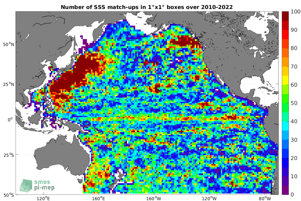
Figure 4: Number of SSS match-ups between Argo SSS and the SMOS SSS L4 v1 - Monthly (CMEMS-CNR) SSS product for the Pacific Ocean Pi-MEP region over 1°×1° boxes and for the full satellite product period.
