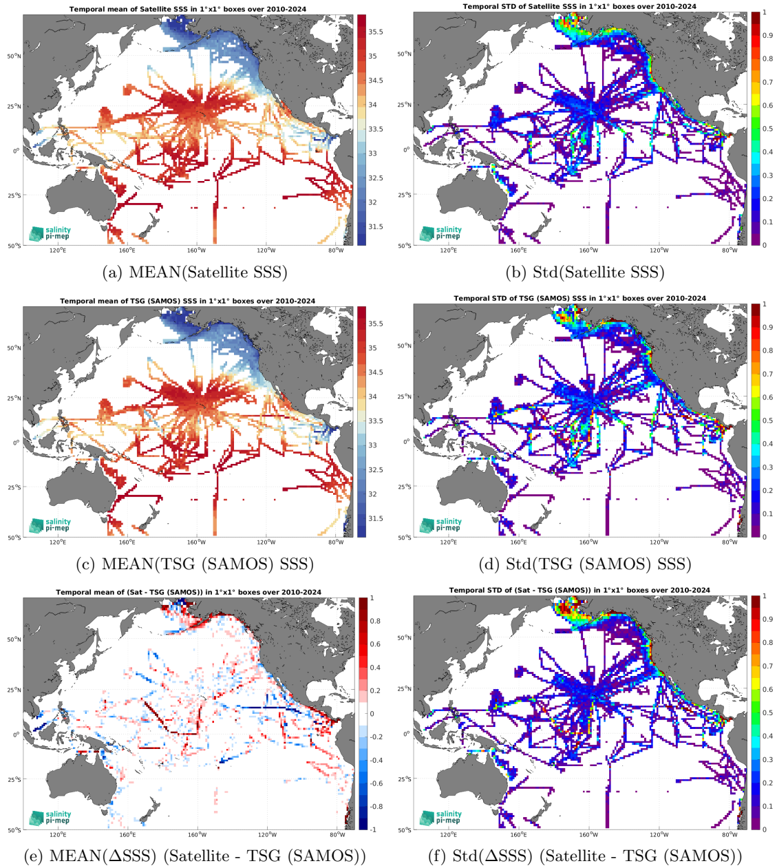
Figure 7: Temporal mean (left) and Std (right) of SSS from SMOS SSS L4 v1 - Daily (CMEMS-CNR) (top), TSG (SAMOS) (middle), and of \Delta SSS (Satellite - TSG (SAMOS)). Only match-up pairs are used to generate these maps.
