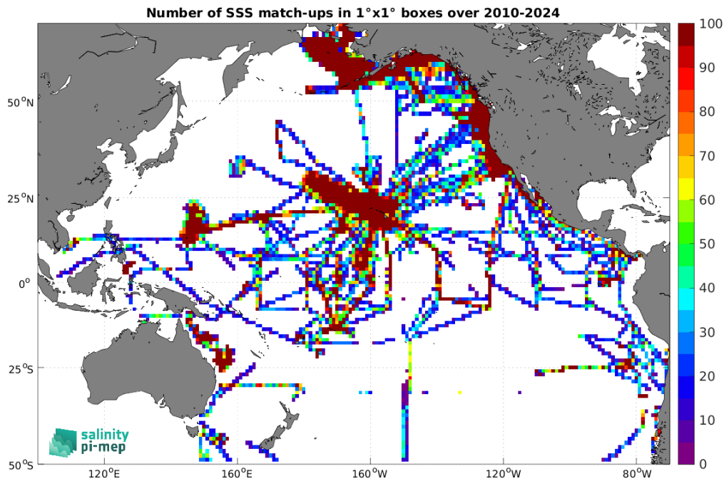
Figure 5: Number of SSS match-ups between TSG (SAMOS) SSS and the SMOS SSS L4 v1 - Daily (CMEMS-CNR) SSS product for the Pacific Ocean Pi-MEP region over 1^\circ \times 1^\circ boxes and for the full satellite product period.
