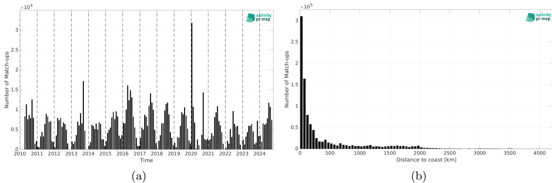
Figure 2: Number of match-ups between TSG (SAMOS) and SMOS SSS L4 v1 - Daily (CMEMS-CNR) SSS as a function of time (a) and as function of the distance to coast (b) over the Pacific Ocean Pi-MEP region and for the full satellite product period.
