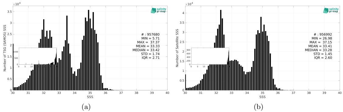
Figure 3: Histograms of SSS from TSG (SAMOS) (a) and SMOS SSS L4 v1 - Daily (CMEMS-CNR) (b) considering all match-up pairs per bins of 0.1 over the Pacific Ocean Pi-MEP region and for the full satellite product period.
