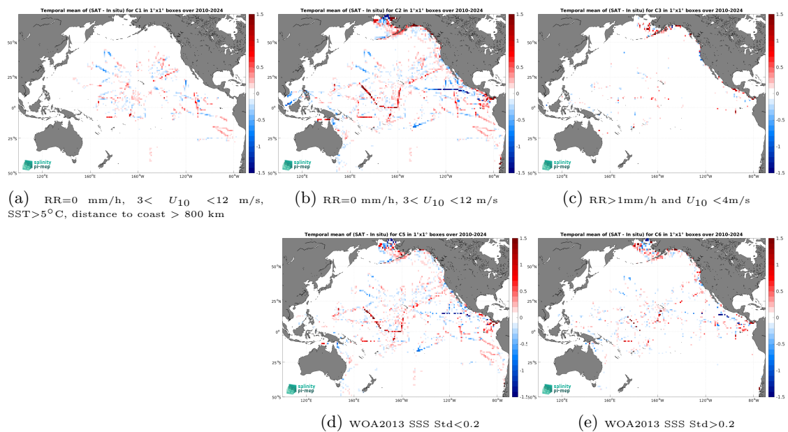
Figure 14: Temporal mean gridded over spatial boxes of size 1^\circ \times 1^\circ of \Delta\text{SSS} (SMOS SSS L4 v1 - Daily (CMEMS-CNR) - TSG (SAMOS)) for 5 different subdatasets corresponding to:RR=0 mm/h, 3 < U_{10} < 12 m/s, SST > 5^\circ\text{C} , distance to coast > 800 km (a), RR=0 mm/h, 3 < U_{10} < 12 m/s (b), RR > 1 mm/h and U_{10} < 4 m/s (c), WOA2013 SSS Std < 0.2 (d), WOA2013 SSS Std > 0.2 (e).
