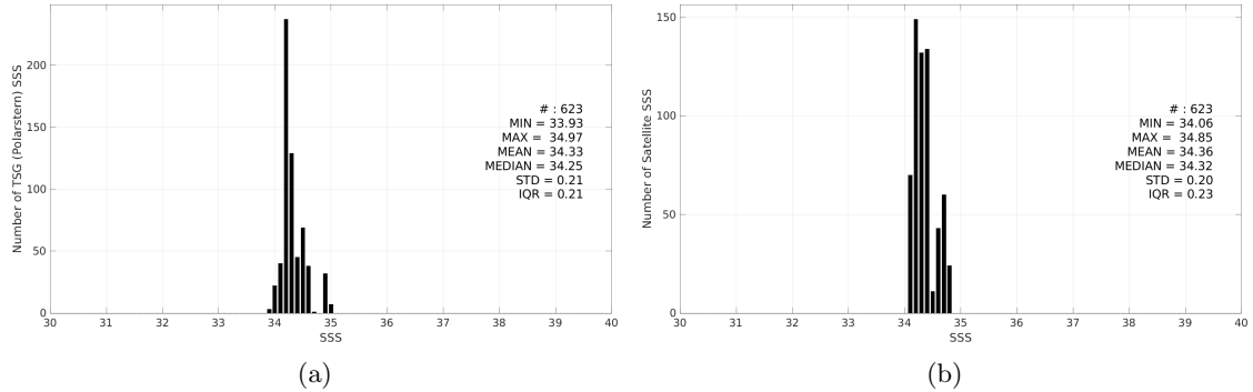
Figure 3: Histograms of SSS from TSG (Polarstern) (a) and SMOS SSS L4 v1 - Daily (CMEMS-CNR) (b) considering all match-up pairs per bins of 0.1 over the Pacific Ocean Pi-MEP region and for the full satellite product period.
