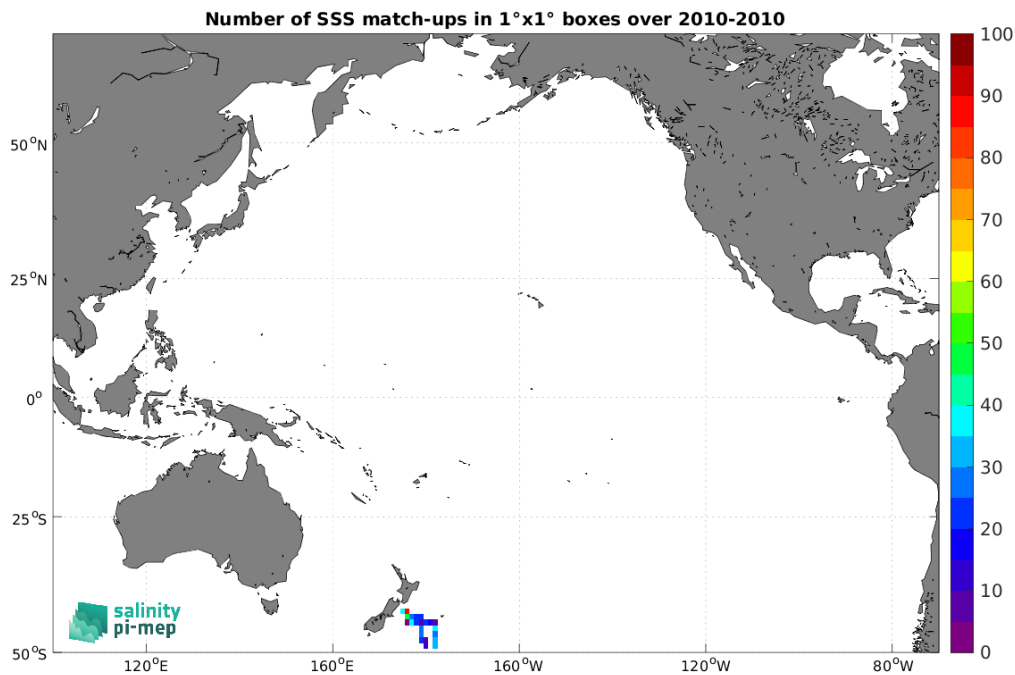
Figure 5: Number of SSS match-ups between TSG (Polarstern) SSS and the SMOS SSS L4 v1 - Daily (CMEMS-CNR) SSS product for the Pacific Ocean Pi-MEP region over 1^\circ \times 1^\circ boxes and for the full satellite product period.
